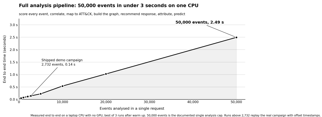
Figure 3. Measured end to end analysis time against input size.
