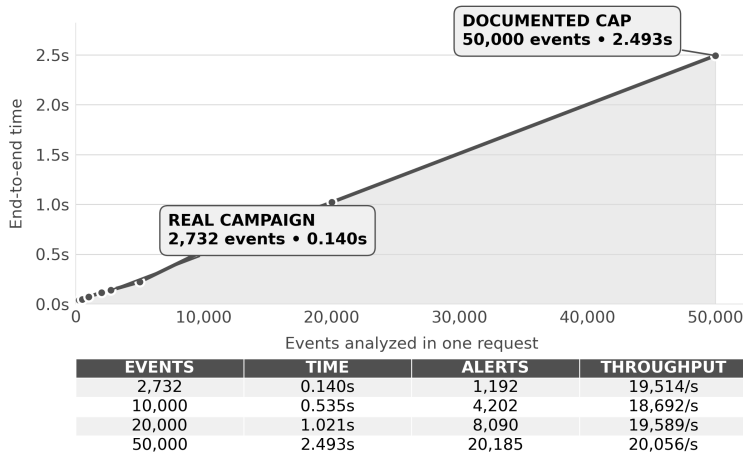
Figure 3. Measured end to end analysis time against input size, with the measurement table and verification notes.
