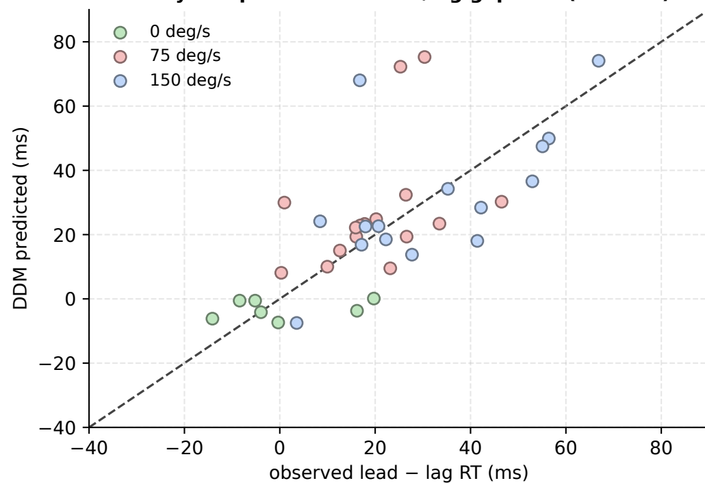
D ...yet it predicts the lead/lag gap well ( r = 0.72 )
