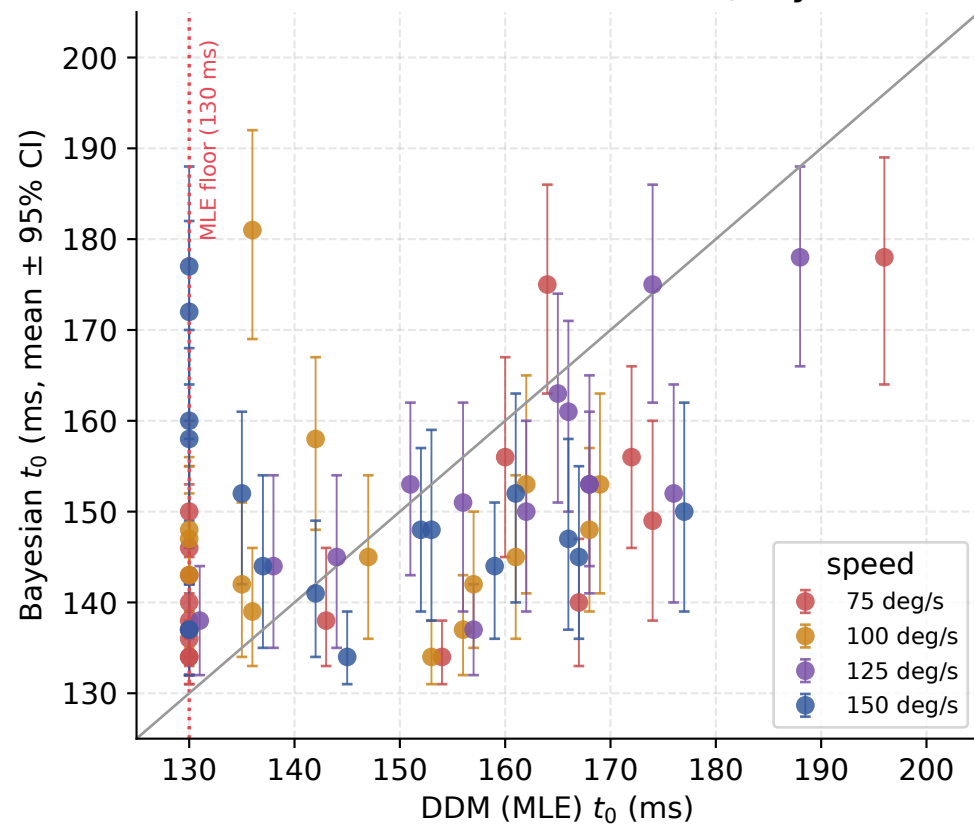
A. HRT t_0 : Method A (MLE) vs Method B (Bayesian) (cells at the 130 ms floor: MLE 19/64, Bayesian 0/64)
