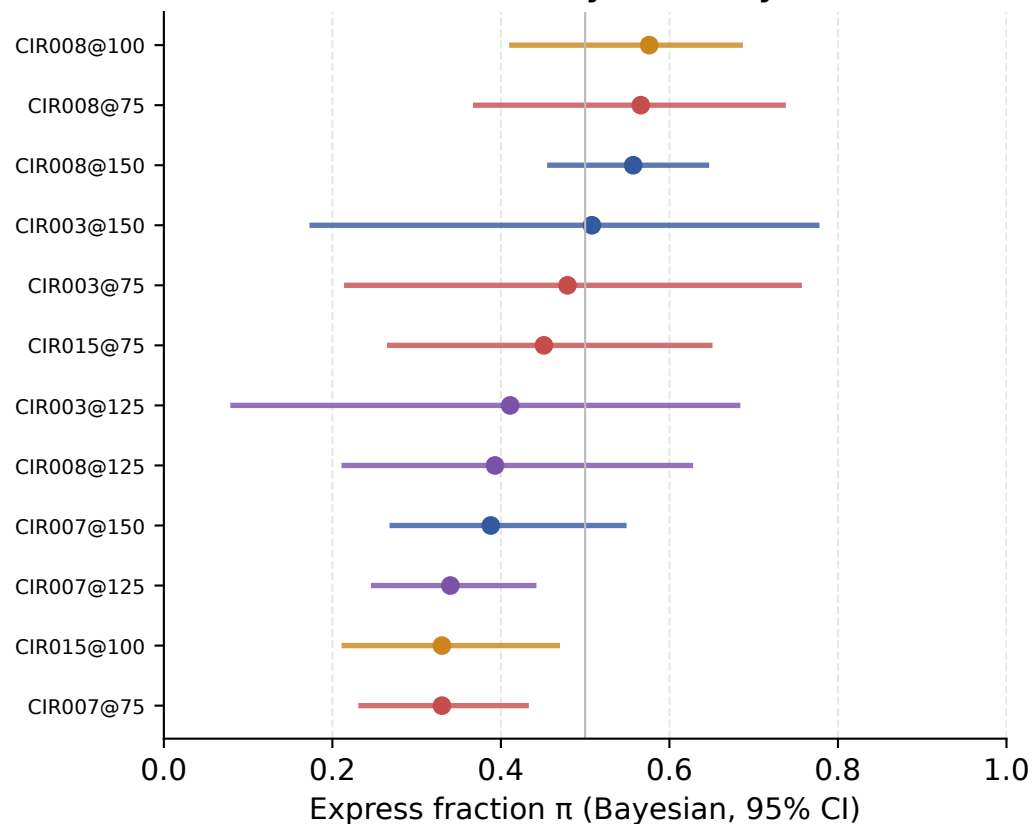
B. SRT express fraction & uncertainty (wide bars = bimodality not firmly identified)
