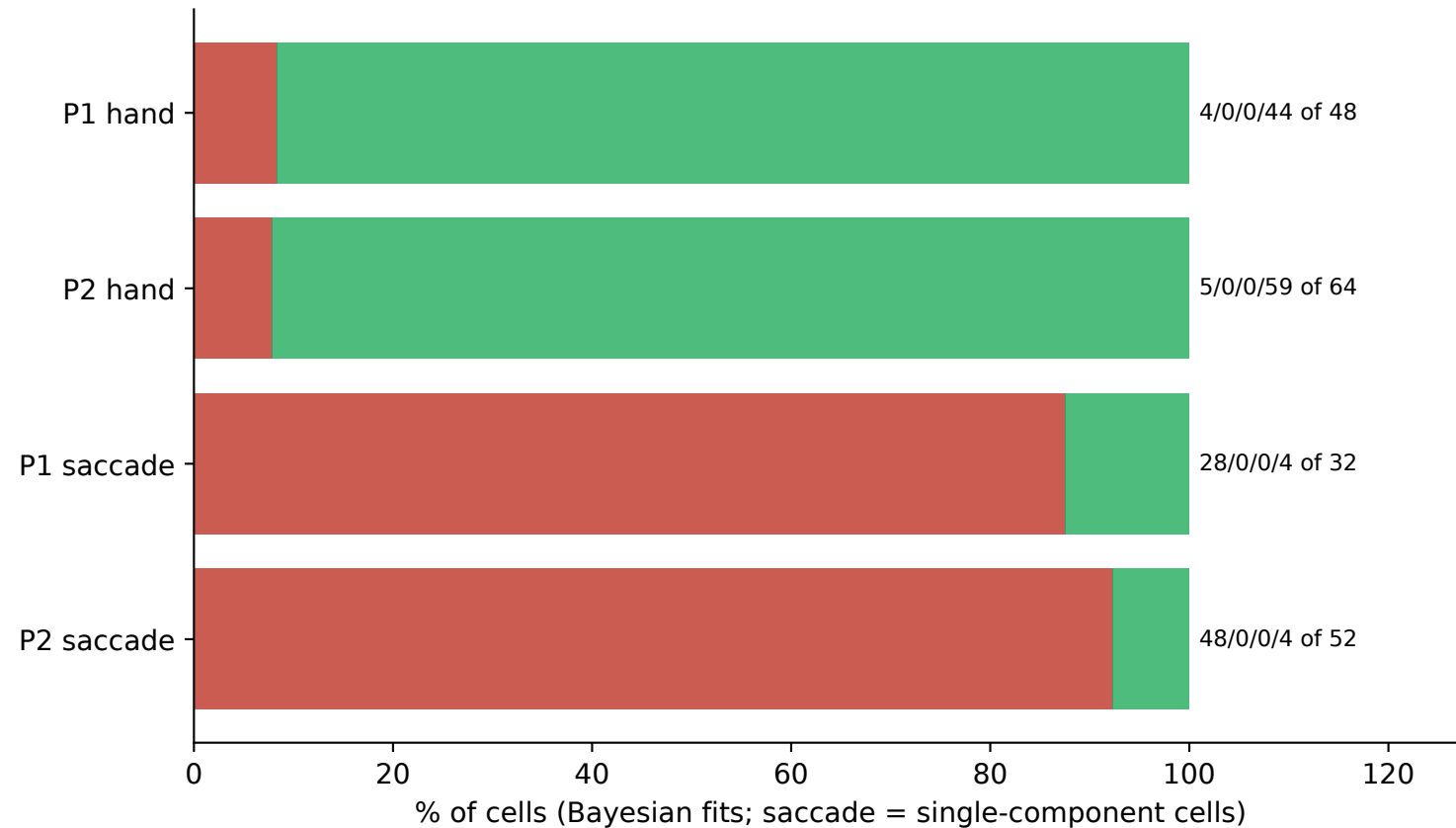
C. Does each cell's 95% interval for t_0 run into a bound? red = floor, orange = the cell's fastest RT, purple = both, green = neither
