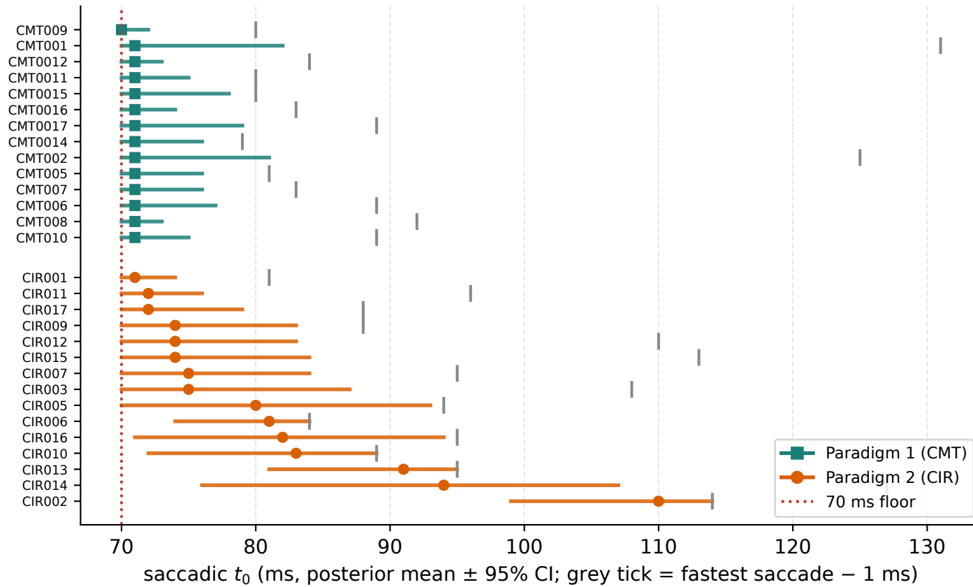
A. Participant-level saccadic t_0 vs its two bounds P1: 14/14 at floor, 0 at ceiling | P2: 10/15 at floor, 6 at ceiling
