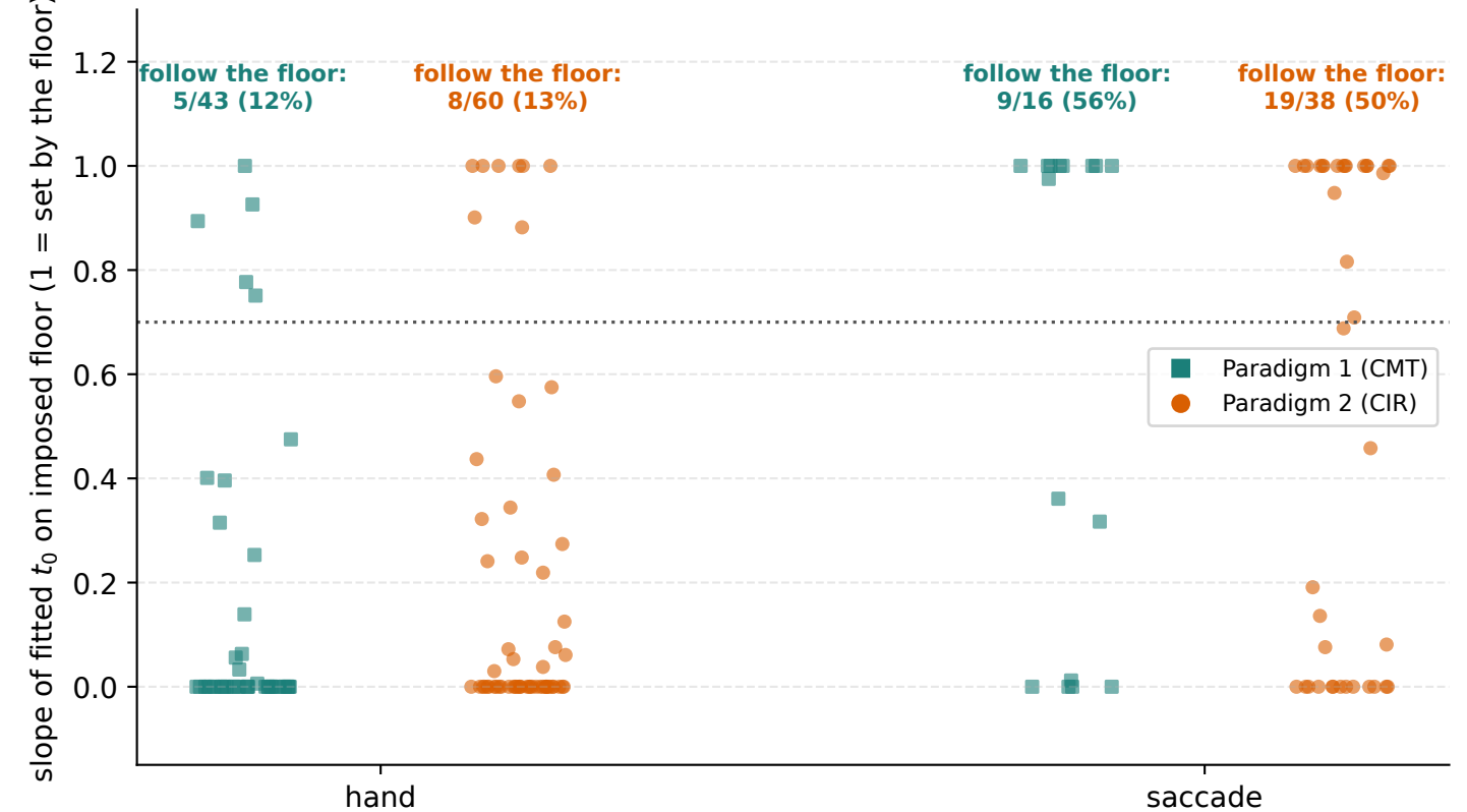
D. Floor sweep, same code on both paradigms: share of fits whose t_0 follows the floor (dots = fits; above the dotted line = follows the floor; fits stuck at their fastest RT excluded)
