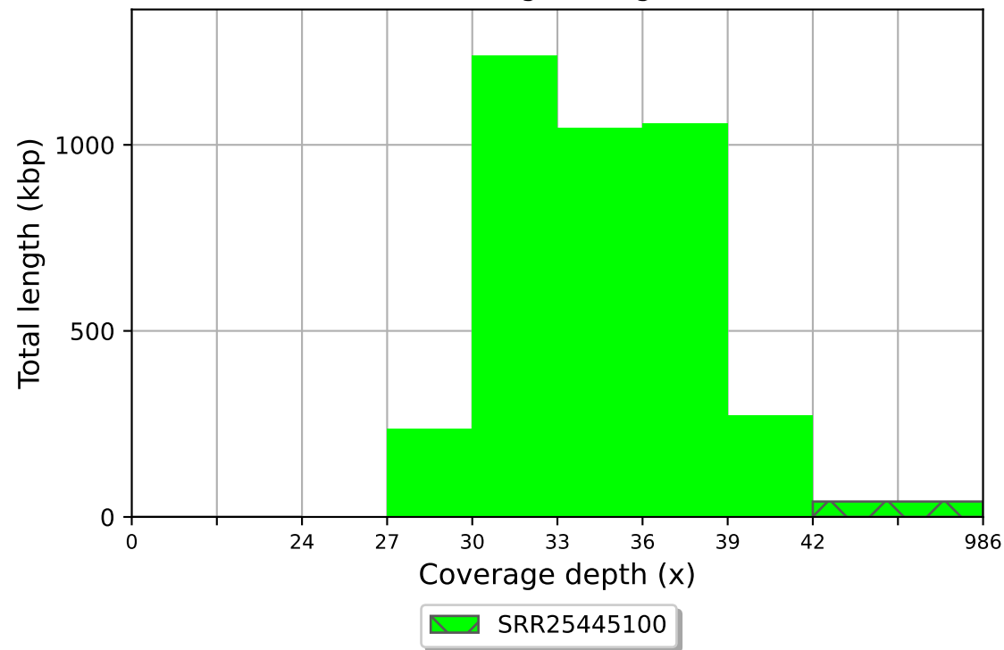
SRR25445100 coverage histogram (bin size: 3x)
