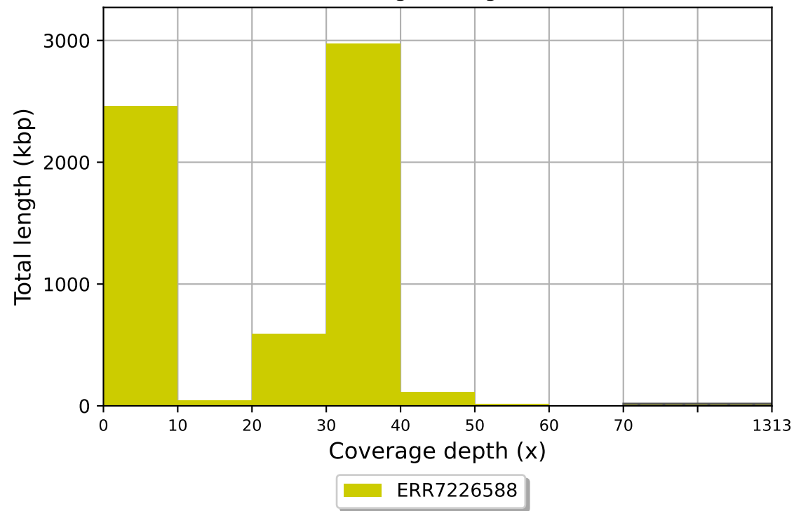
ERR7226588 coverage histogram (bin size: 10x)
