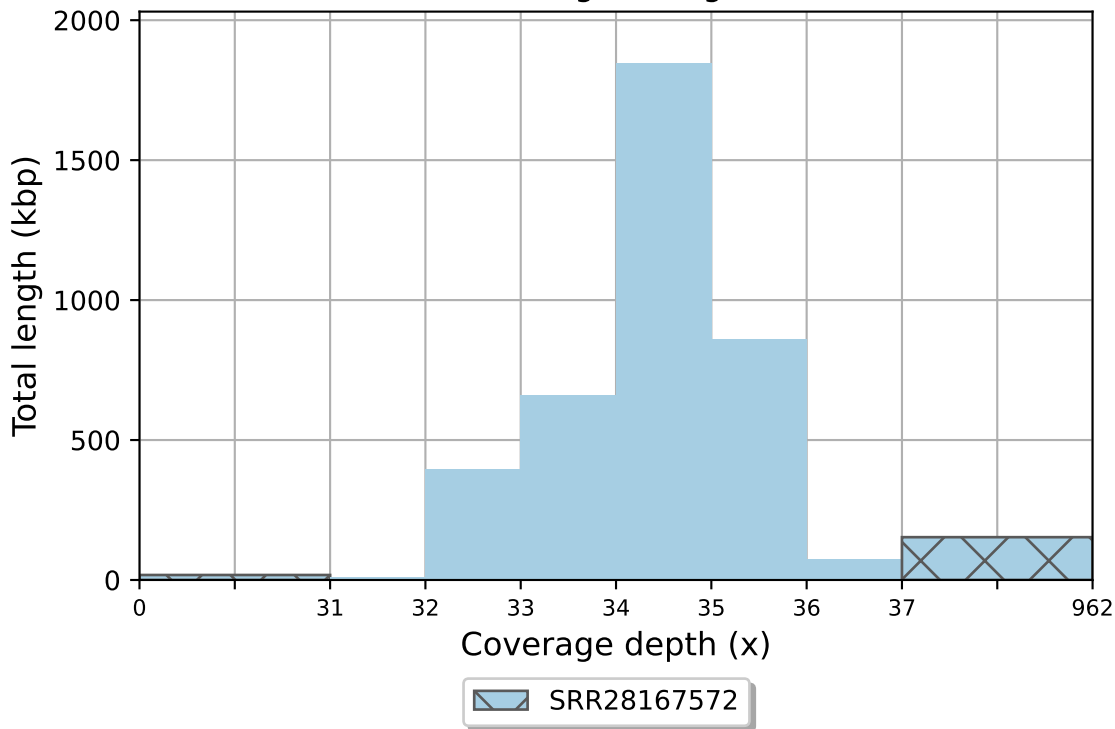
SRR28167572 coverage histogram (bin size: 1x)
