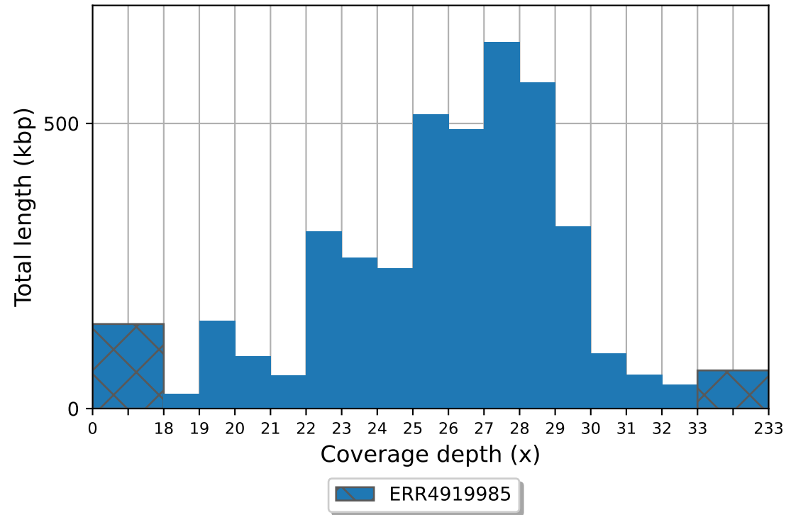
ERR4919985 coverage histogram (bin size: 1x)
