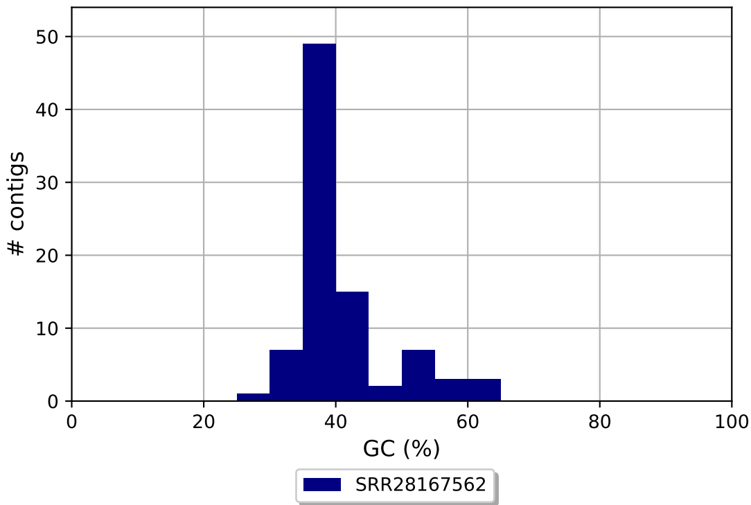
SRR28167562 GC content
