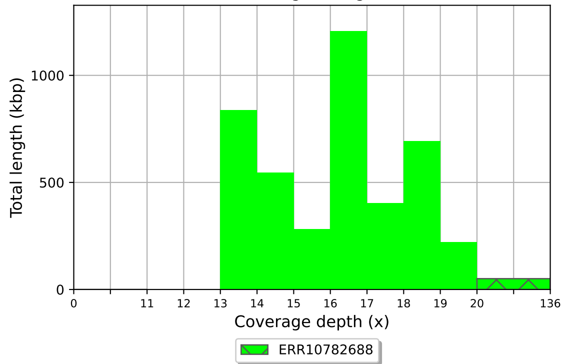
ERR10782688 coverage histogram (bin size: 1x)
