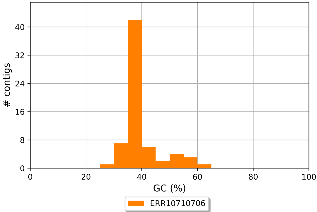
ERR10710706 GC content
