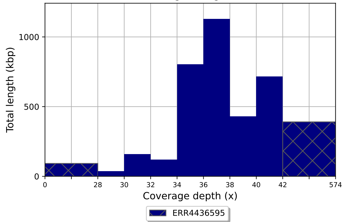
ERR4436595 coverage histogram (bin size: 2x)
