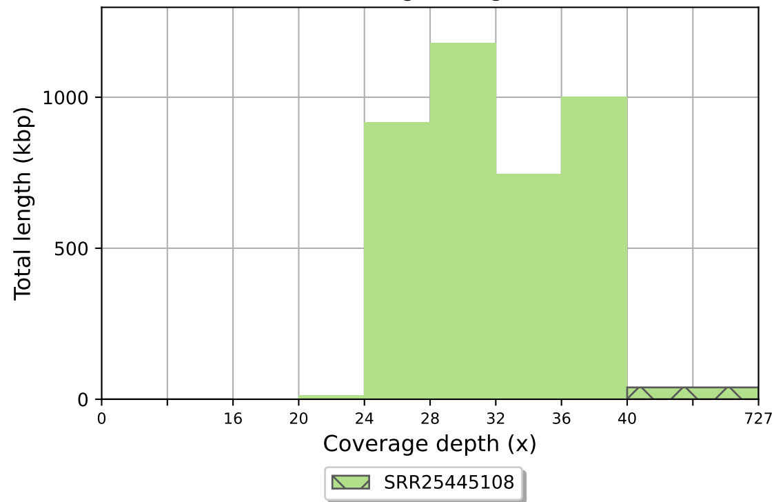
SRR25445108 coverage histogram (bin size: 4x)
