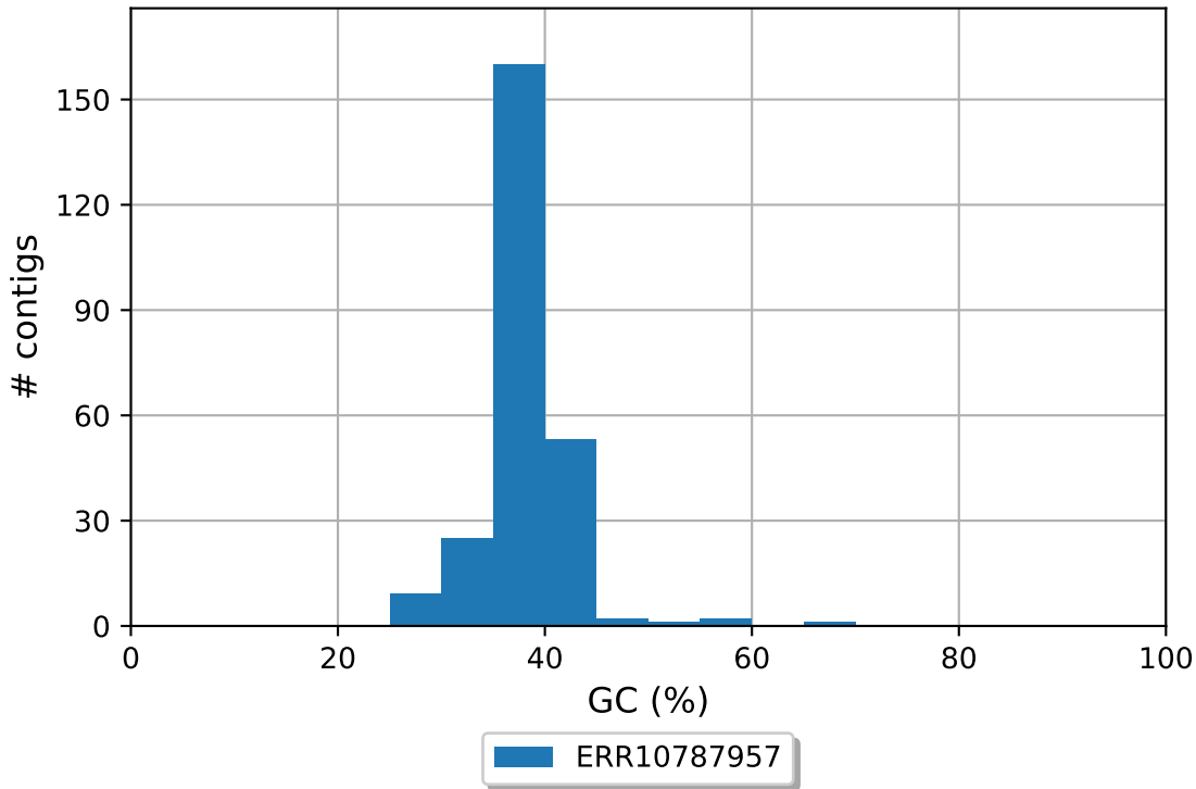
ERR10787957 GC content
