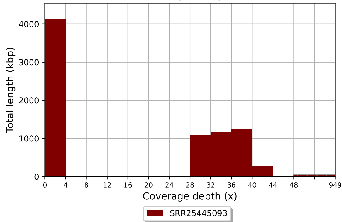
SRR25445093 coverage histogram (bin size: 4x)
