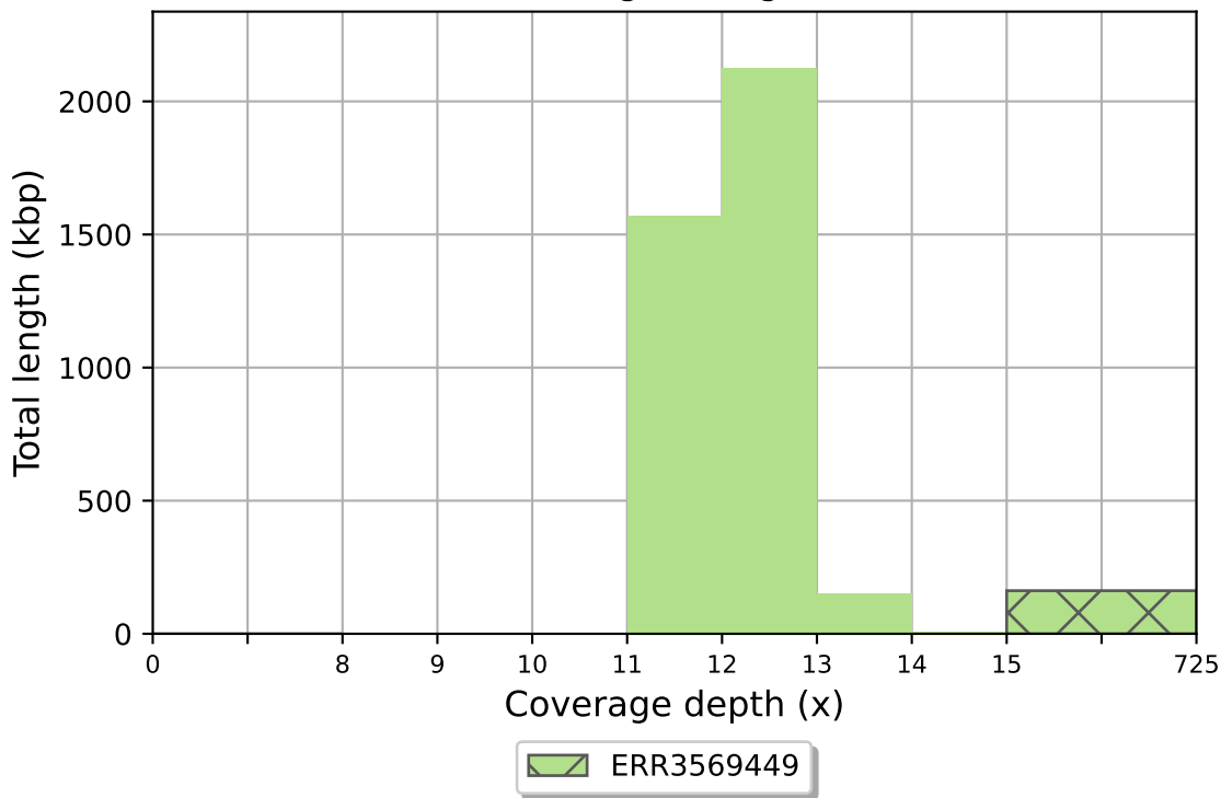
ERR3569449 coverage histogram (bin size: 1x)
