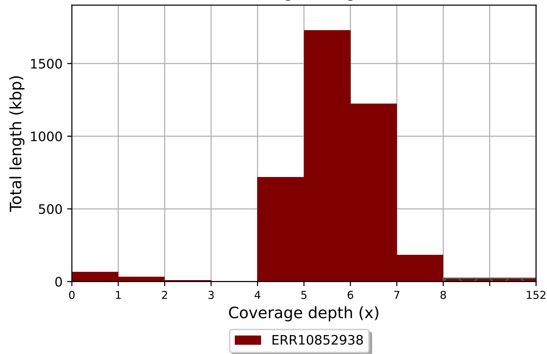
ERR10852938 coverage histogram (bin size: 1x)
