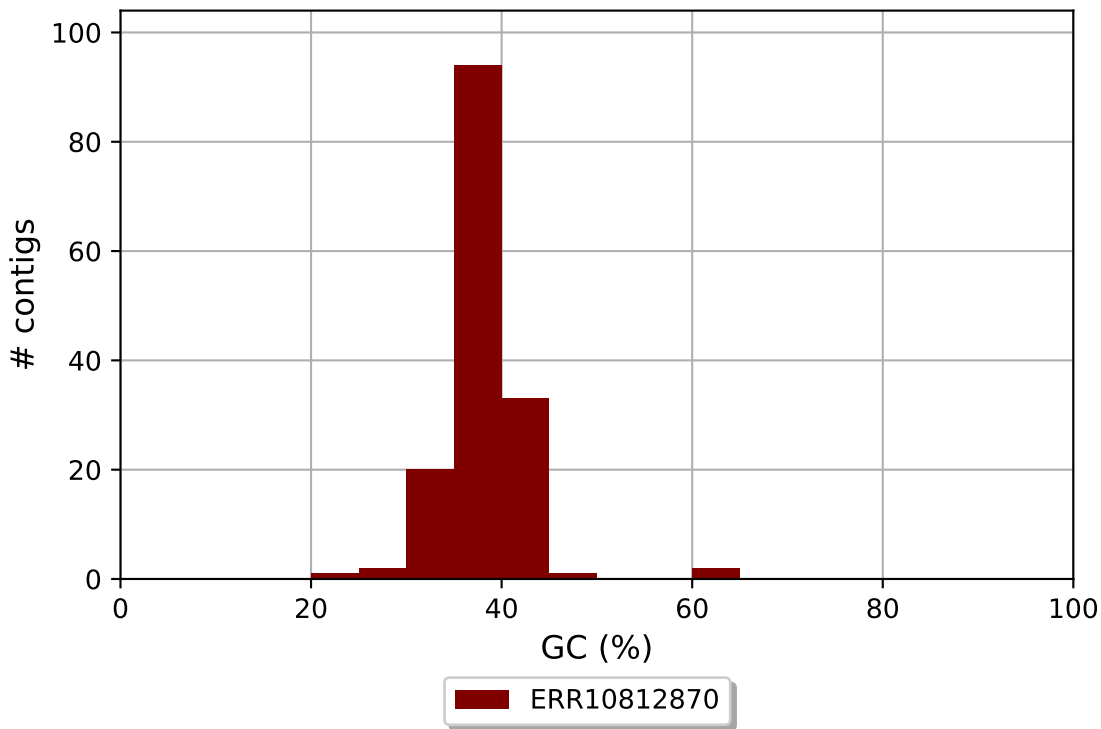
ERR10812870 GC content
