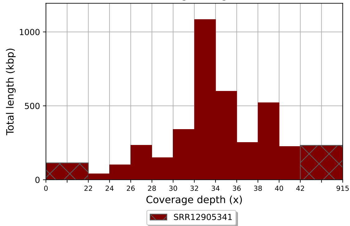
SRR12905341 coverage histogram (bin size: 2x)
