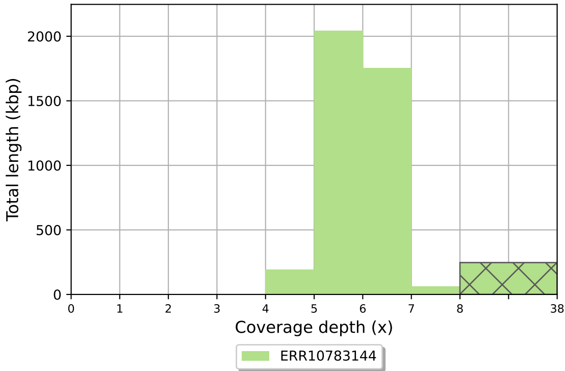
ERR10783144 coverage histogram (bin size: 1x)
