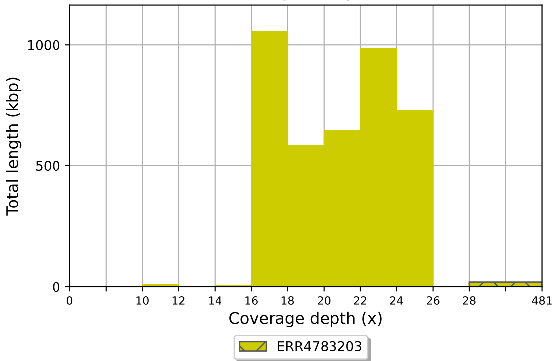
ERR4783203 coverage histogram (bin size: 2x)
