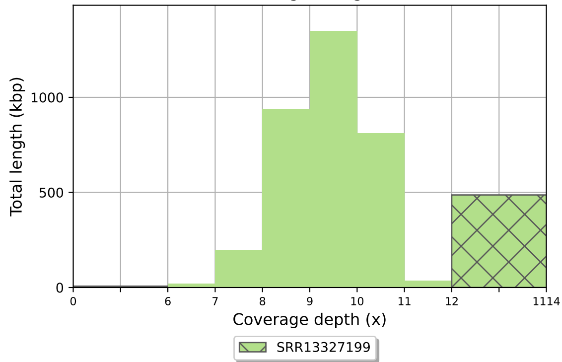
SRR13327199 coverage histogram (bin size: 1x)
