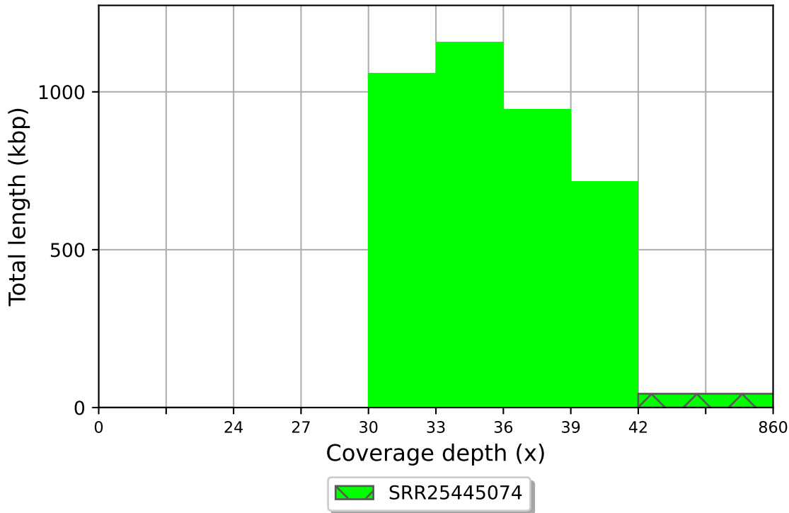
SRR25445074 coverage histogram (bin size: 3x)
