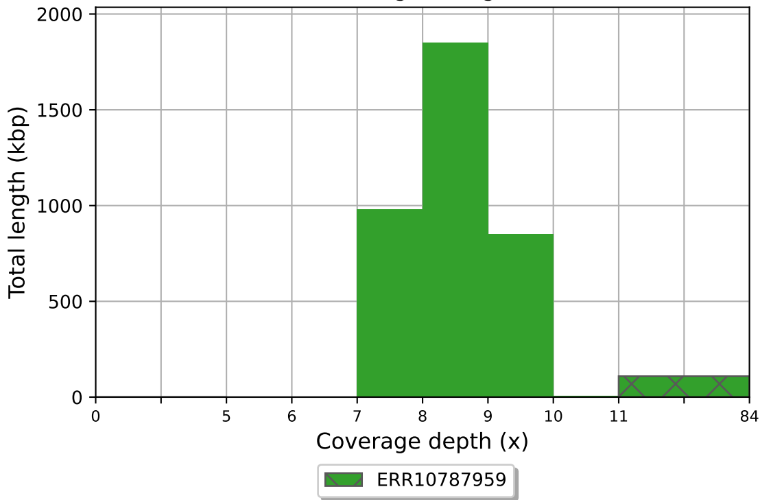
ERR10787959 coverage histogram (bin size: 1x)
