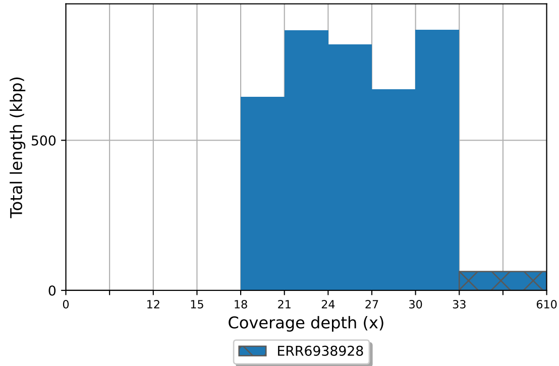
ERR6938928 coverage histogram (bin size: 3x)
