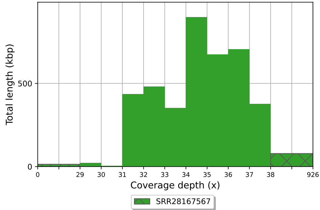
SRR28167567 coverage histogram (bin size: 1x)
