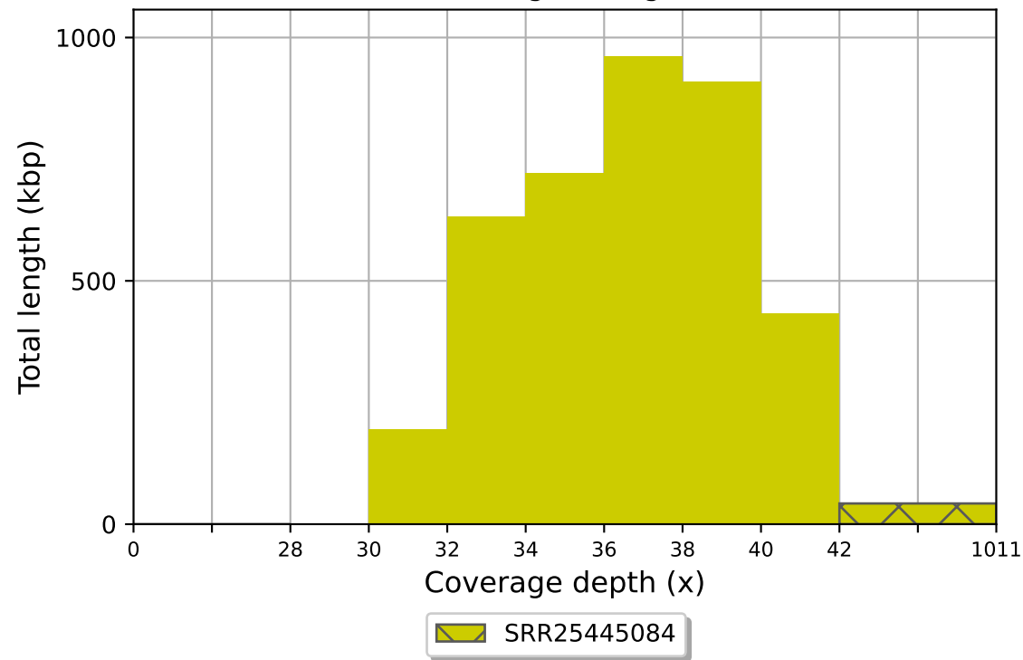
SRR25445084 coverage histogram (bin size: 2x)
