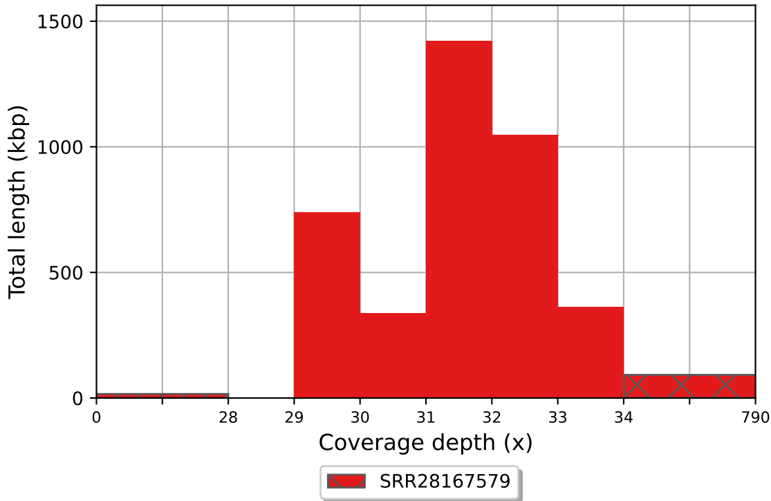
SRR28167579 coverage histogram (bin size: 1x)
