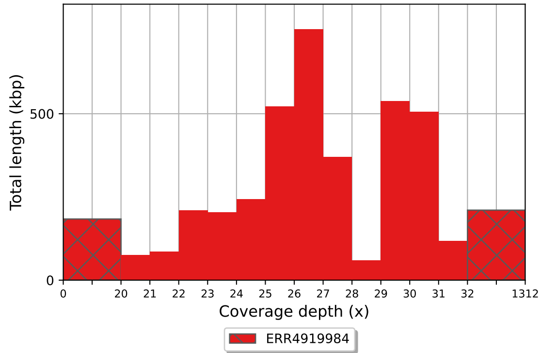
ERR4919984 coverage histogram (bin size: 1x)
