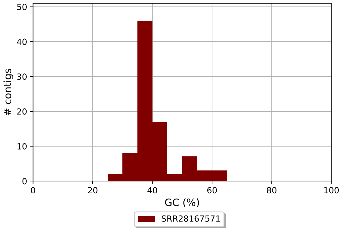
SRR28167571 GC content
