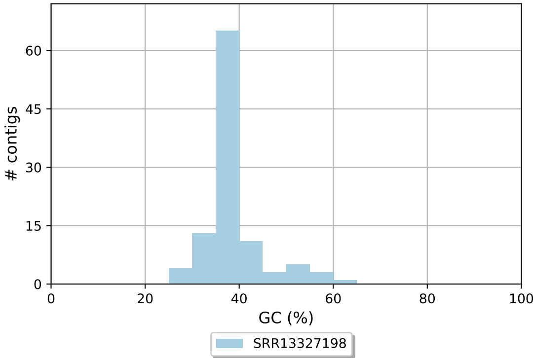
SRR13327198 GC content
