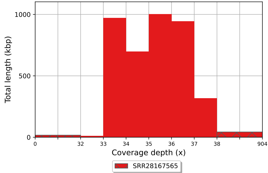
SRR28167565 coverage histogram (bin size: 1x)
