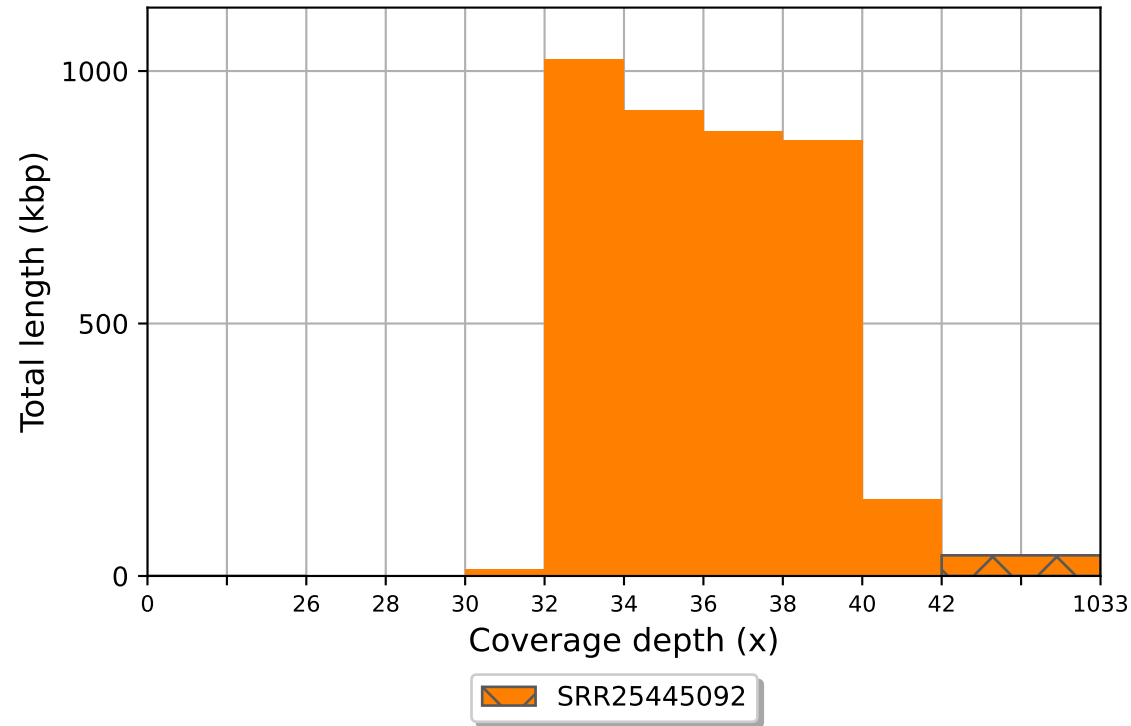
SRR25445092 coverage histogram (bin size: 2x)
