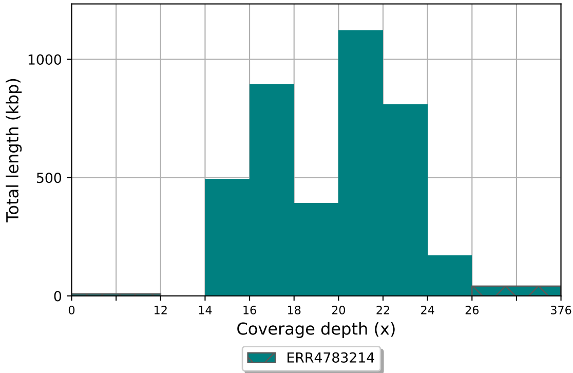
ERR4783214 coverage histogram (bin size: 2x)
