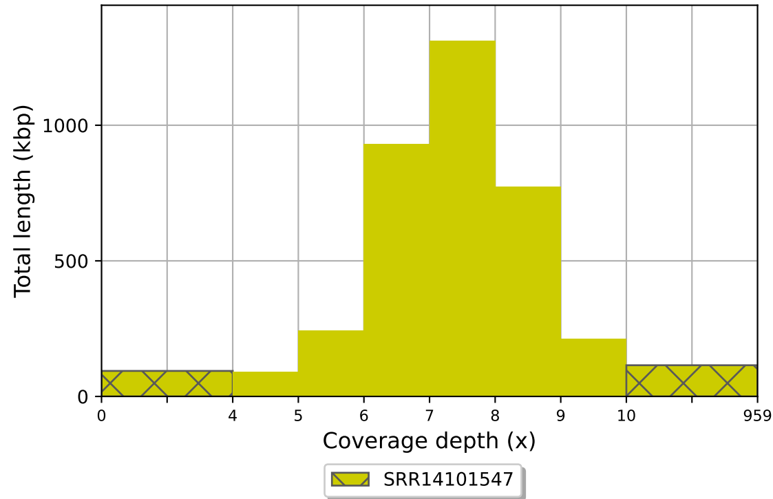
SRR14101547 coverage histogram (bin size: 1x)
