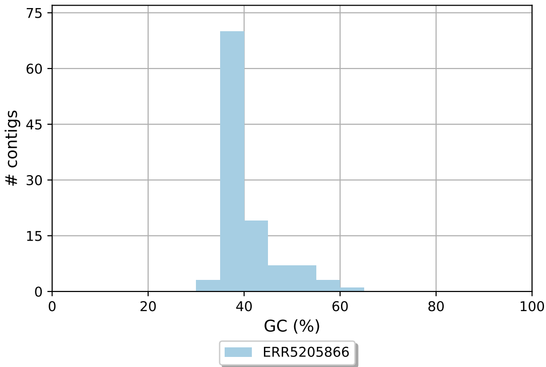
ERR5205866 GC content
