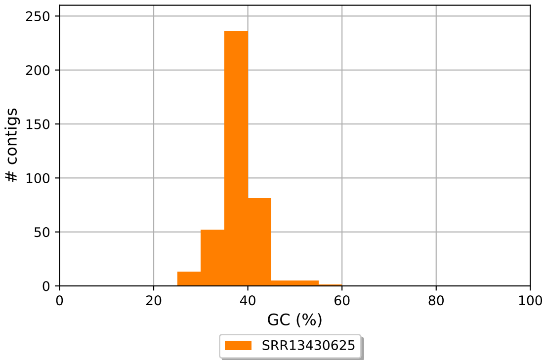
SRR13430625 GC content
