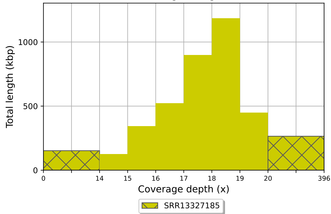
SRR13327185 coverage histogram (bin size: 1x)
