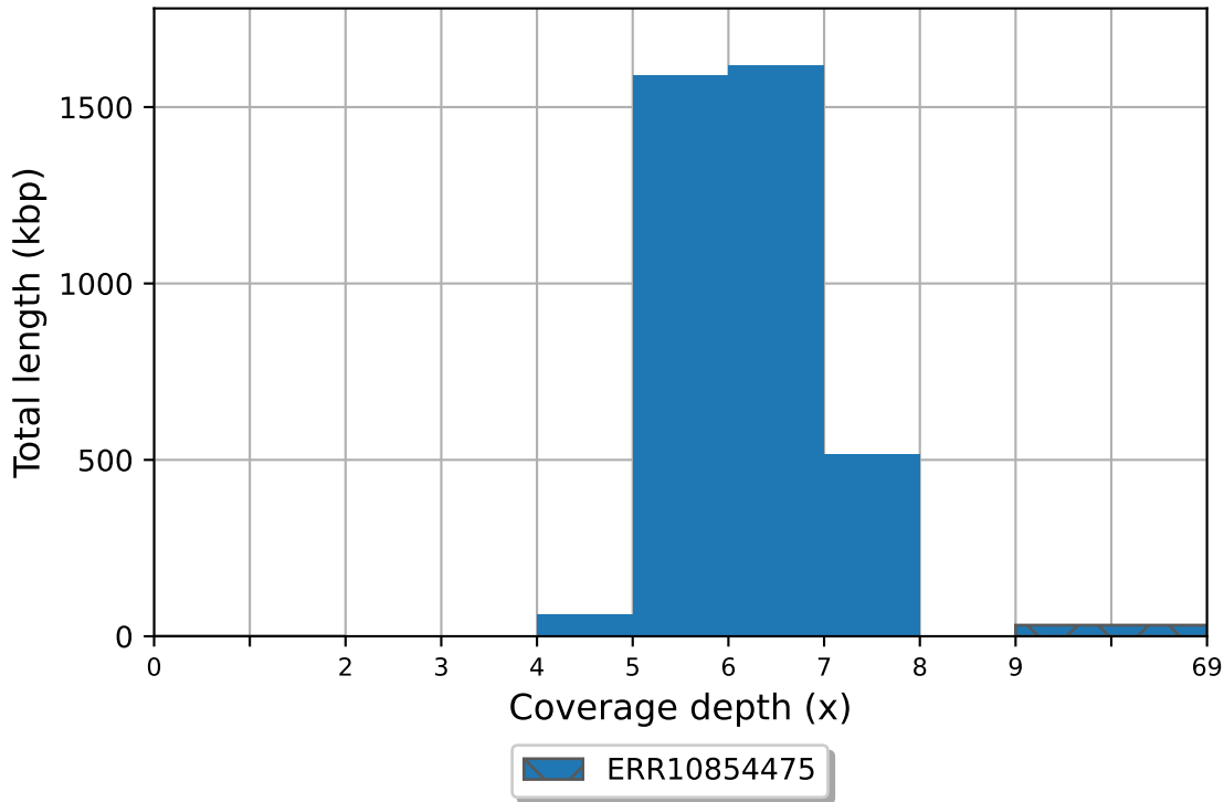
ERR10854475 coverage histogram (bin size: 1x)
