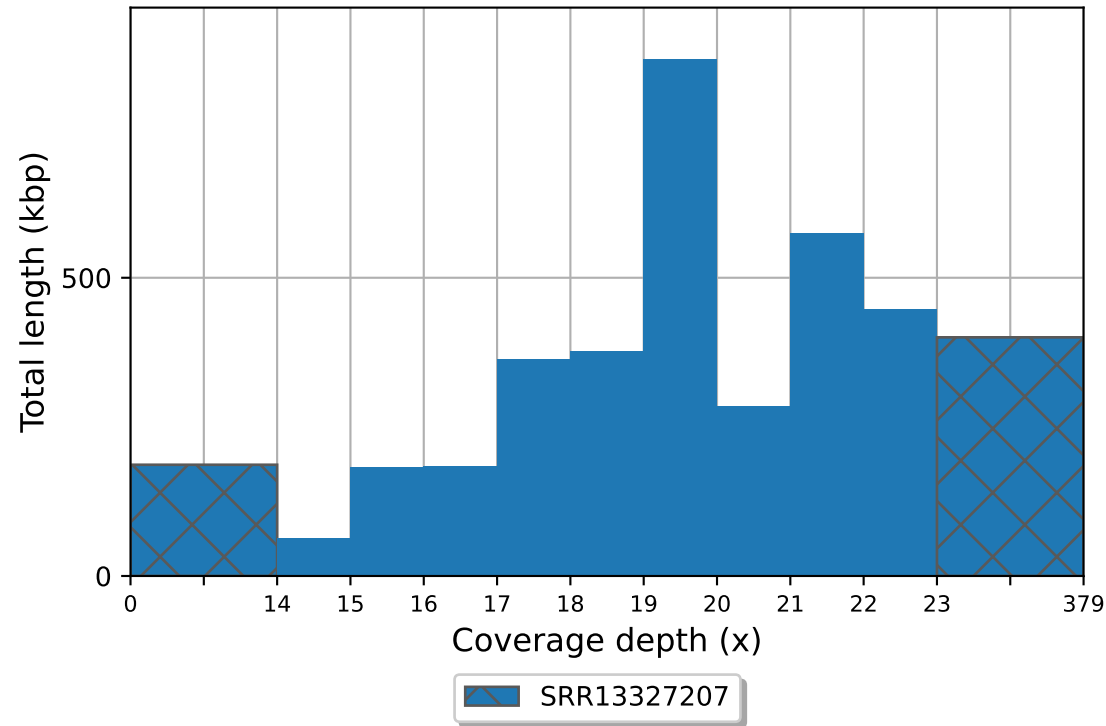
SRR13327207 coverage histogram (bin size: 1x)
