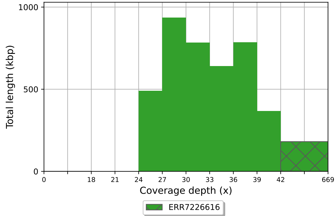
ERR7226616 coverage histogram (bin size: 3x)
