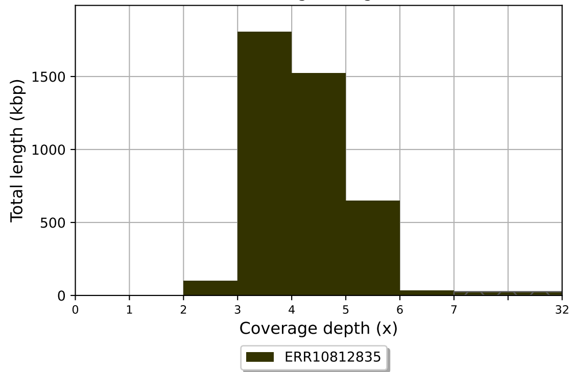
ERR10812835 coverage histogram (bin size: 1x)
