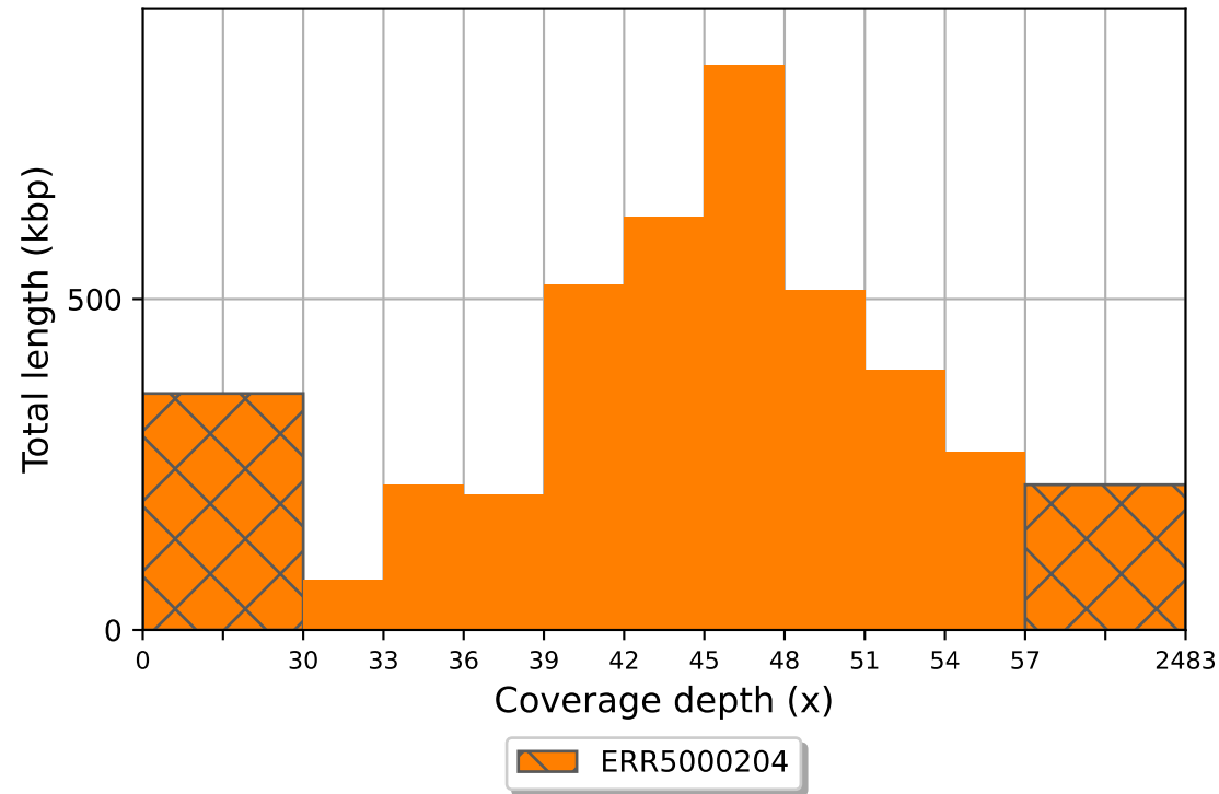
ERR5000204 coverage histogram (bin size: 3x)
