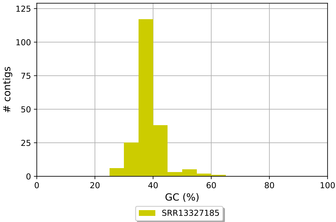
SRR13327185 GC content
