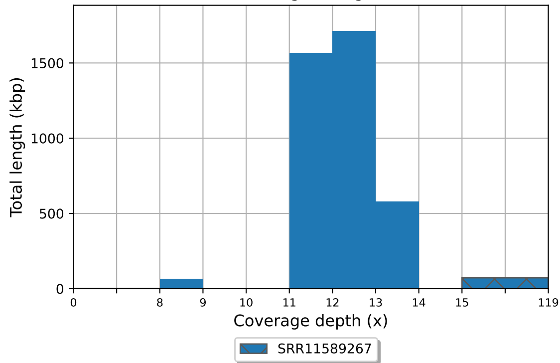
SRR11589267 coverage histogram (bin size: 1x)
