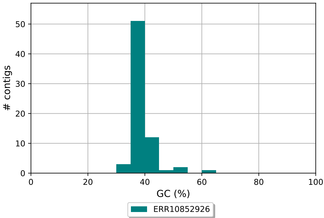
ERR10852926 GC content
