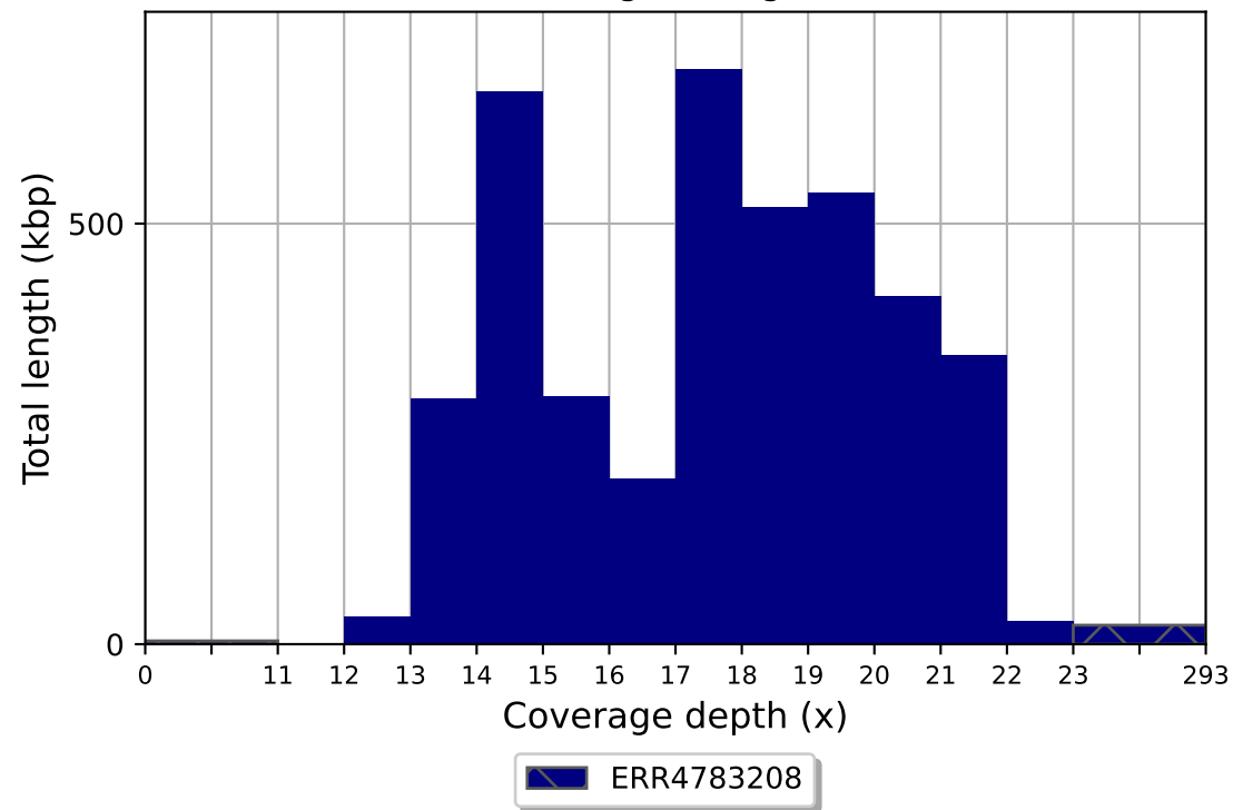
ERR4783208 coverage histogram (bin size: 1x)
