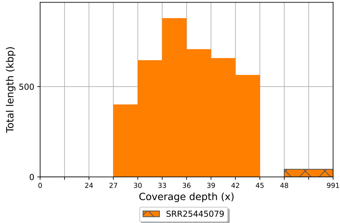
SRR25445079 coverage histogram (bin size: 3x)
