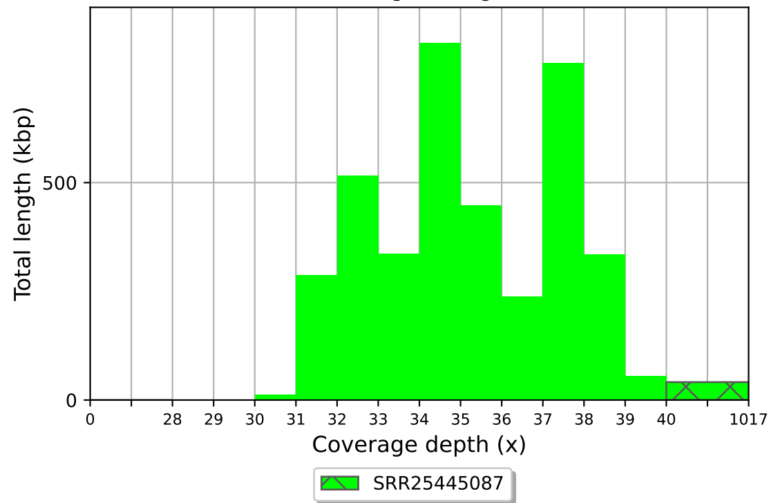
SRR25445087 coverage histogram (bin size: 1x)
