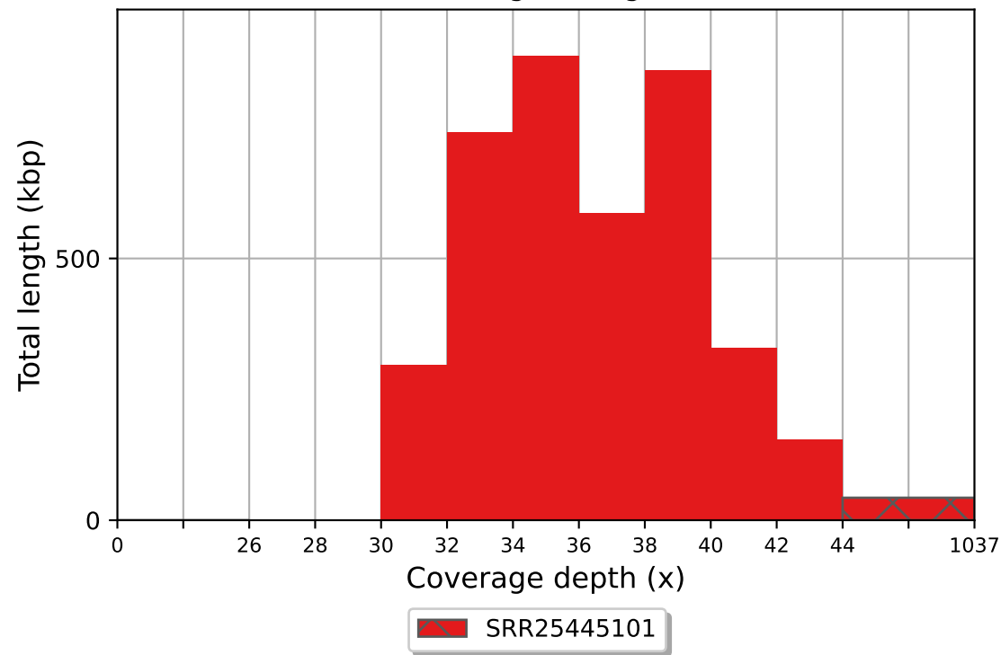
SRR25445101 coverage histogram (bin size: 2x)
