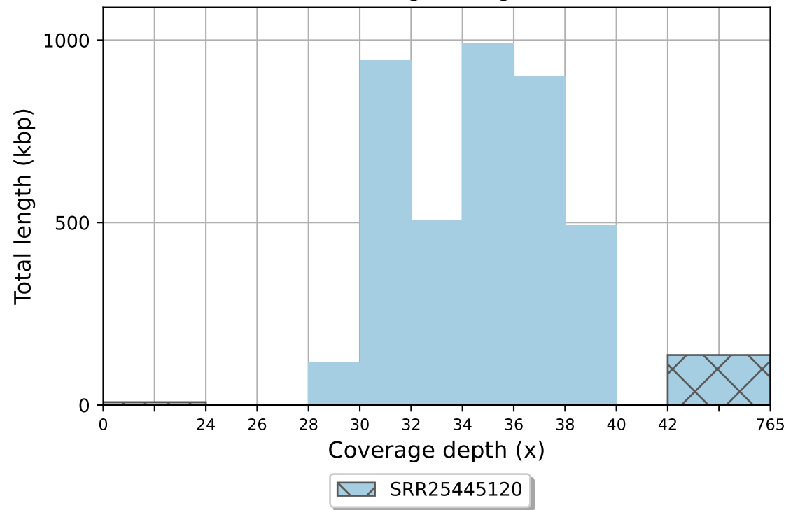
SRR25445120 coverage histogram (bin size: 2x)
