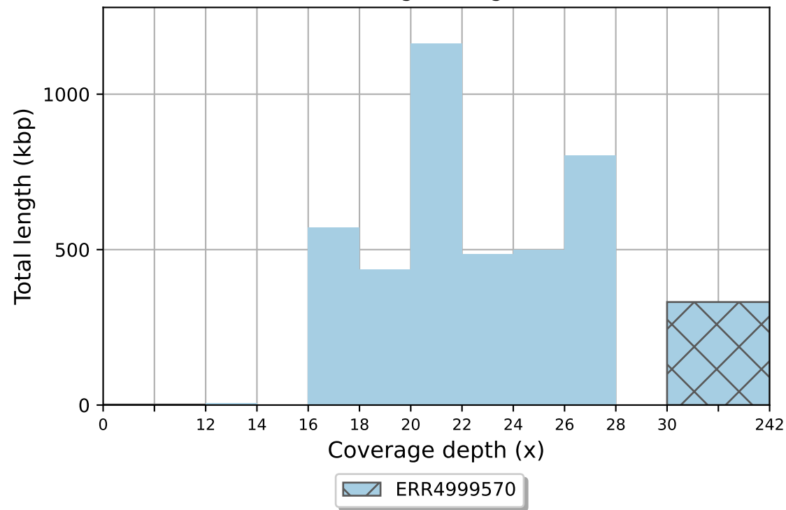
ERR4999570 coverage histogram (bin size: 2x)
