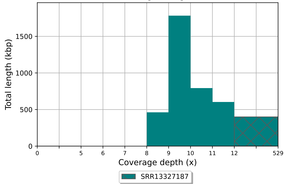
SRR13327187 coverage histogram (bin size: 1x)
