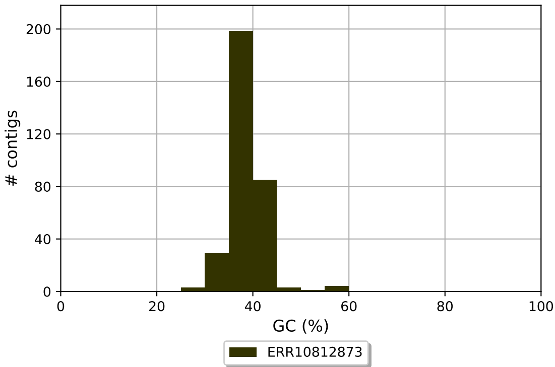
ERR10812873 GC content
