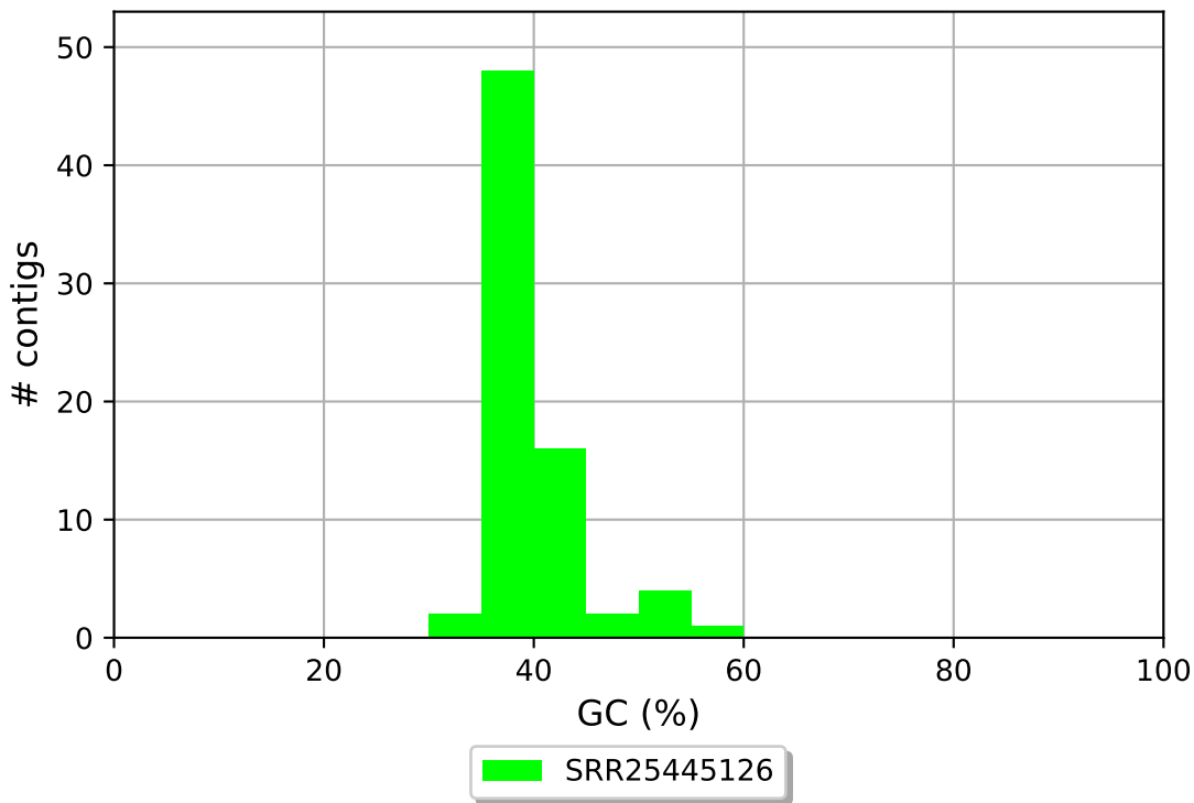
SRR25445126 GC content
