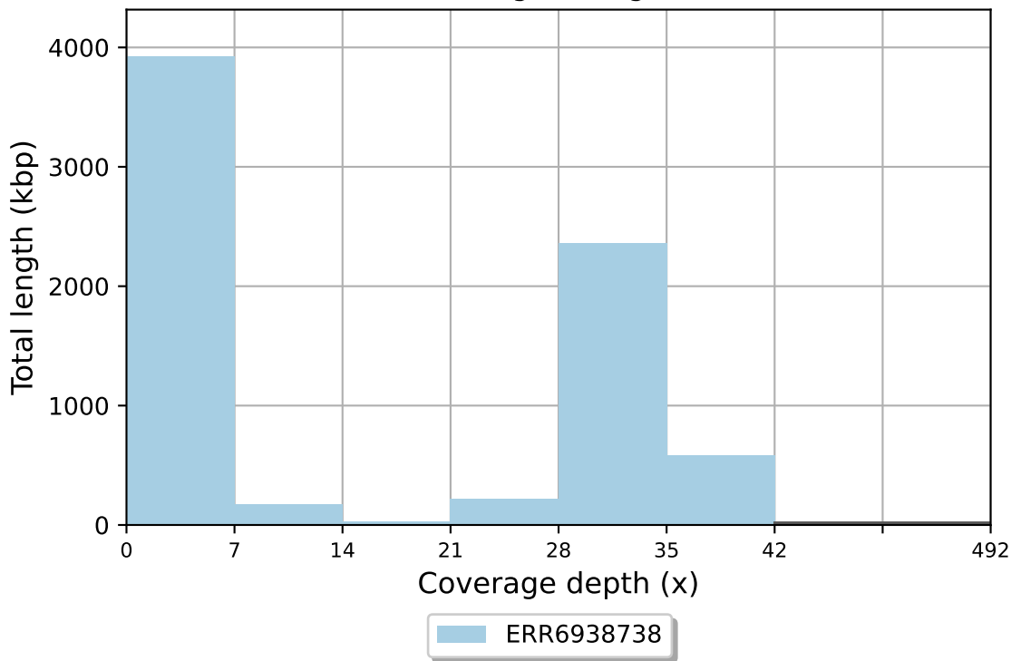
ERR6938738 coverage histogram (bin size: 7x)
