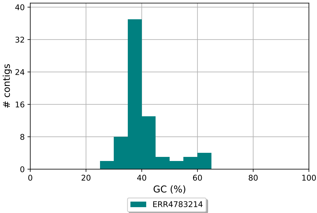
ERR4783214 GC content
