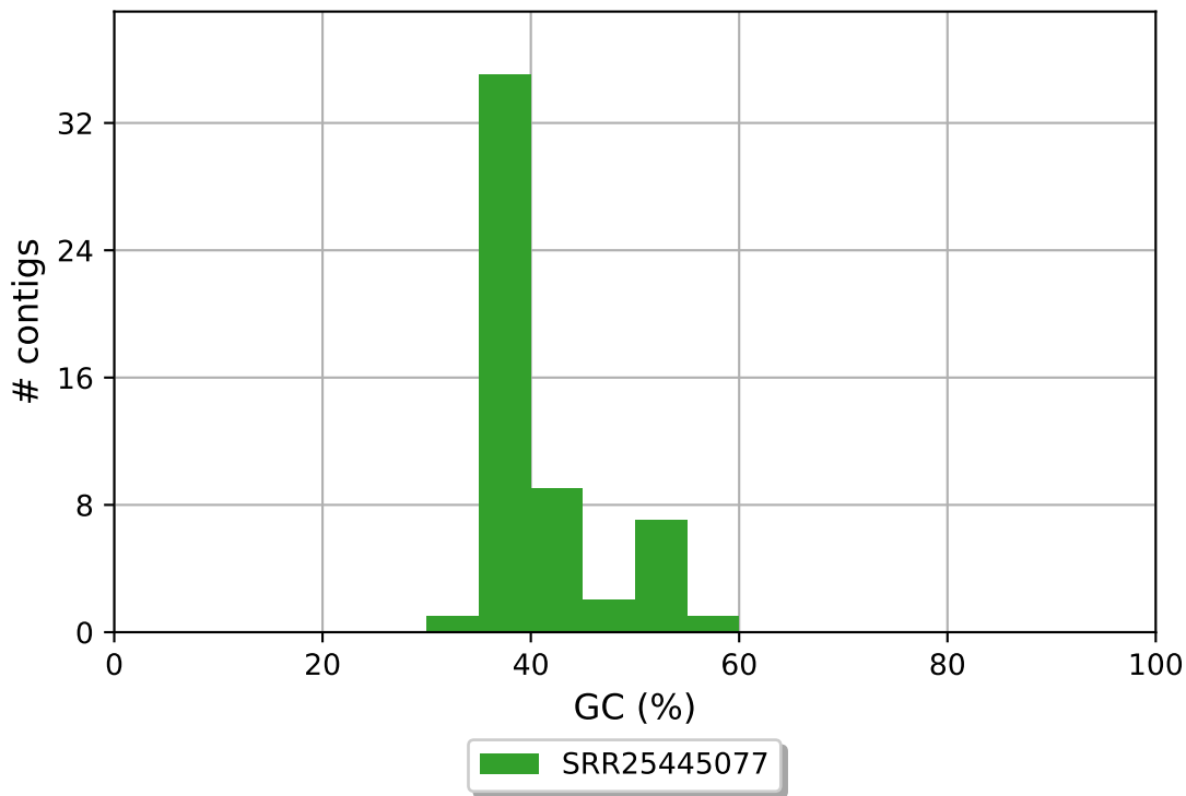
SRR25445077 GC content
