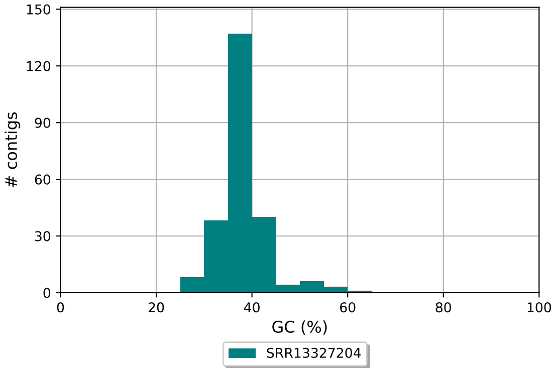
SRR13327204 GC content
