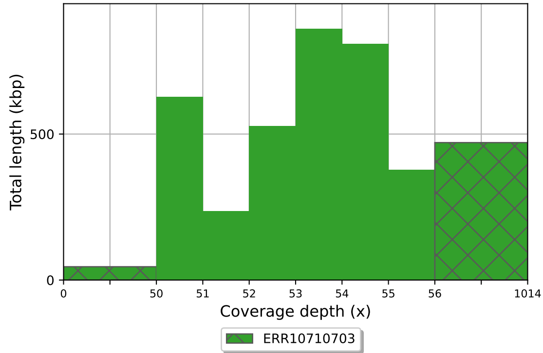
ERR10710703 coverage histogram (bin size: 1x)
