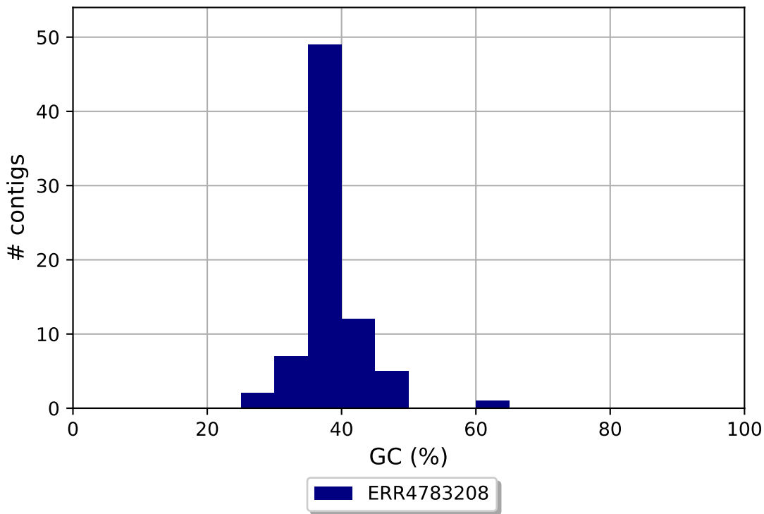
ERR4783208 GC content
