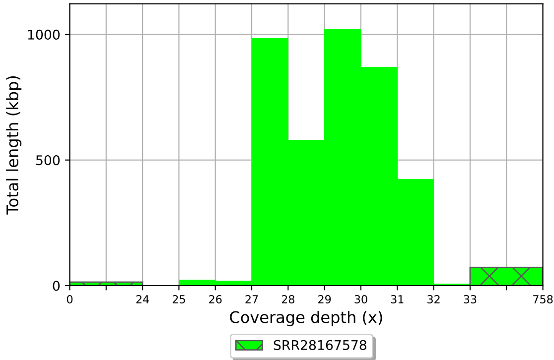
SRR28167578 coverage histogram (bin size: 1x)
