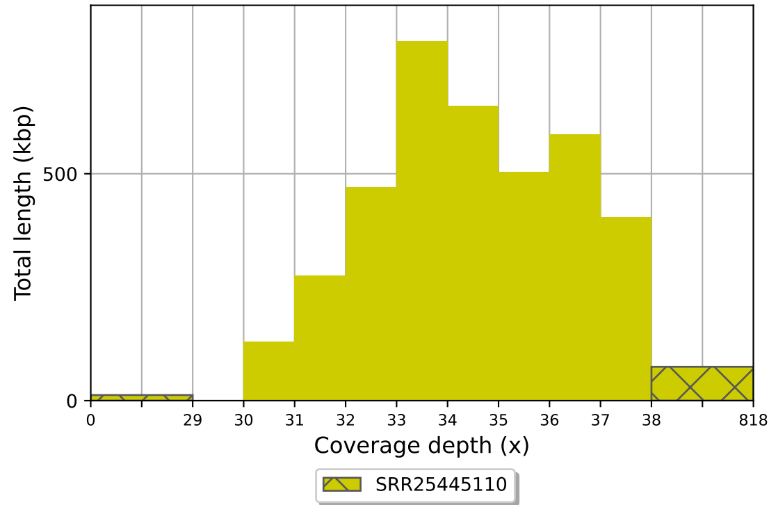
SRR25445110 coverage histogram (bin size: 1x)
