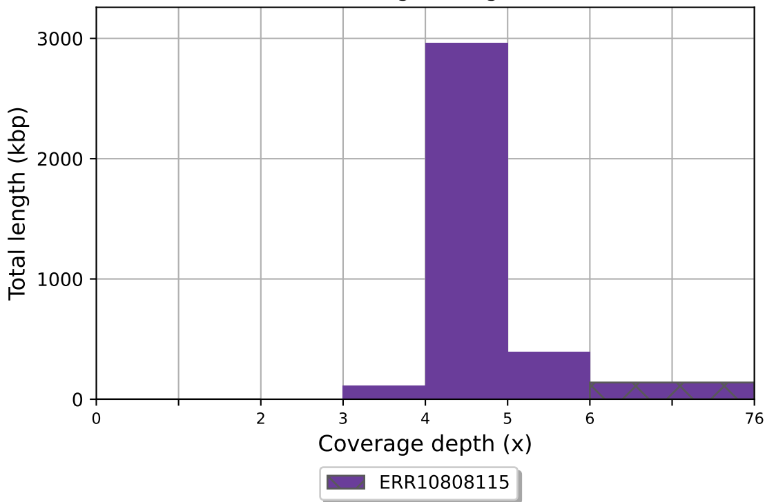
ERR10808115 coverage histogram (bin size: 1x)
