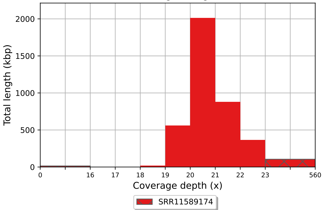
SRR11589174 coverage histogram (bin size: 1x)
