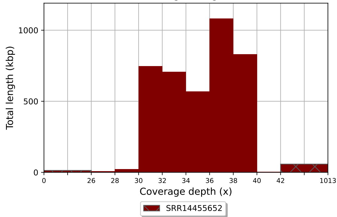
SRR14455652 coverage histogram (bin size: 2x)
