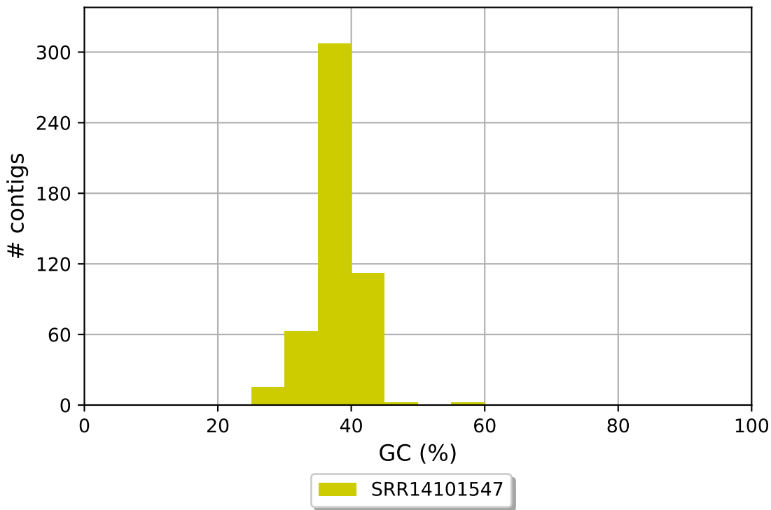
SRR14101547 GC content
