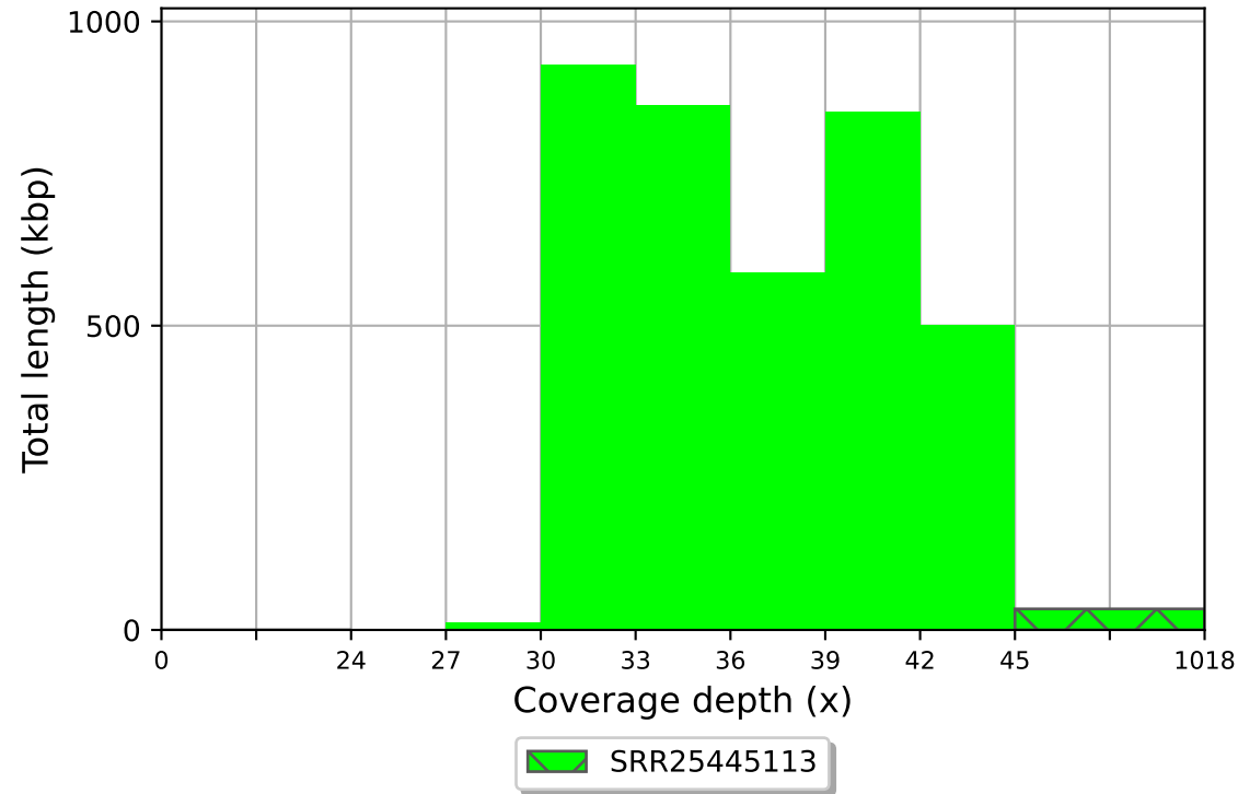
SRR25445113 coverage histogram (bin size: 3x)
