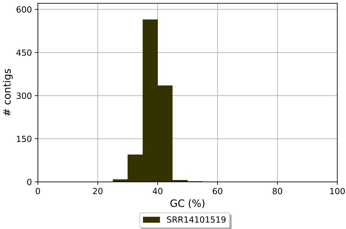
SRR14101519 GC content
