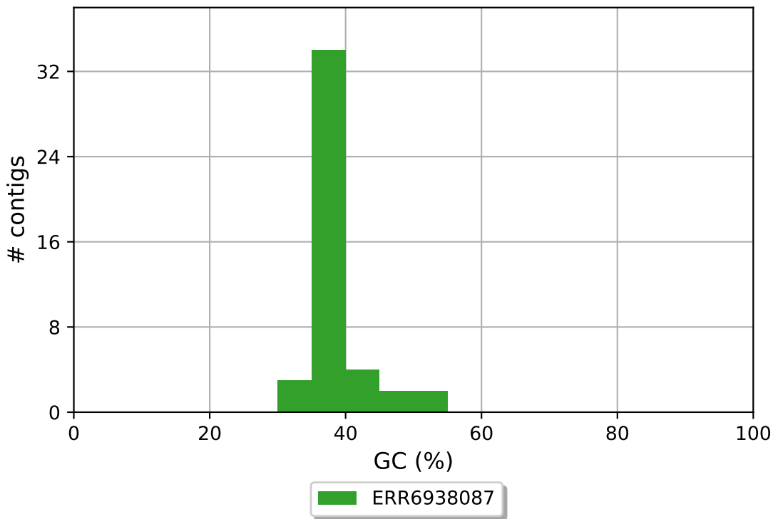
ERR6938087 GC content
