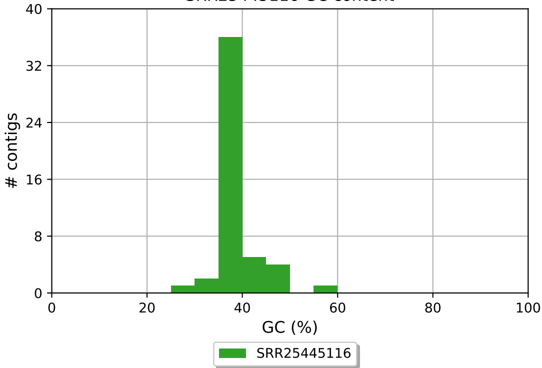
SRR25445116 GC content
