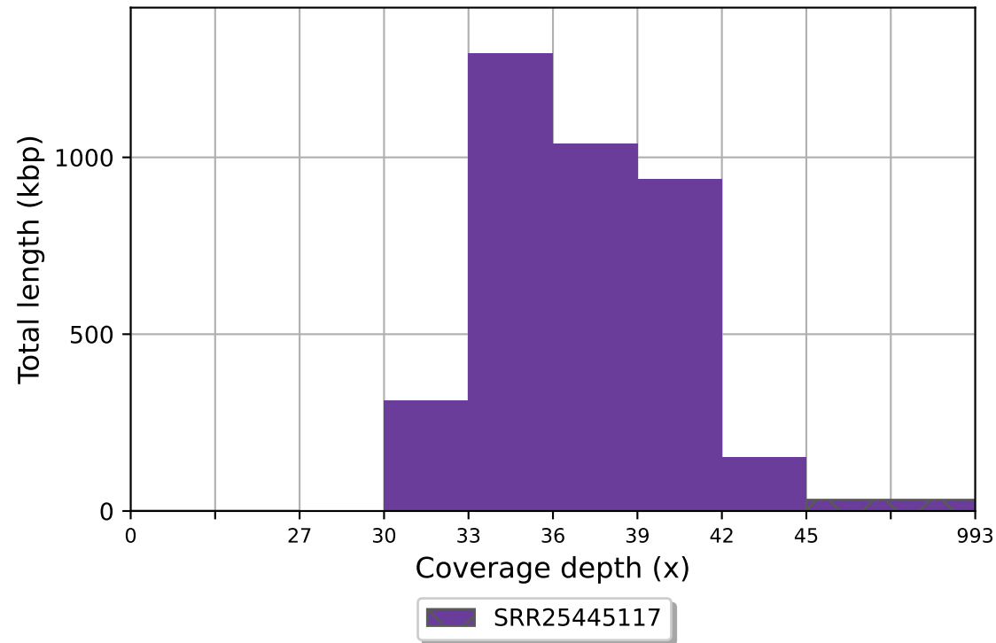
SRR25445117 coverage histogram (bin size: 3x)
