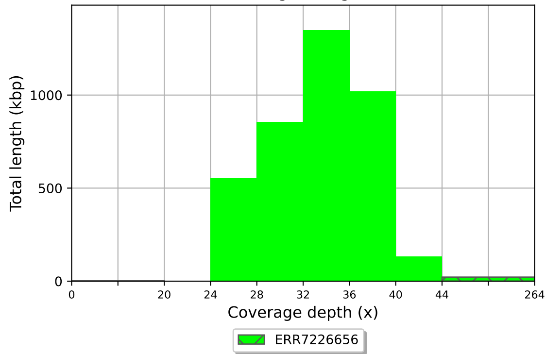
ERR7226656 coverage histogram (bin size: 4x)
