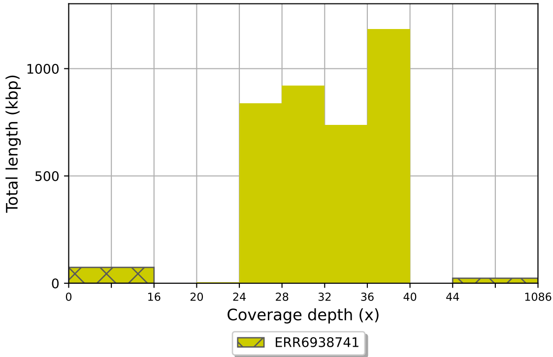
ERR6938741 coverage histogram (bin size: 4x)
