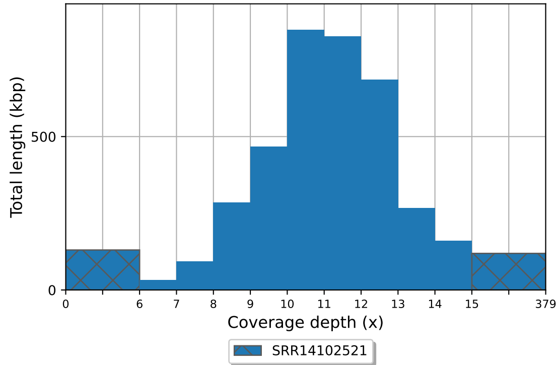
SRR14102521 coverage histogram (bin size: 1x)
