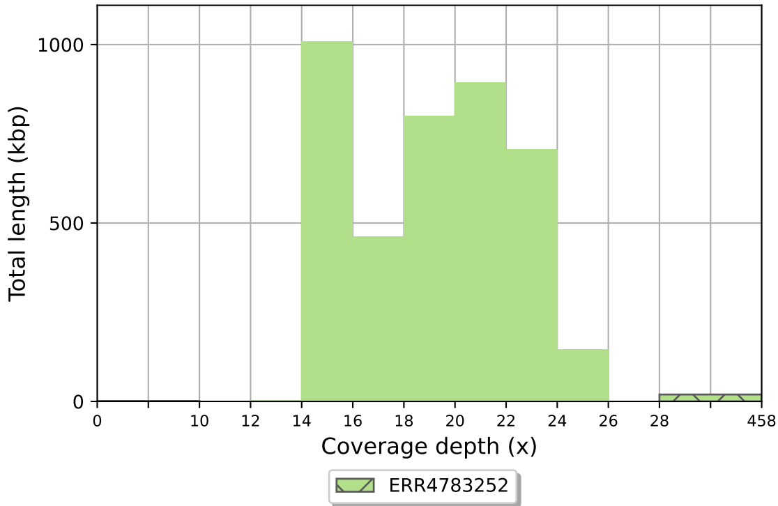
ERR4783252 coverage histogram (bin size: 2x)
