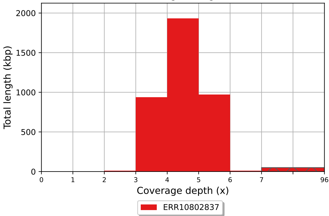
ERR10802837 coverage histogram (bin size: 1x)
