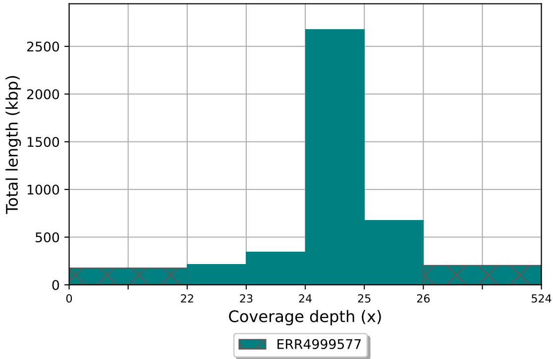
ERR4999577 coverage histogram (bin size: 1x)
