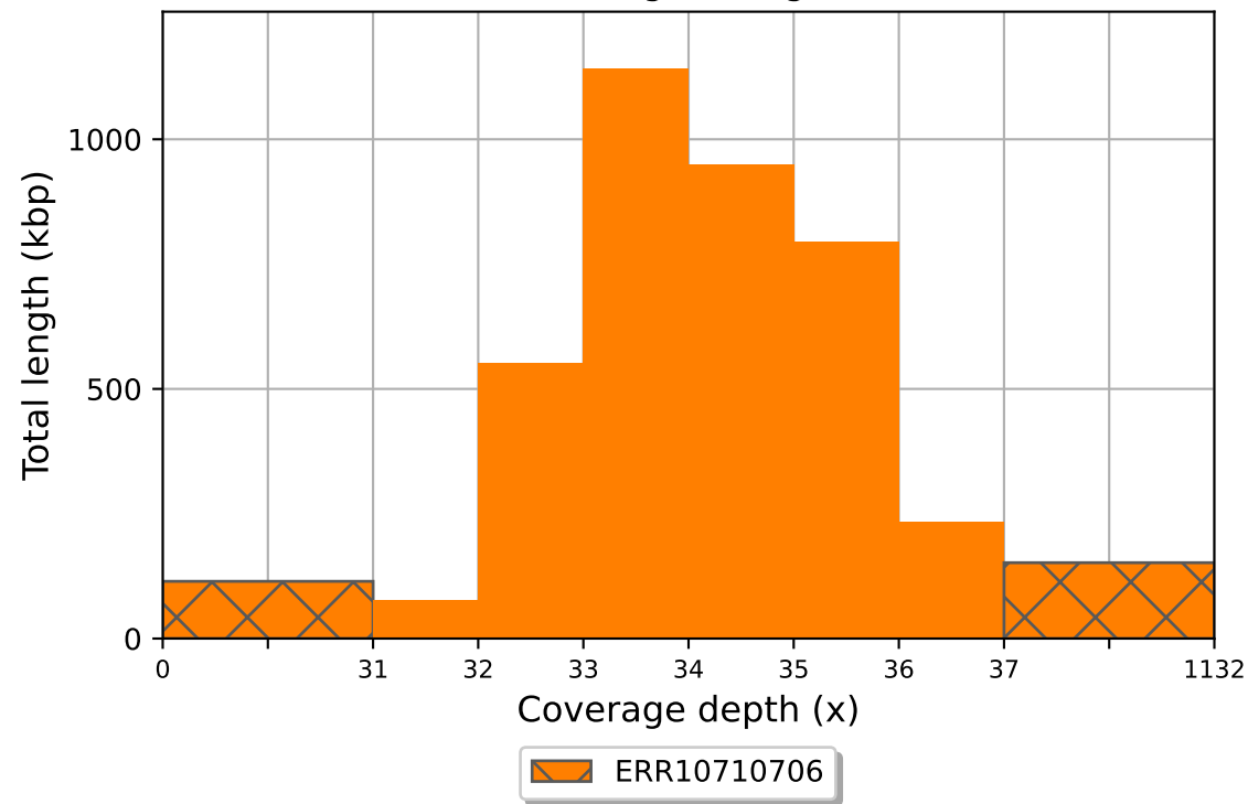
ERR10710706 coverage histogram (bin size: 1x)
