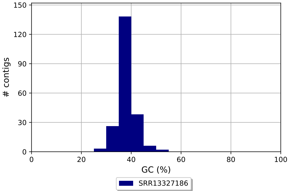
SRR13327186 GC content
