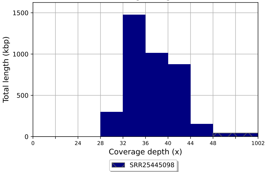
SRR25445098 coverage histogram (bin size: 4x)
