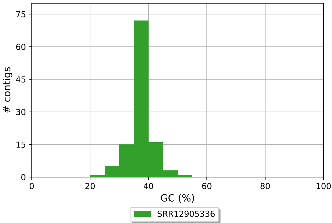
SRR12905336 GC content
