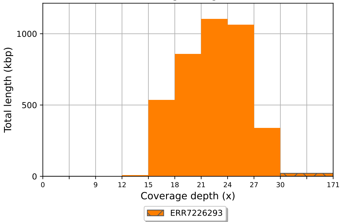
ERR7226293 coverage histogram (bin size: 3x)
