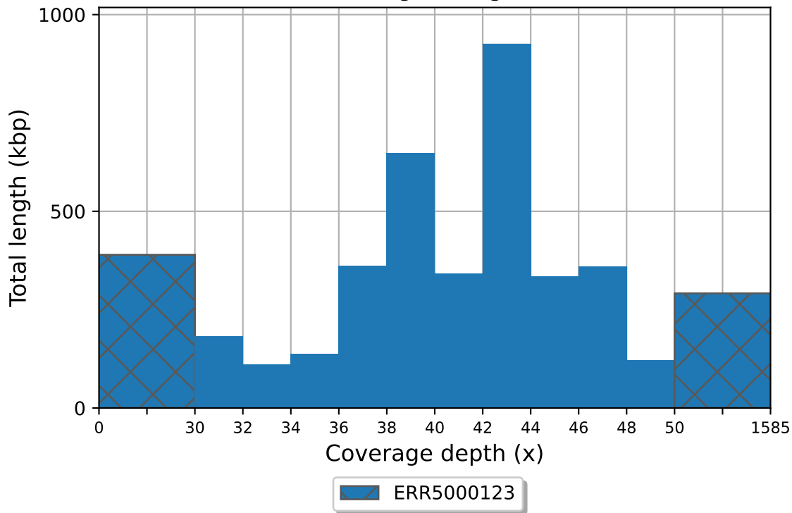
ERR5000123 coverage histogram (bin size: 2x)
