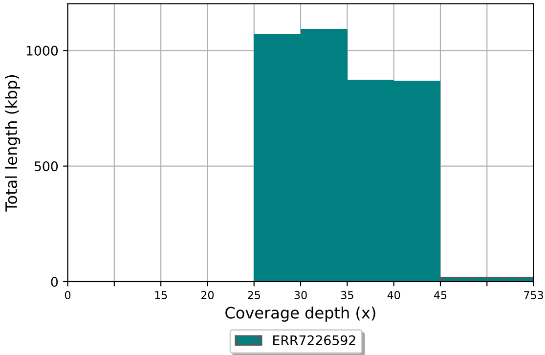
ERR7226592 coverage histogram (bin size: 5x)
