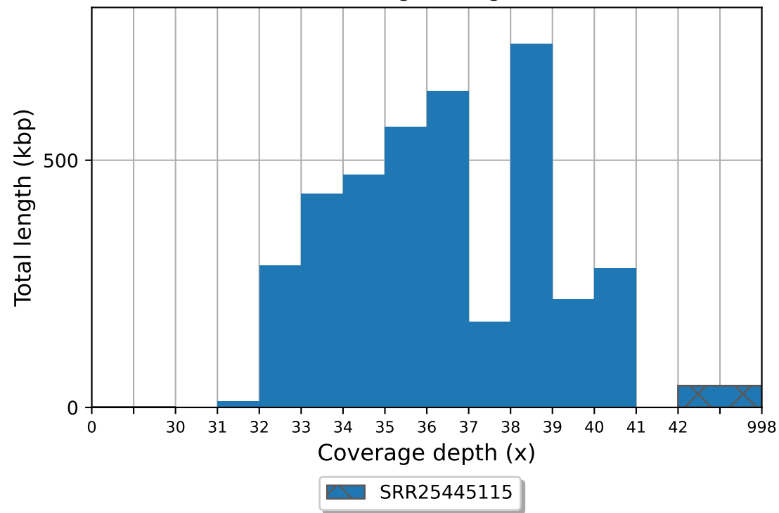
SRR25445115 coverage histogram (bin size: 1x)
