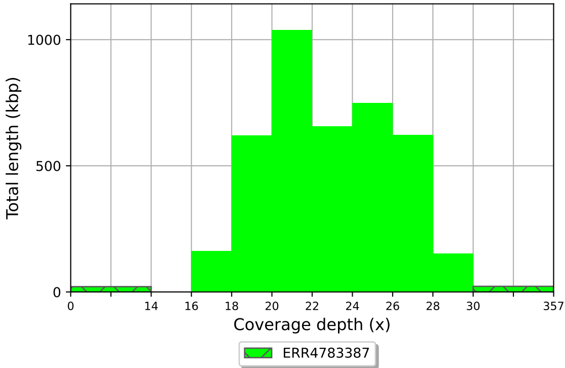
ERR4783387 coverage histogram (bin size: 2x)
