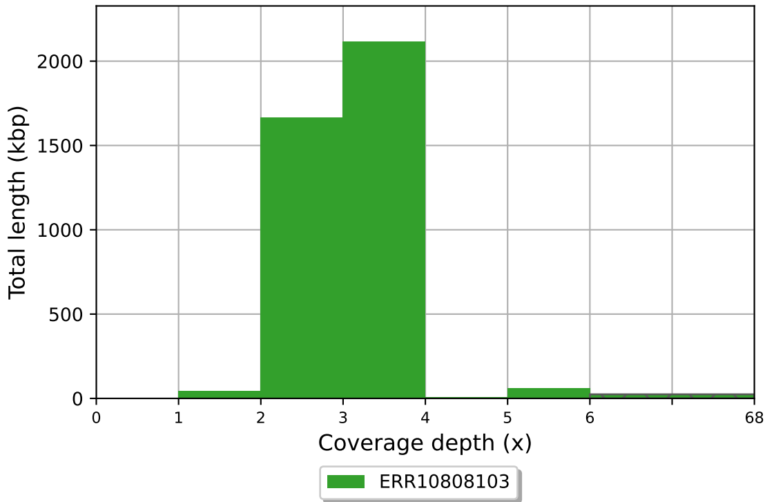
ERR10808103 coverage histogram (bin size: 1x)
