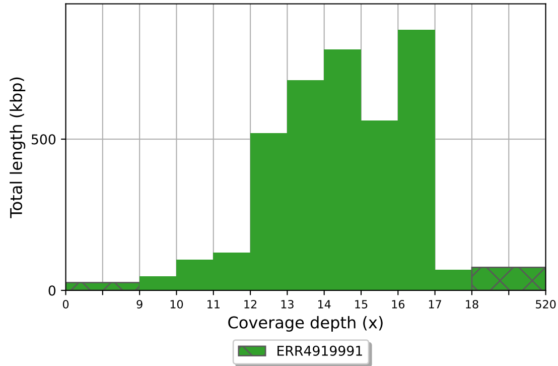
ERR4919991 coverage histogram (bin size: 1x)
