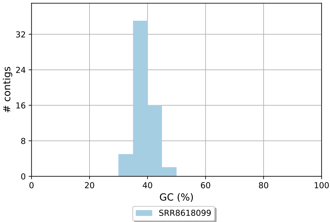
SRR8618099 GC content
