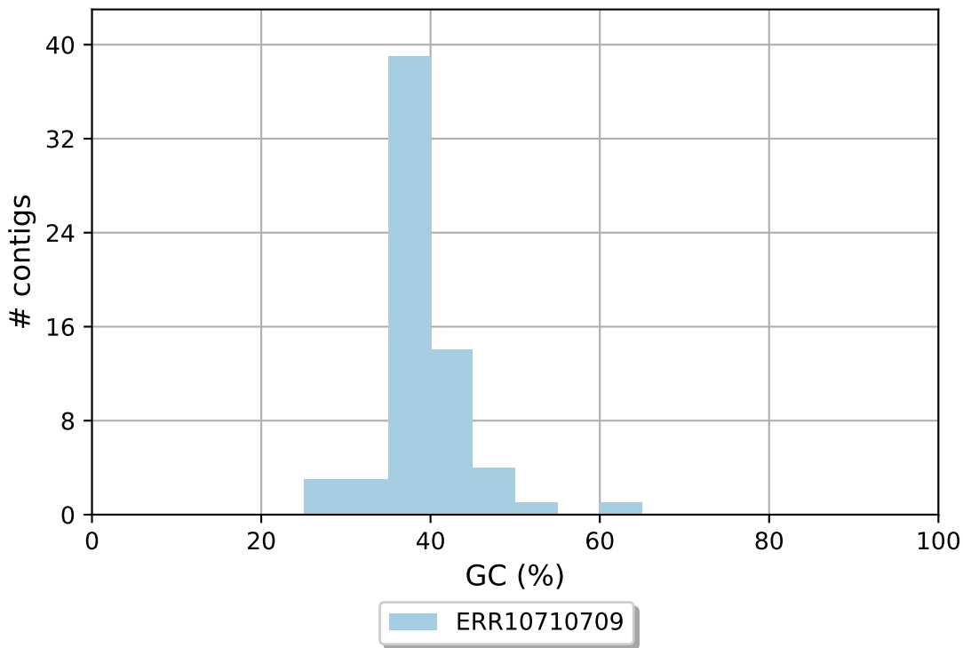
ERR10710709 GC content
