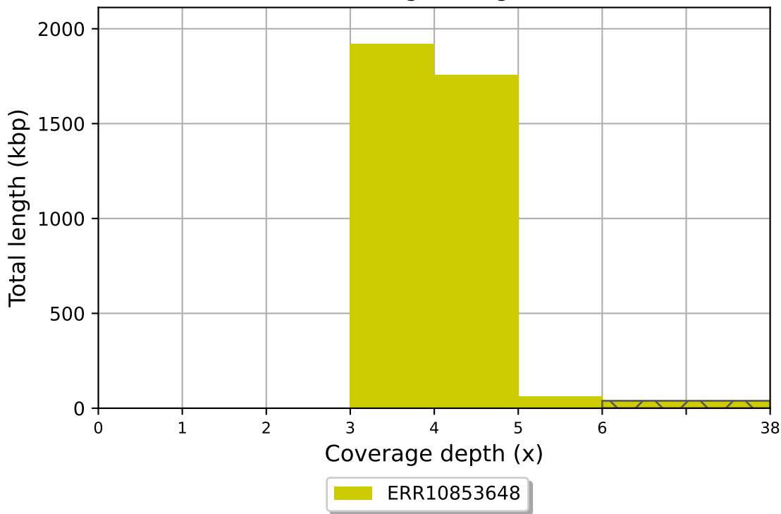
ERR10853648 coverage histogram (bin size: 1x)
