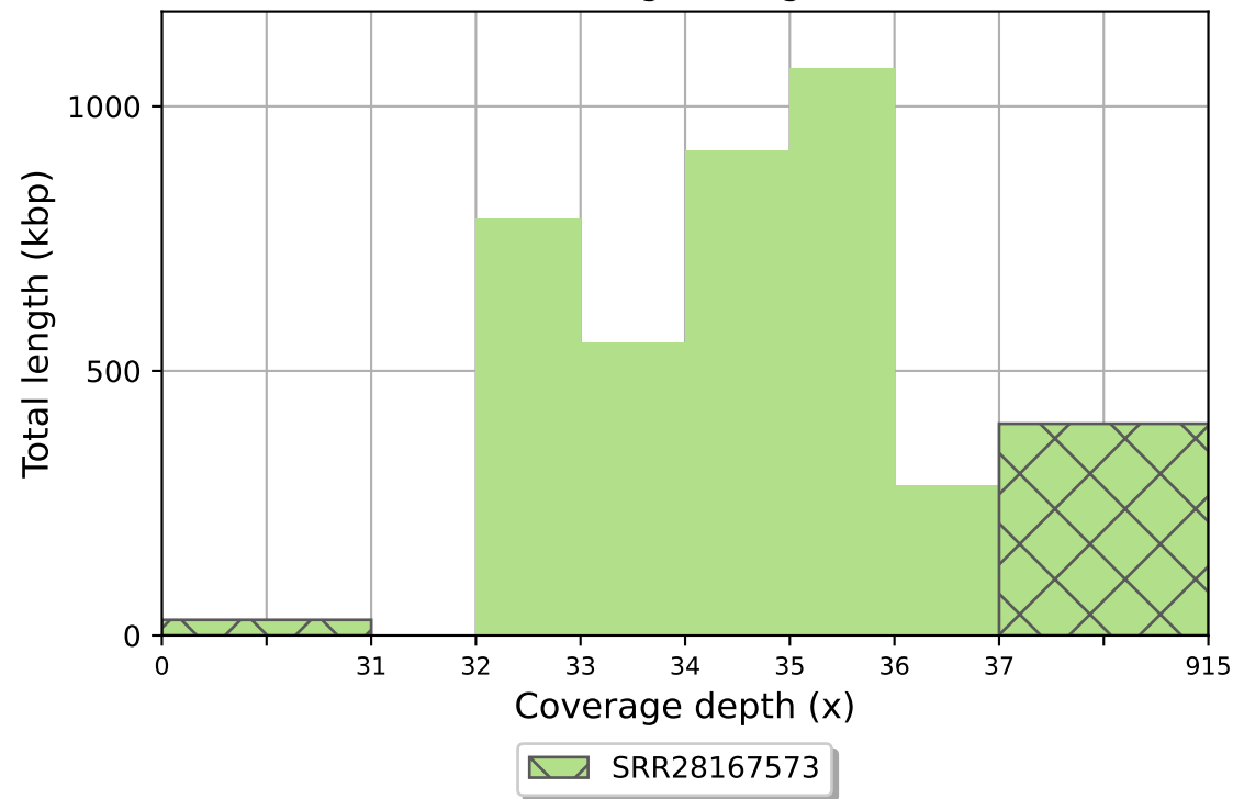
SRR28167573 coverage histogram (bin size: 1x)
