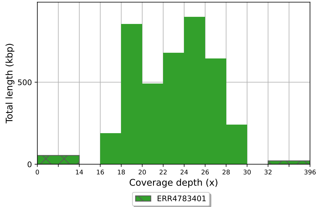
ERR4783401 coverage histogram (bin size: 2x)
