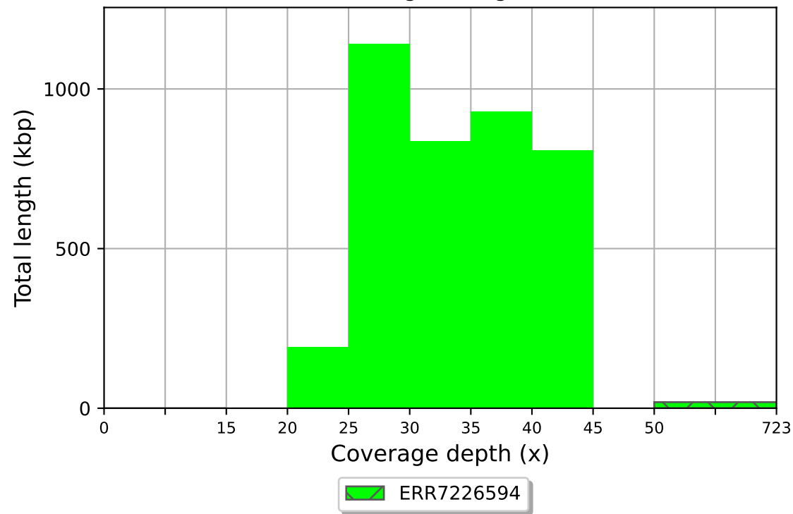
ERR7226594 coverage histogram (bin size: 5x)
