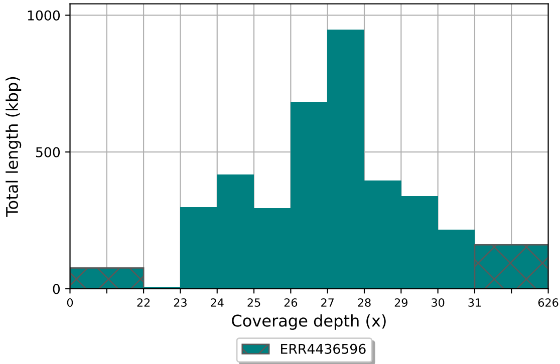
ERR4436596 coverage histogram (bin size: 1x)
