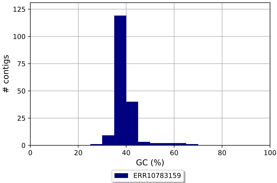
ERR10783159 GC content
