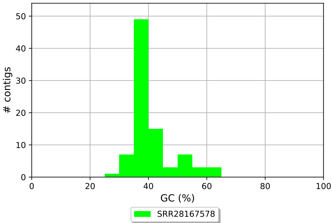
SRR28167578 GC content
