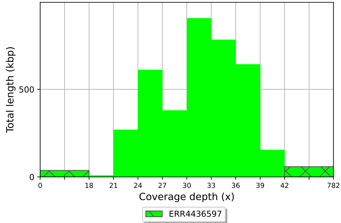
ERR4436597 coverage histogram (bin size: 3x)
