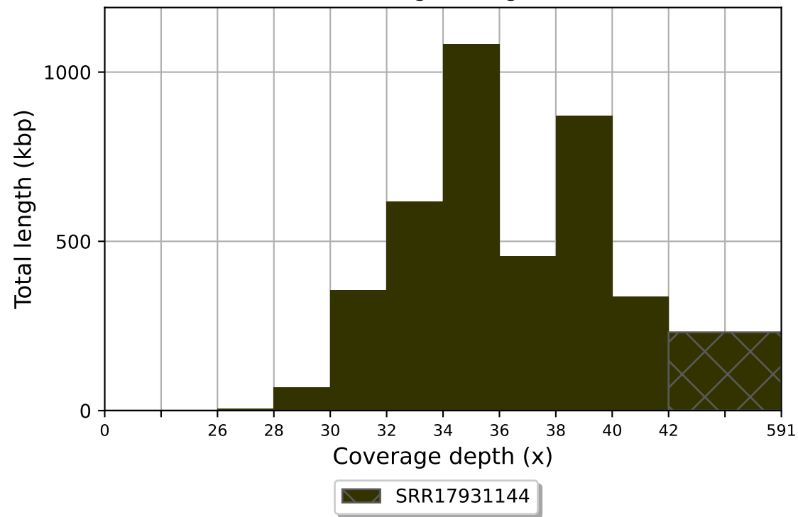
SRR17931144 coverage histogram (bin size: 2x)
