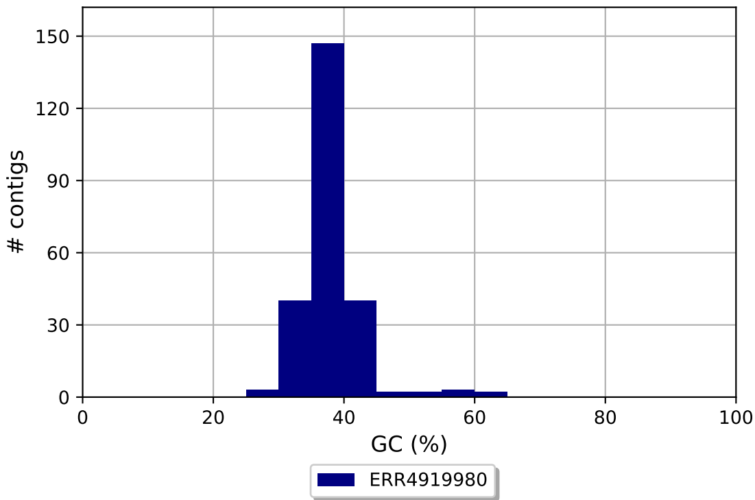
ERR4919980 GC content
