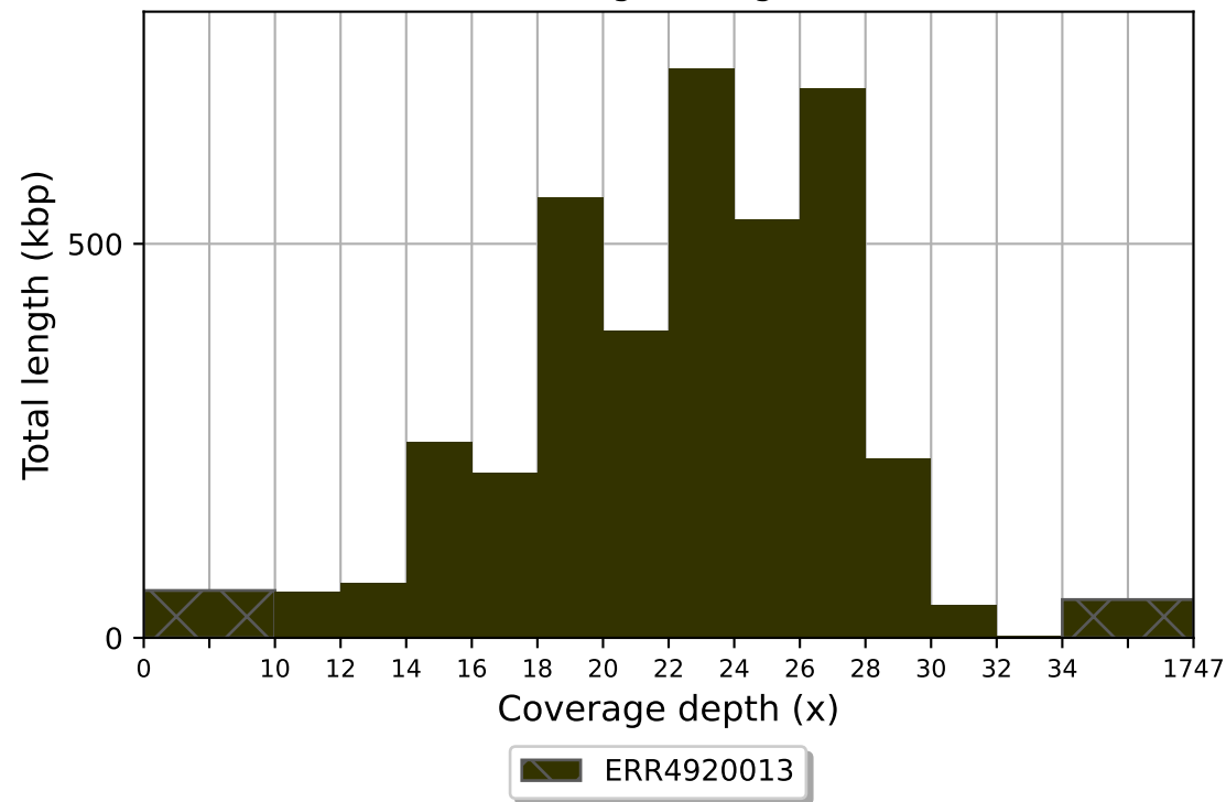
ERR4920013 coverage histogram (bin size: 2x)
