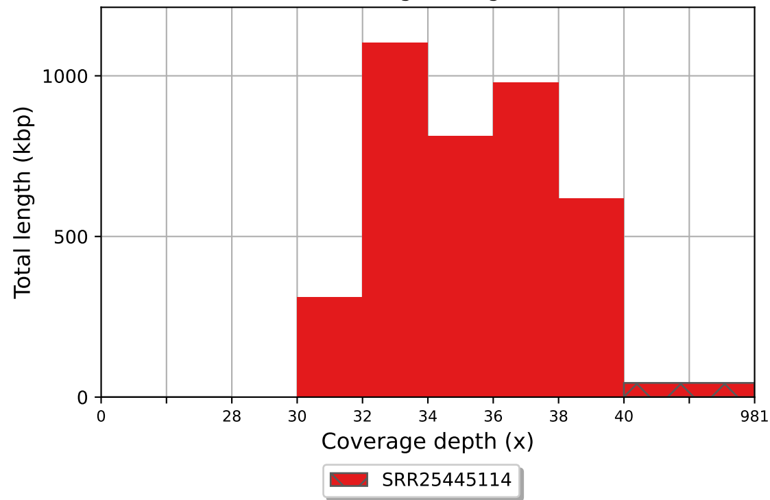
SRR25445114 coverage histogram (bin size: 2x)
