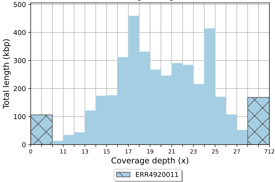
ERR4920011 coverage histogram (bin size: 1x)
