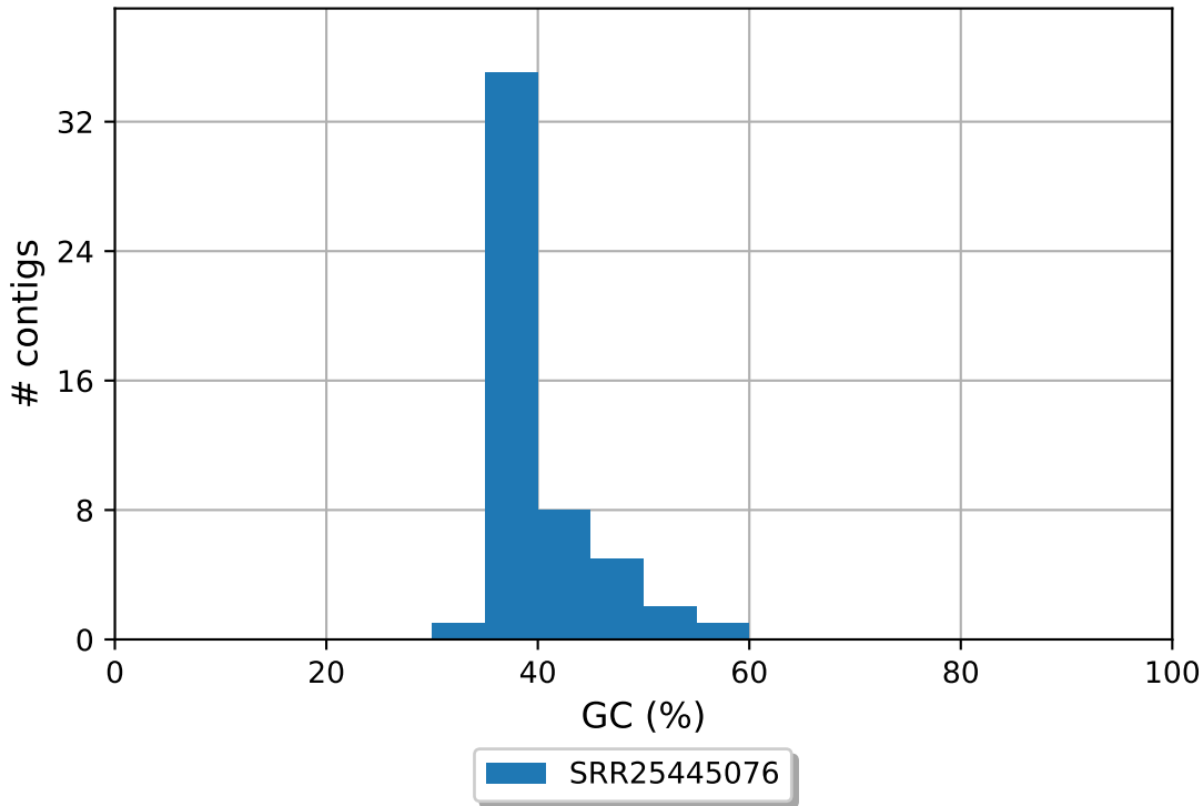
SRR25445076 GC content
