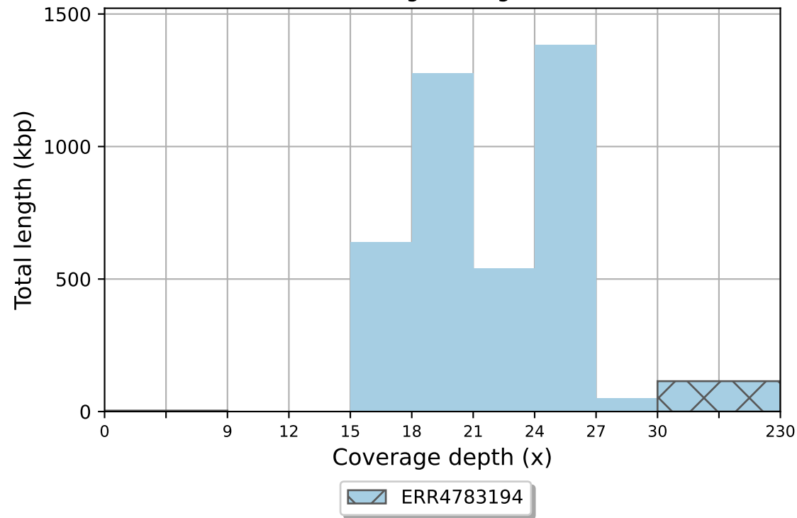
ERR4783194 coverage histogram (bin size: 3x)
