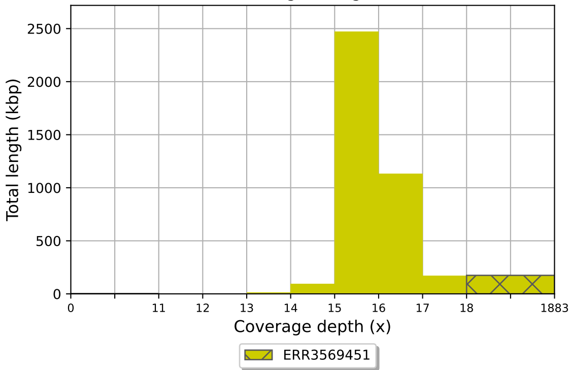
ERR3569451 coverage histogram (bin size: 1x)
