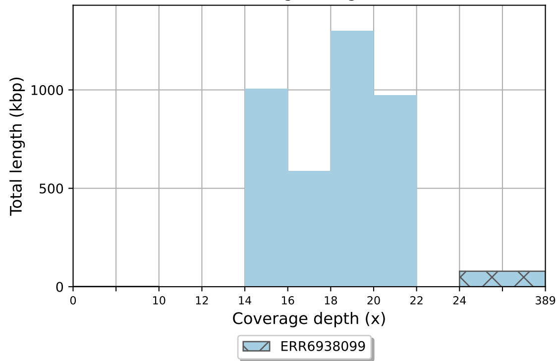
ERR6938099 coverage histogram (bin size: 2x)
