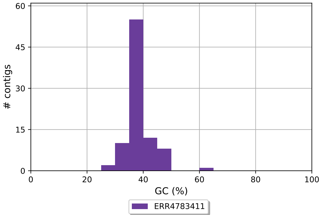
ERR4783411 GC content
