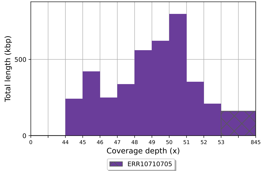
ERR10710705 coverage histogram (bin size: 1x)
