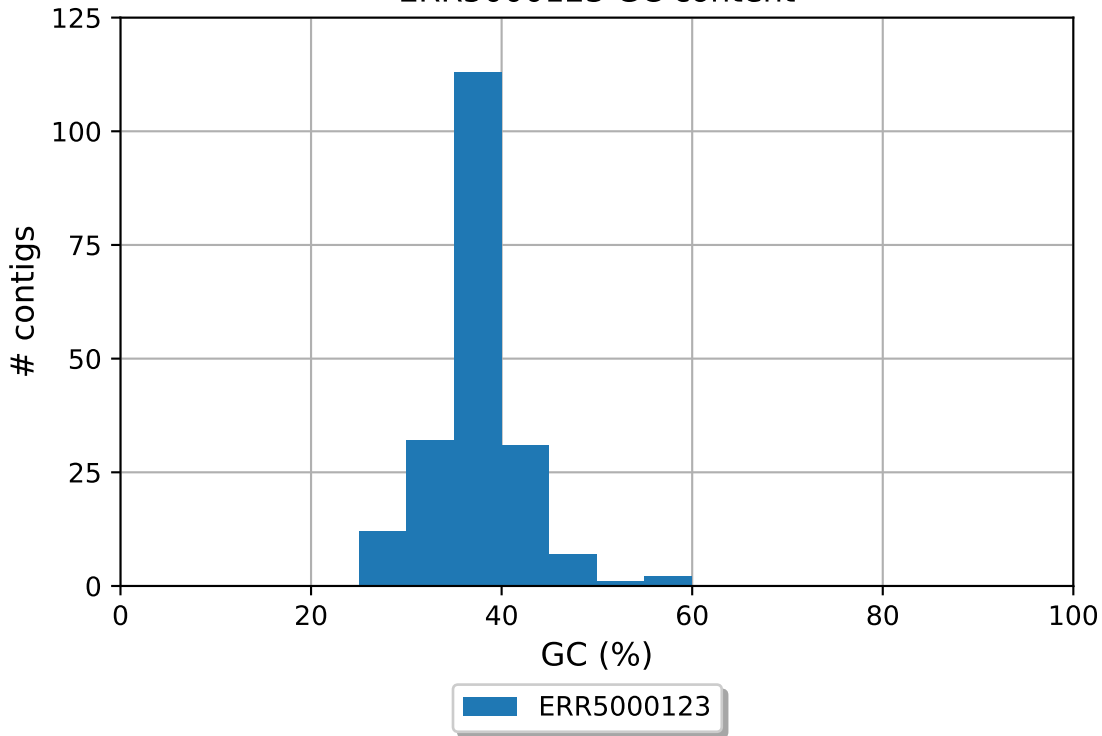
ERR5000123 GC content
