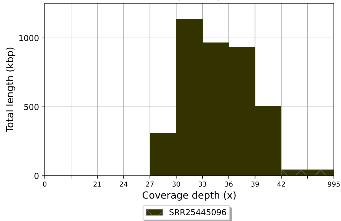
SRR25445096 coverage histogram (bin size: 3x)
