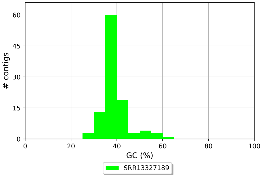
SRR13327189 GC content
