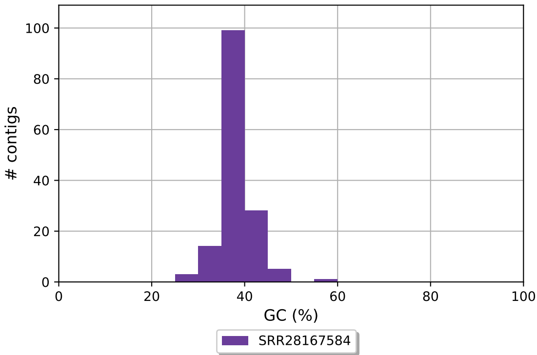
SRR28167584 GC content
