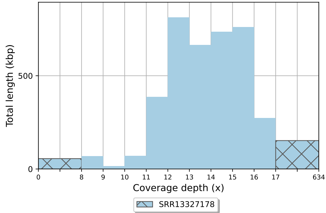
SRR13327178 coverage histogram (bin size: 1x)
