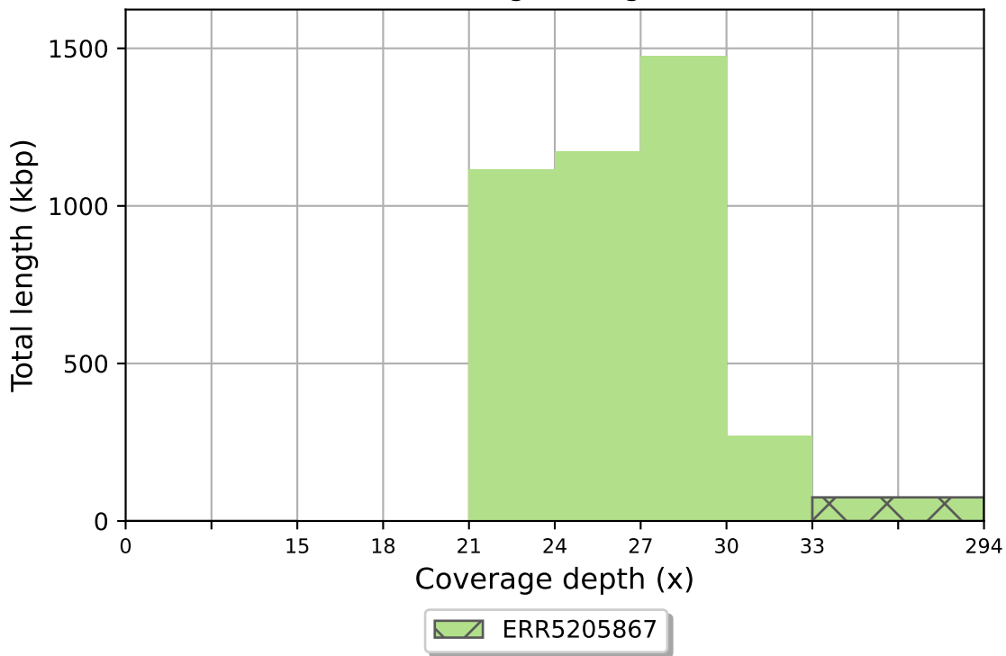
ERR5205867 coverage histogram (bin size: 3x)
