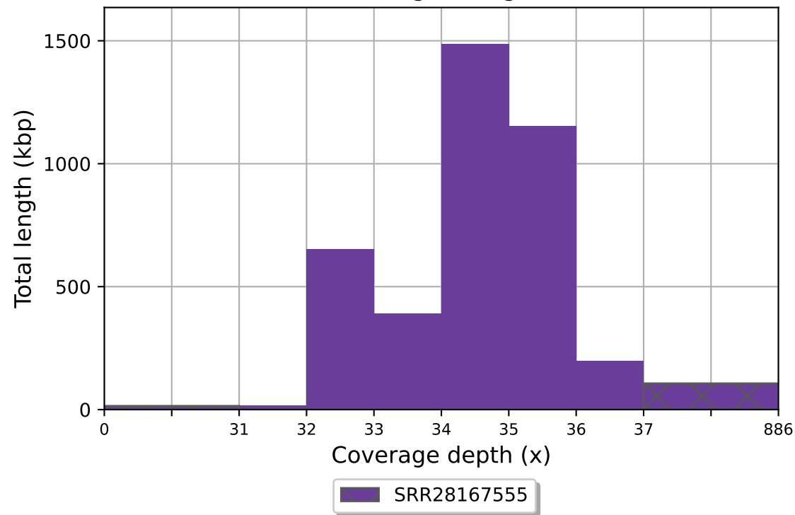
SRR28167555 coverage histogram (bin size: 1x)
