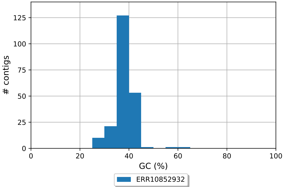
ERR10852932 GC content
