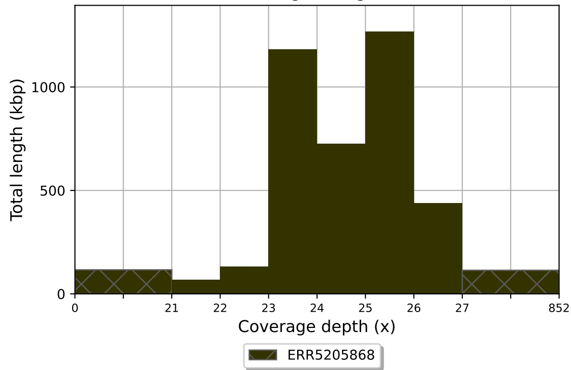
ERR5205868 coverage histogram (bin size: 1x)
