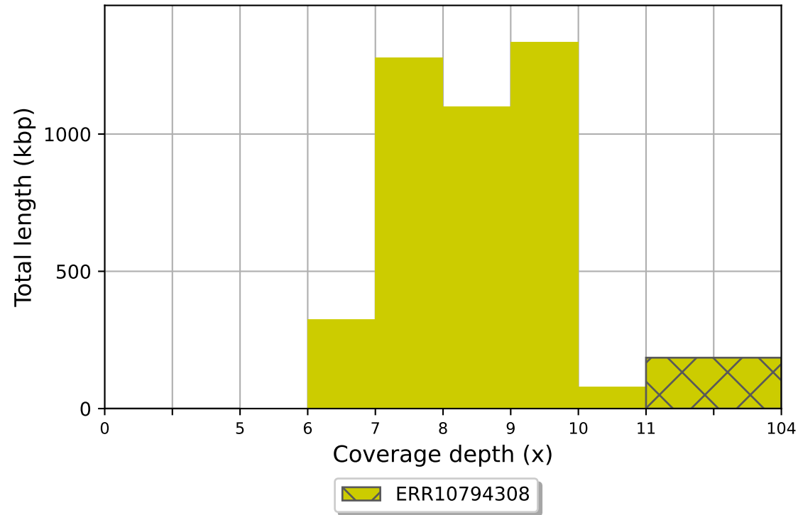
ERR10794308 coverage histogram (bin size: 1x)
