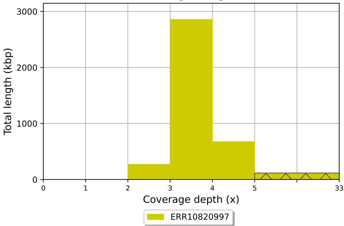
ERR10820997 coverage histogram (bin size: 1x)
