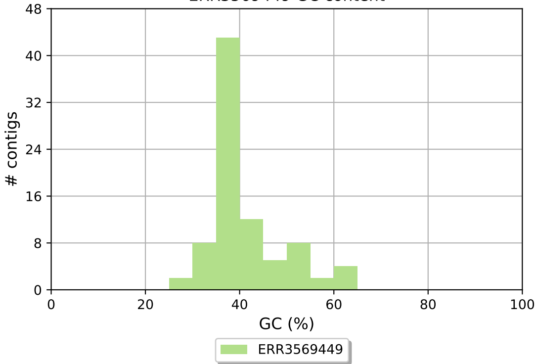
ERR3569449 GC content
