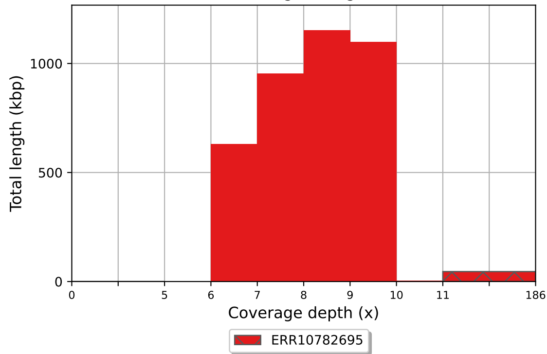
ERR10782695 coverage histogram (bin size: 1x)
