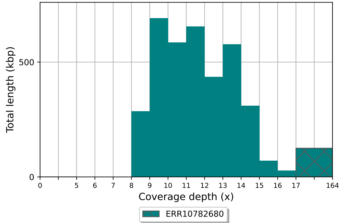
ERR10782680 coverage histogram (bin size: 1x)
