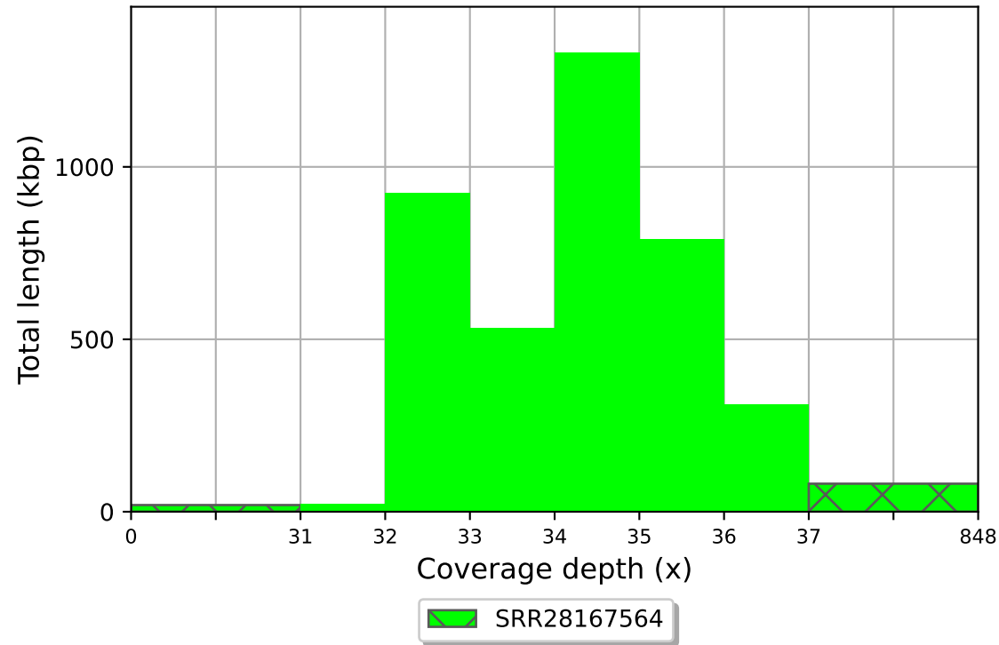
SRR28167564 coverage histogram (bin size: 1x)
