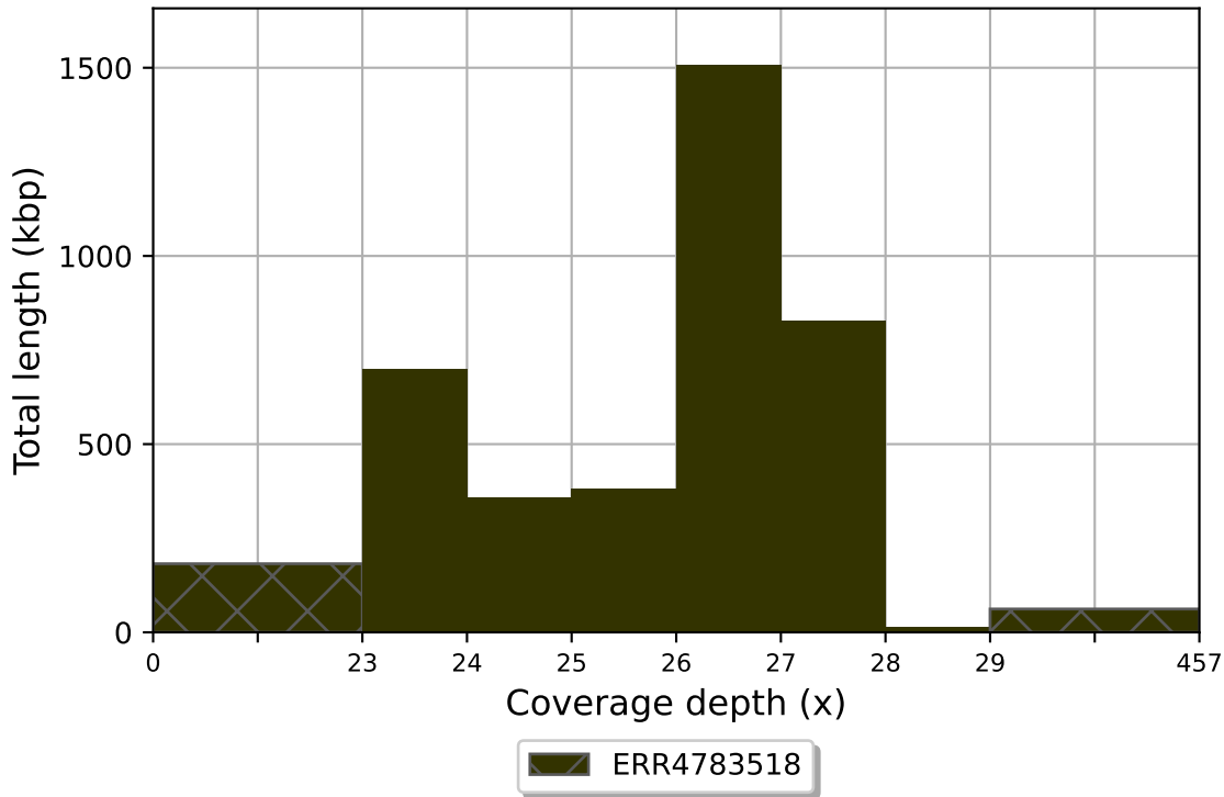
ERR4783518 coverage histogram (bin size: 1x)
