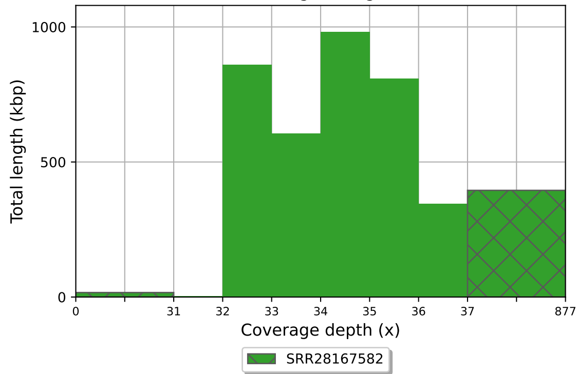
SRR28167582 coverage histogram (bin size: 1x)
