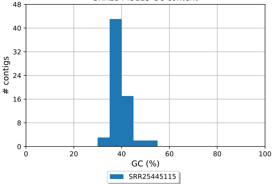
SRR25445115 GC content
