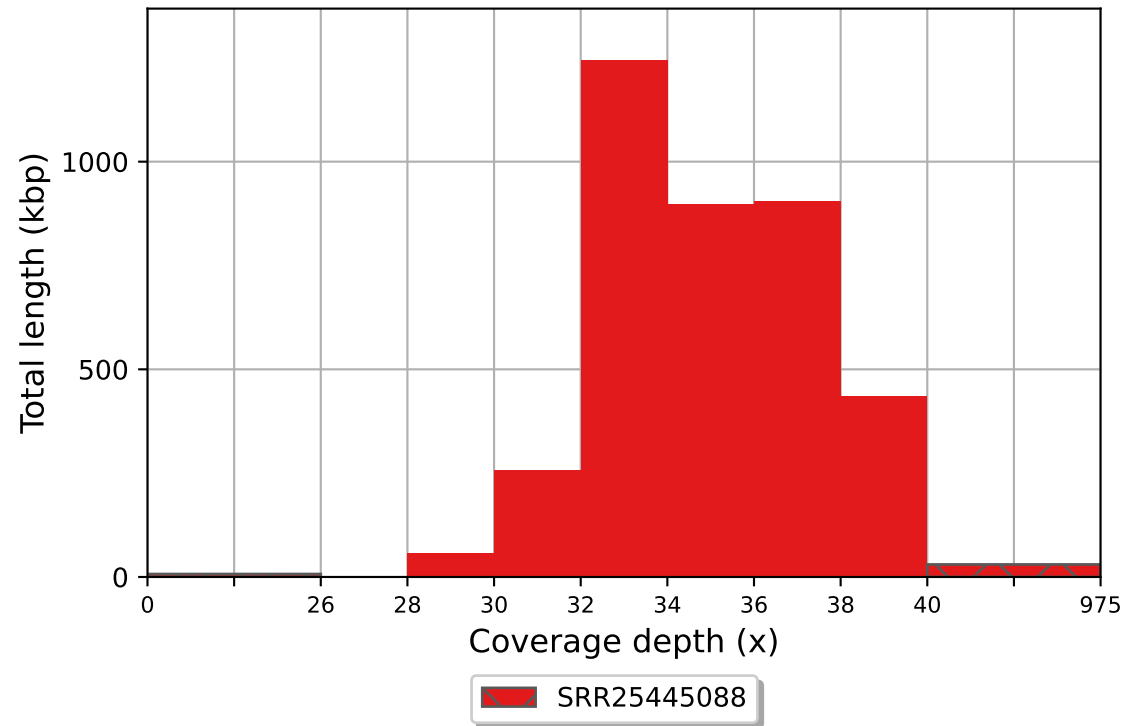
SRR25445088 coverage histogram (bin size: 2x)
