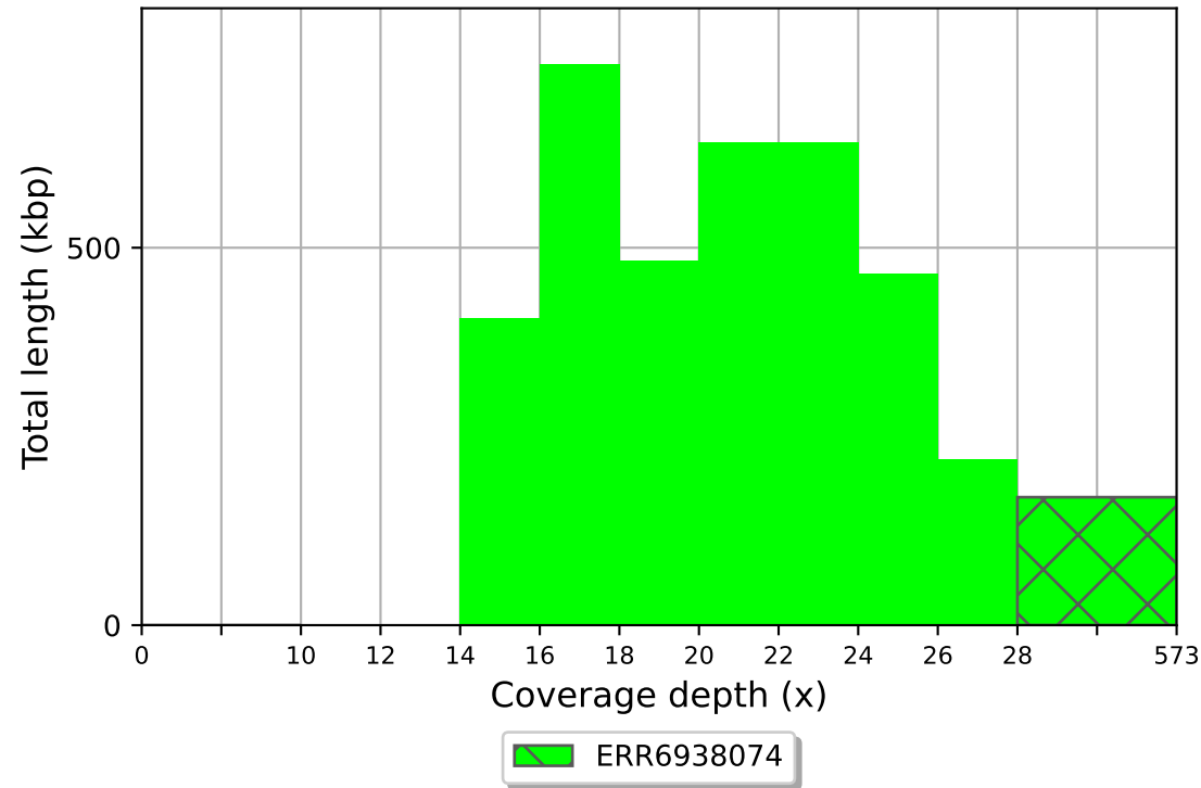
ERR6938074 coverage histogram (bin size: 2x)
