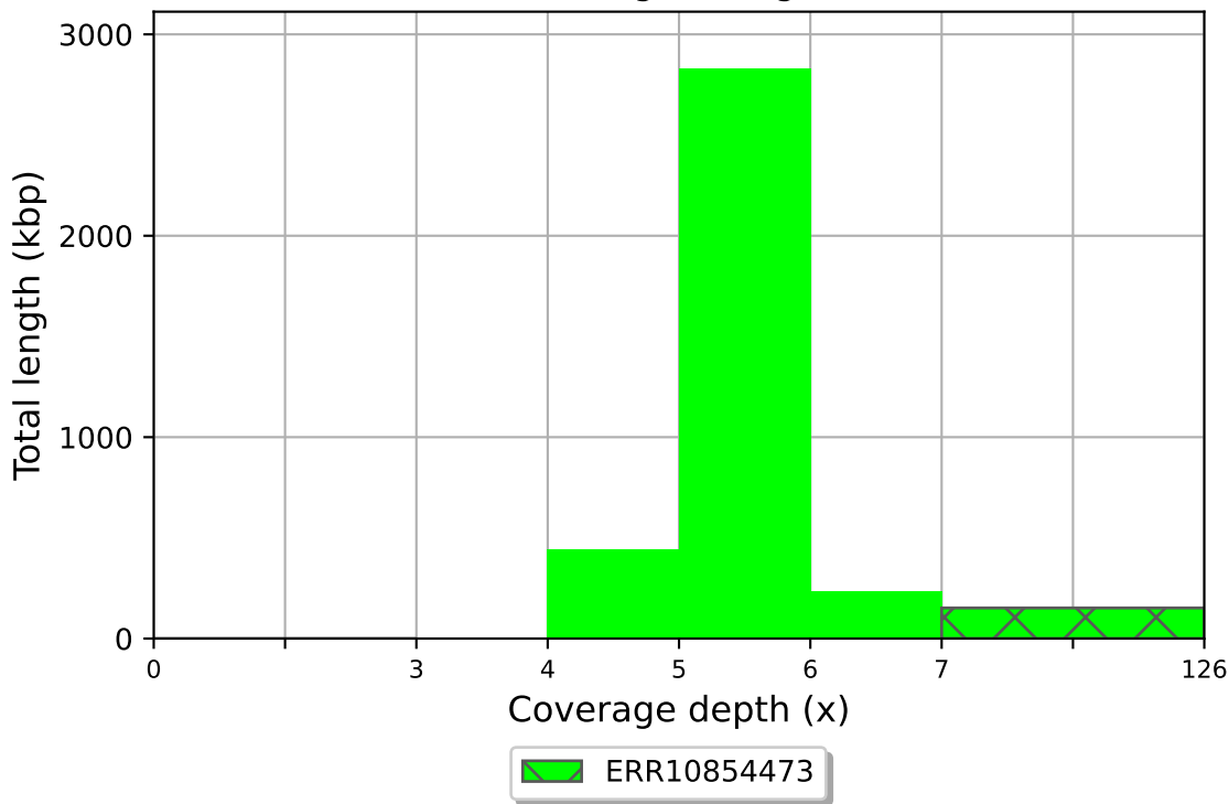
ERR10854473 coverage histogram (bin size: 1x)
