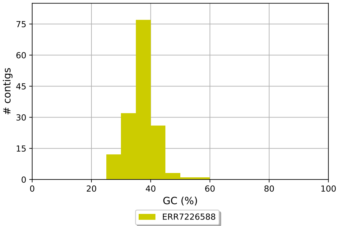
ERR7226588 GC content
