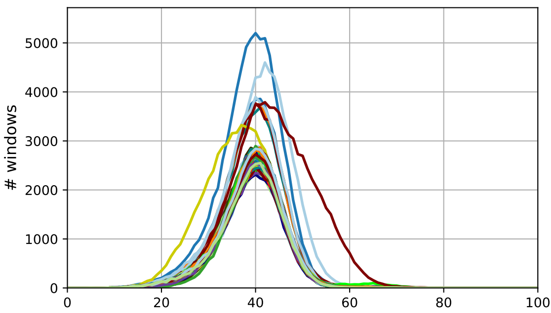
GC content
