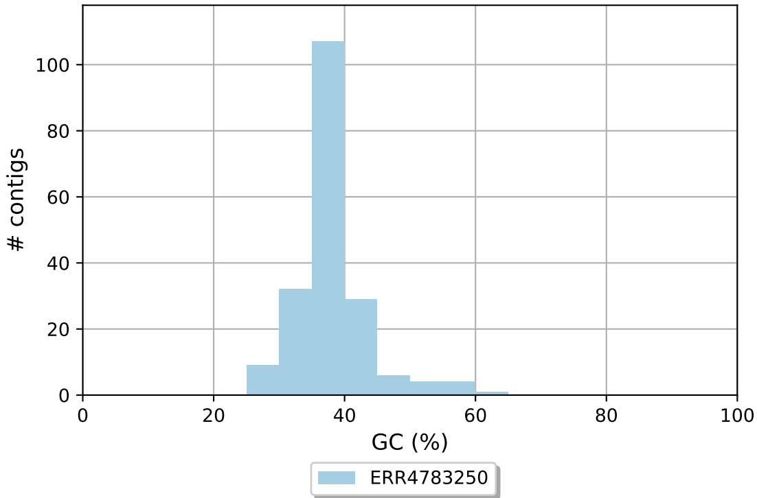
ERR4783250 GC content
