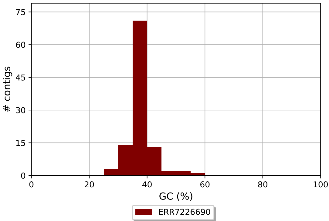
ERR7226690 GC content
