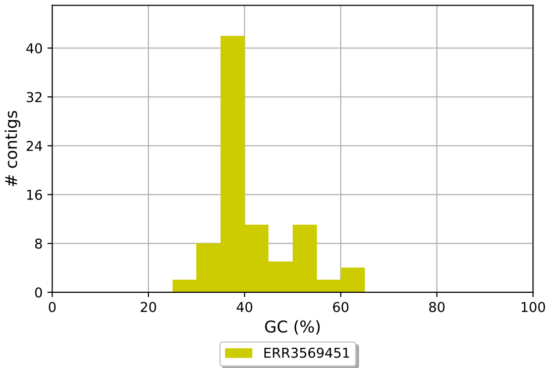
ERR3569451 GC content
