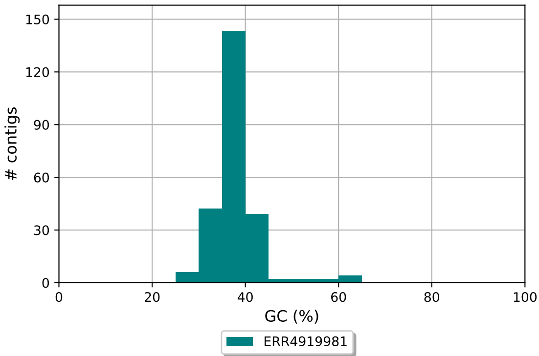
ERR4919981 GC content
