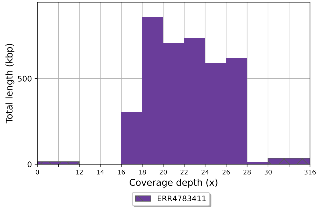
ERR4783411 coverage histogram (bin size: 2x)
