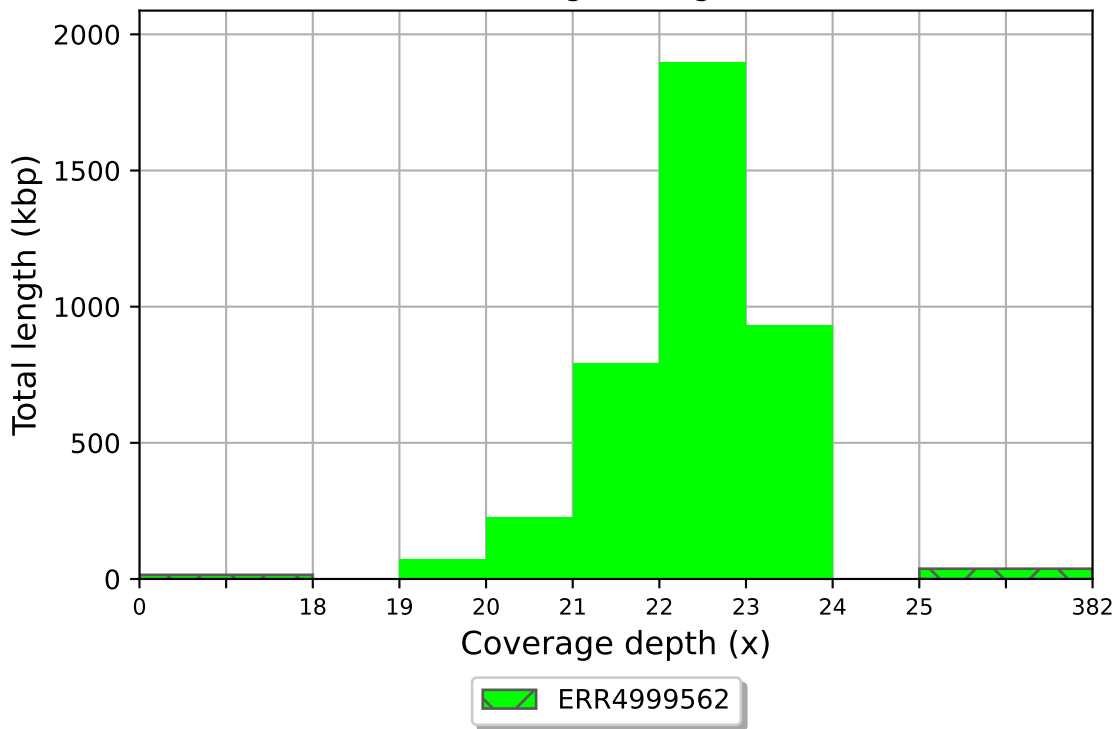
ERR4999562 coverage histogram (bin size: 1x)
