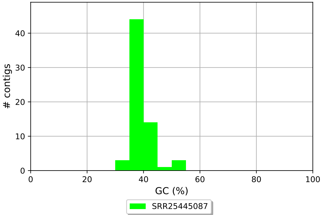
SRR25445087 GC content
