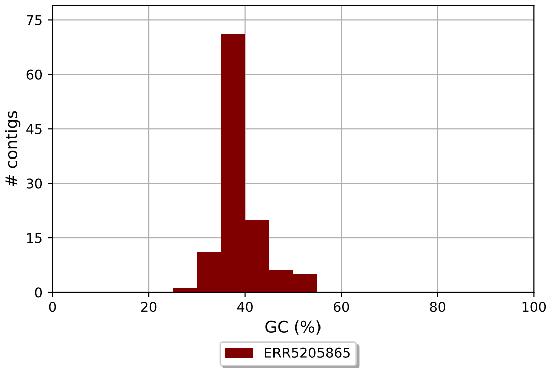
ERR5205865 GC content
