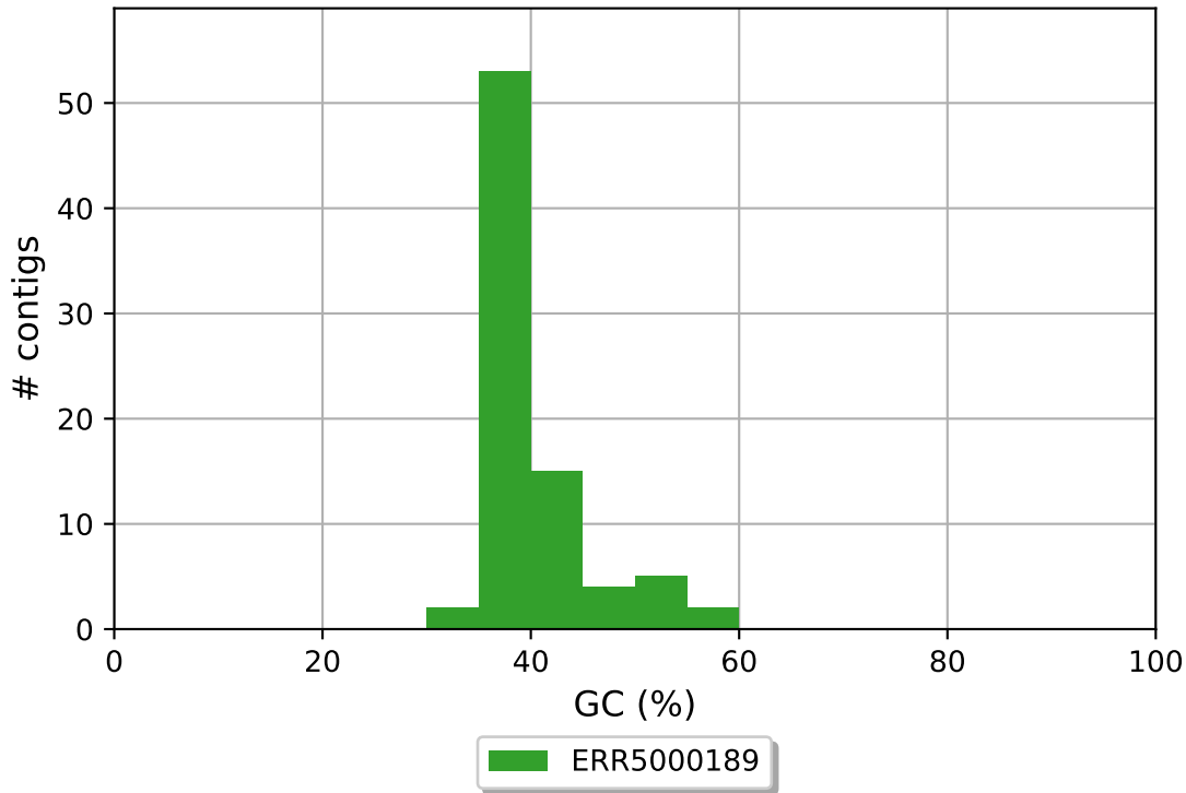
ERR5000189 GC content
