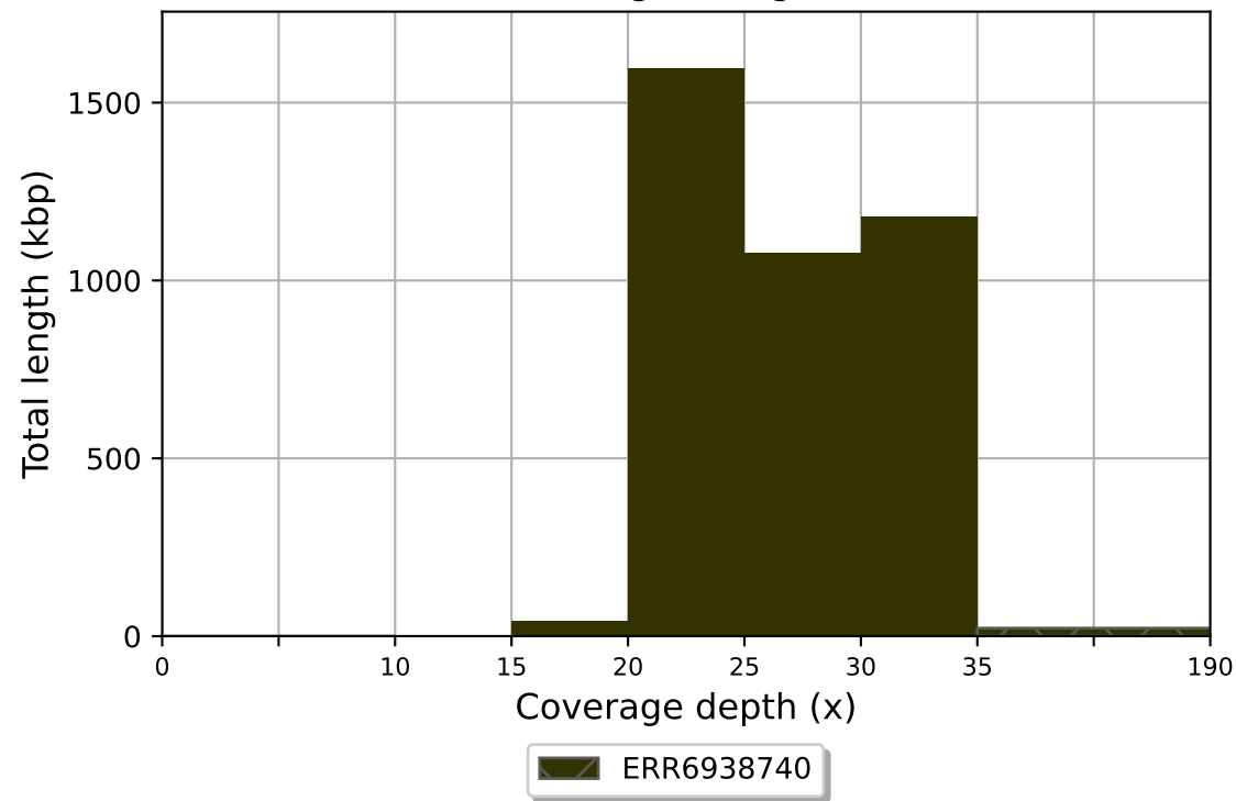
ERR6938740 coverage histogram (bin size: 5x)
