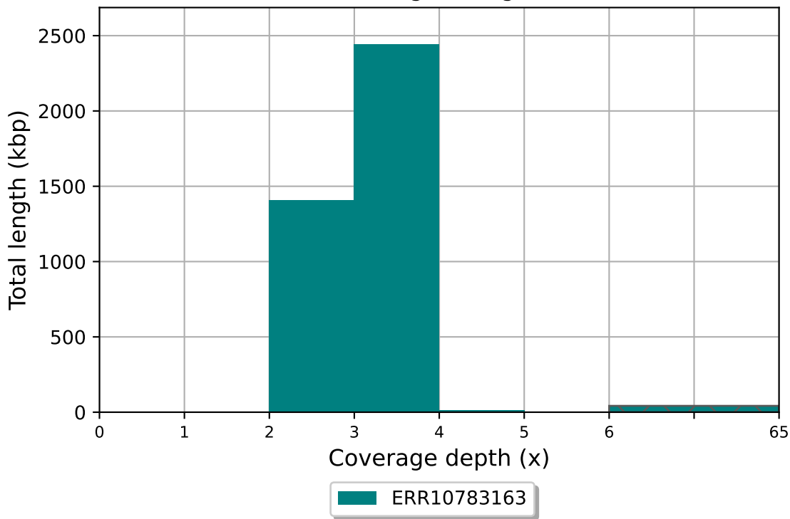
ERR10783163 coverage histogram (bin size: 1x)
