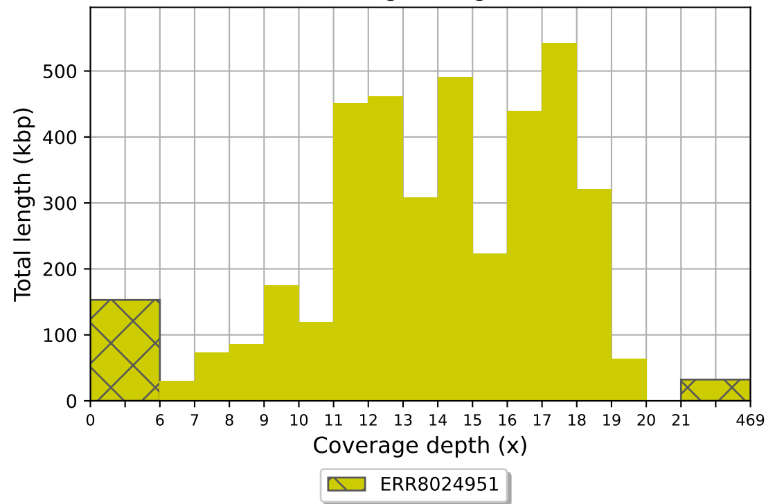
ERR8024951 coverage histogram (bin size: 1x)
