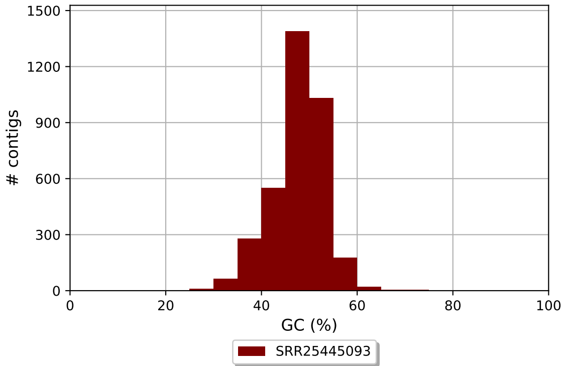
SRR25445093 GC content
