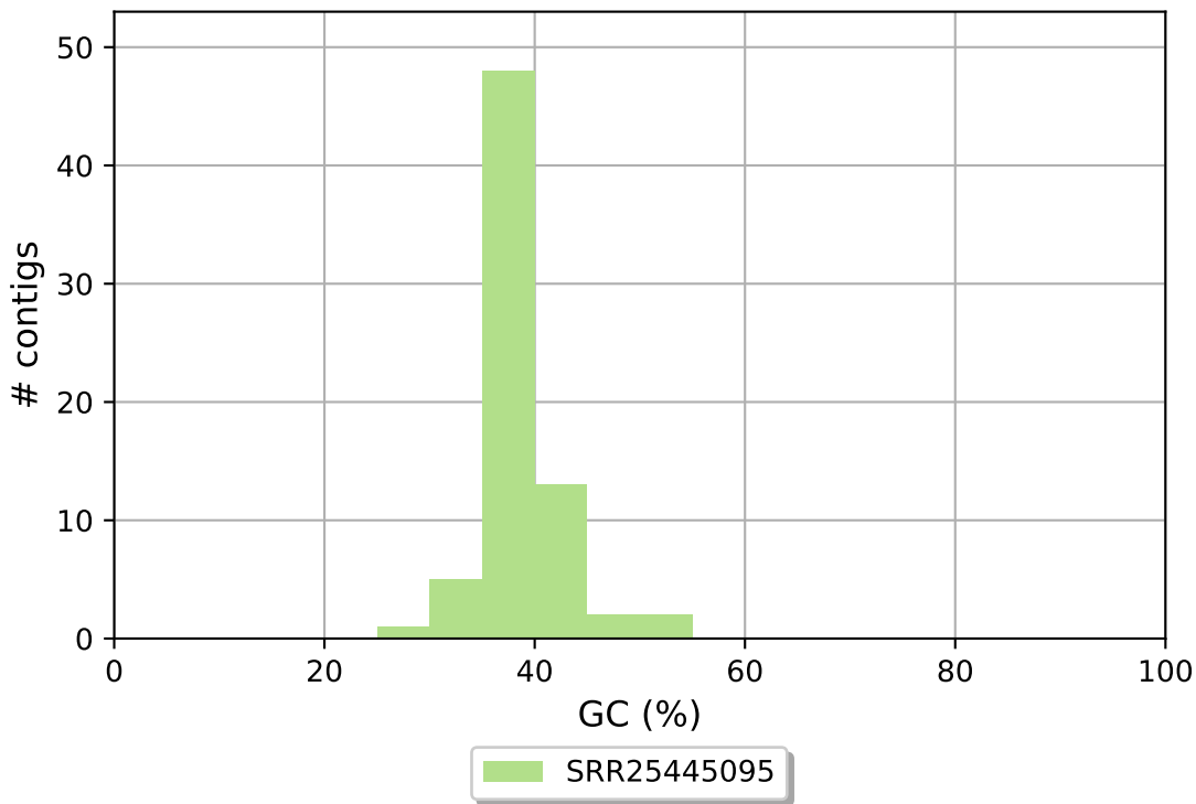
SRR25445095 GC content
