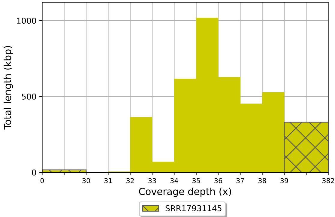
SRR17931145 coverage histogram (bin size: 1x)
