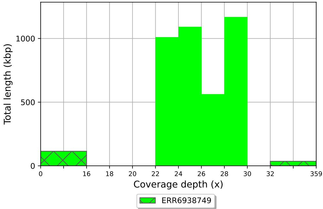
ERR6938749 coverage histogram (bin size: 2x)
