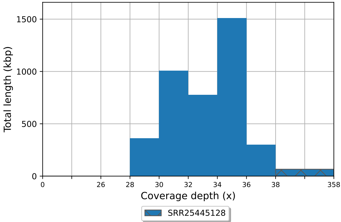
SRR25445128 coverage histogram (bin size: 2x)
