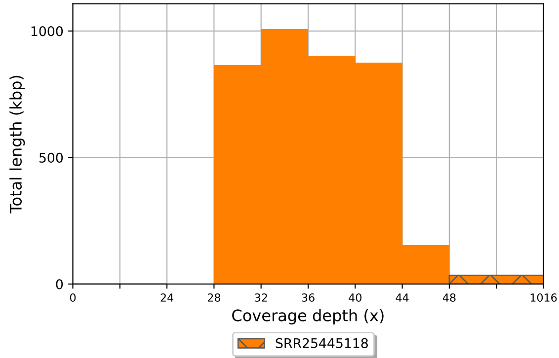
SRR25445118 coverage histogram (bin size: 4x)
