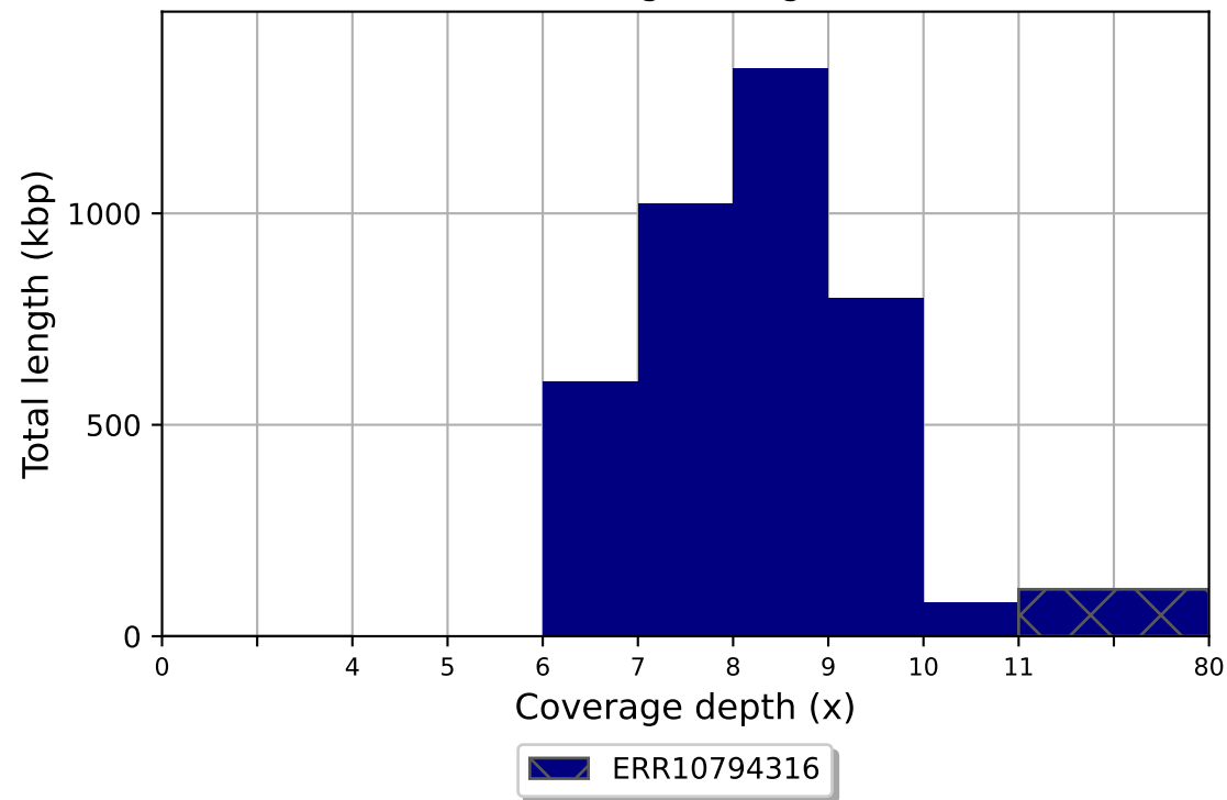
ERR10794316 coverage histogram (bin size: 1x)
