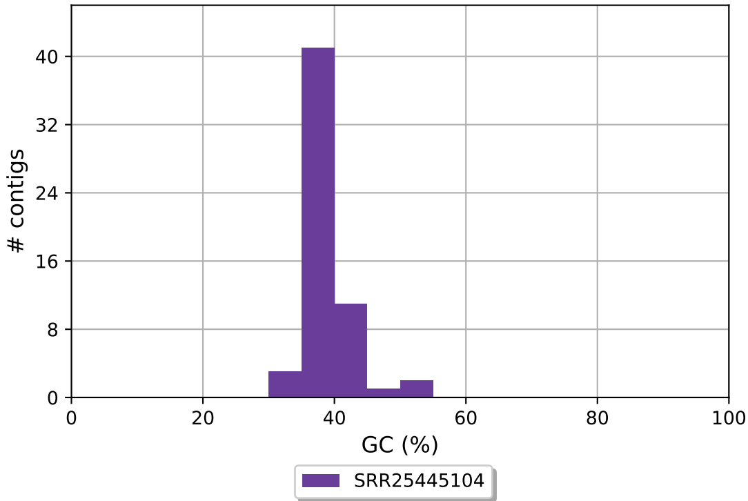
SRR25445104 GC content
