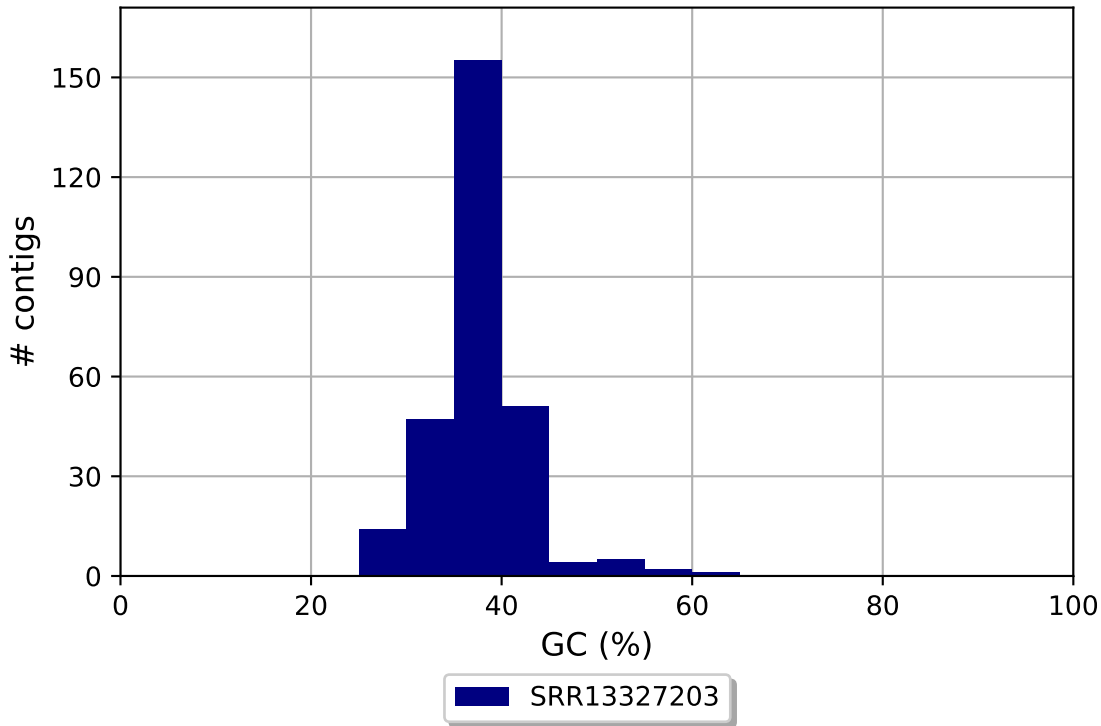
SRR13327203 GC content
