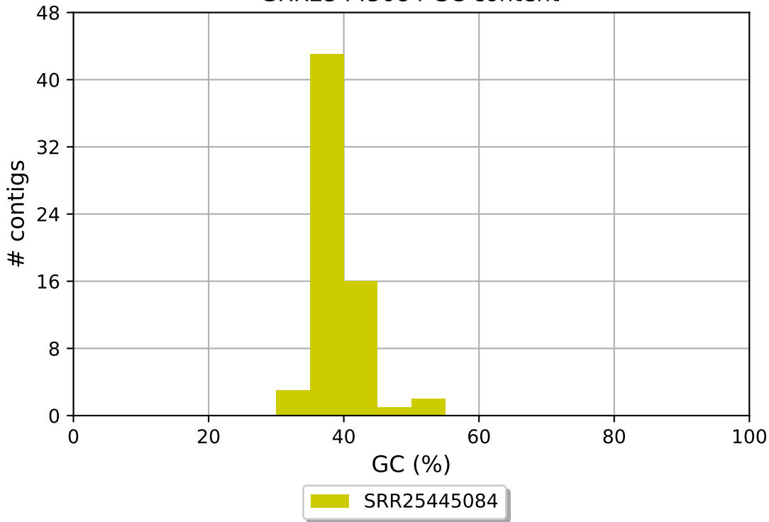
SRR25445084 GC content
