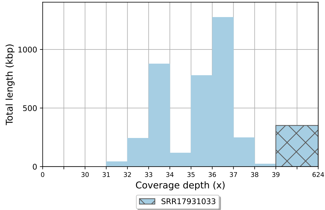
SRR17931033 coverage histogram (bin size: 1x)
