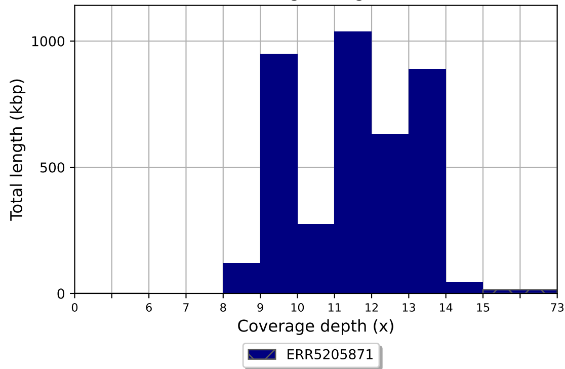
ERR5205871 coverage histogram (bin size: 1x)
