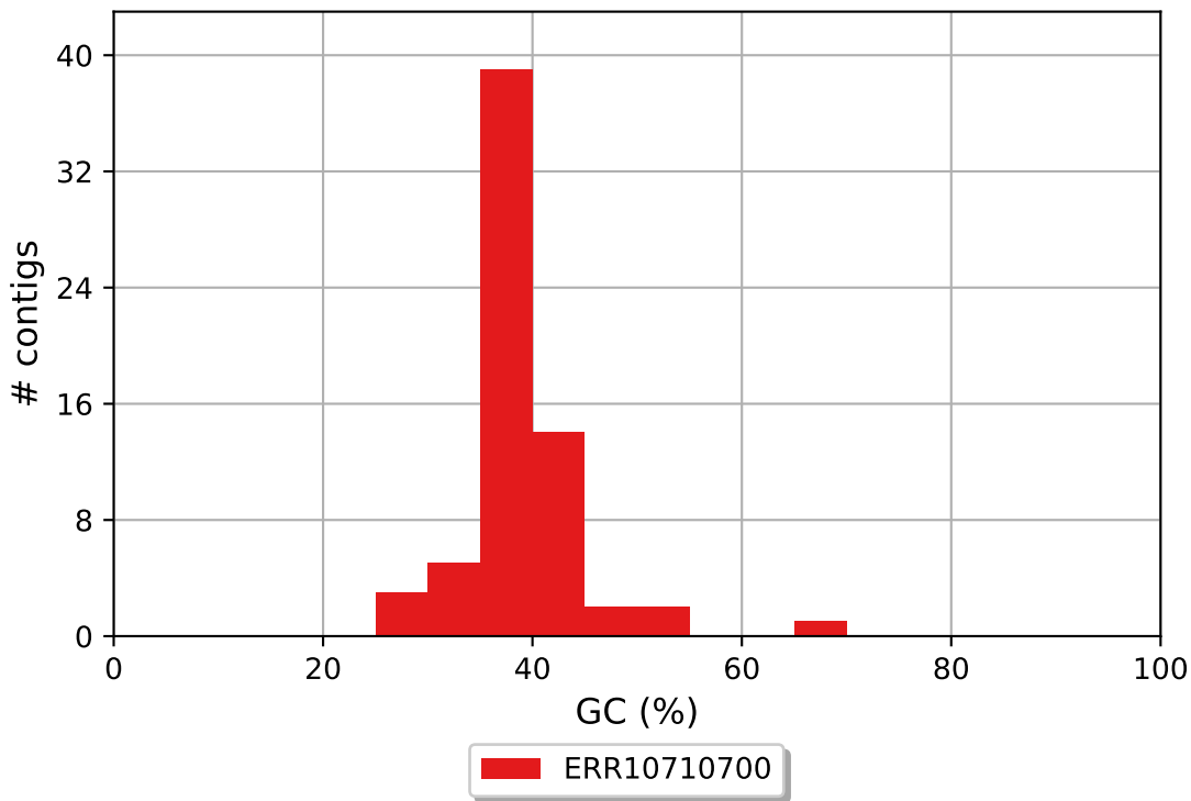
ERR10710700 GC content
