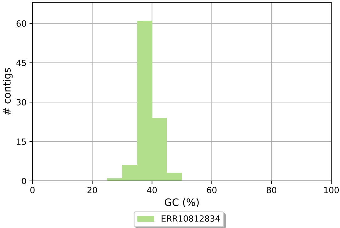
ERR10812834 GC content
