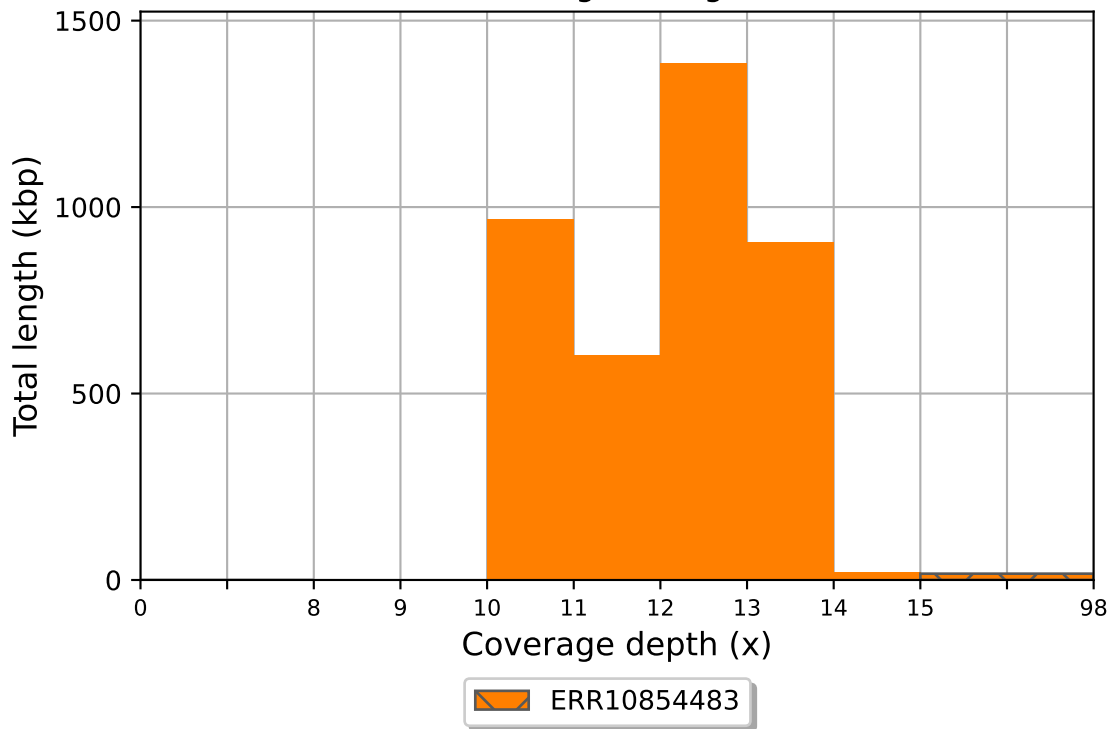
ERR10854483 coverage histogram (bin size: 1x)
