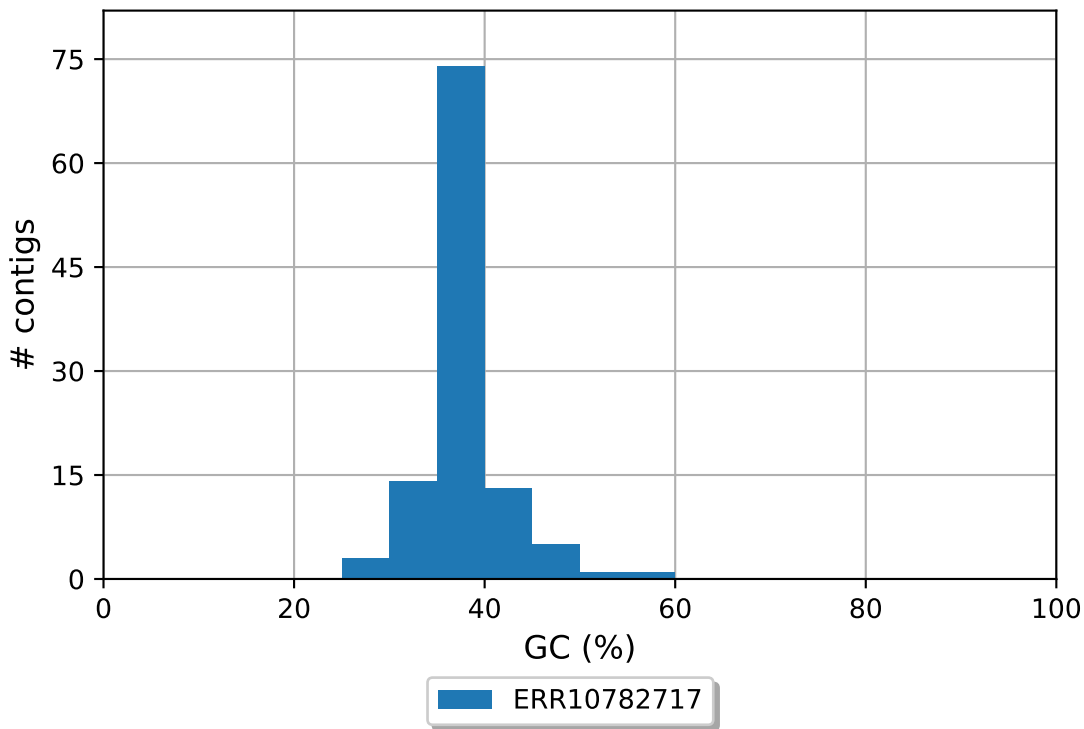
ERR10782717 GC content
