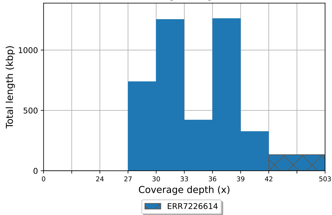
ERR7226614 coverage histogram (bin size: 3x)
