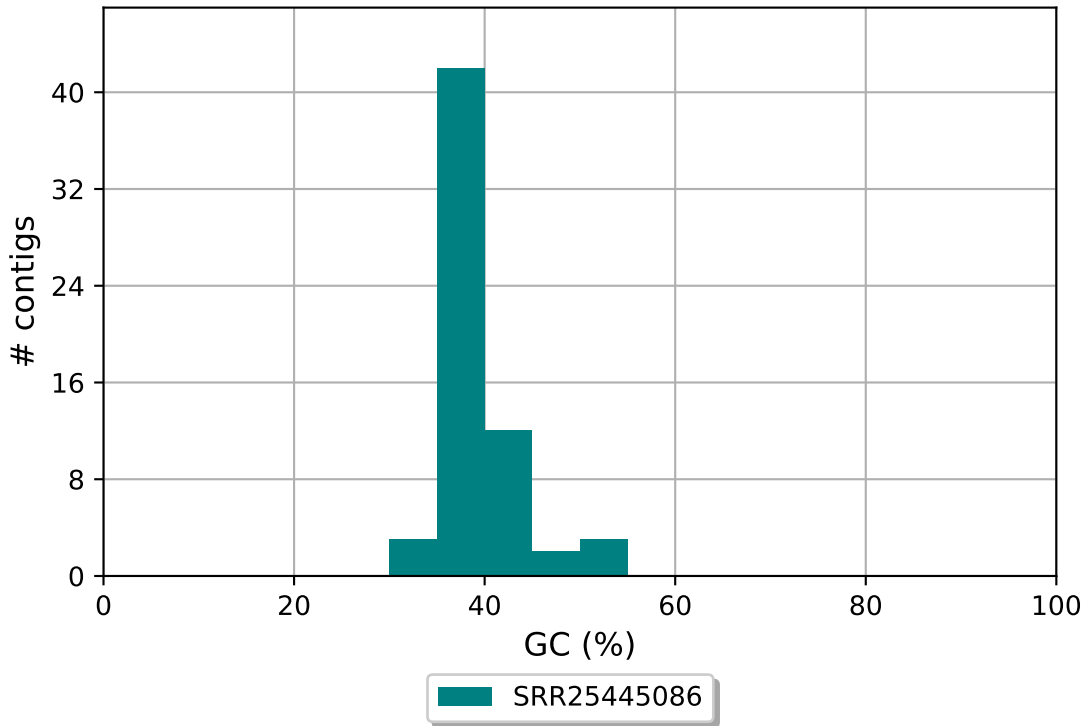
SRR25445086 GC content
