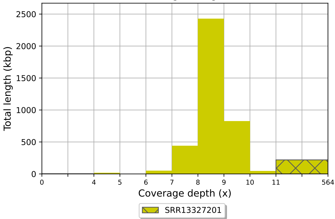
SRR13327201 coverage histogram (bin size: 1x)
