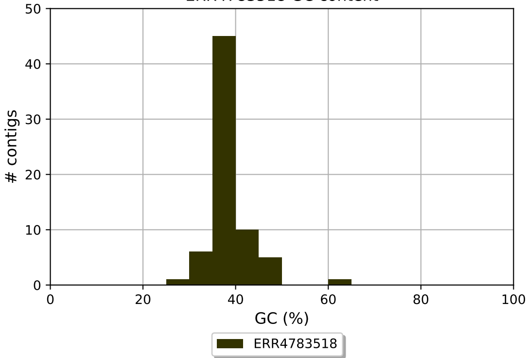
ERR4783518 GC content
