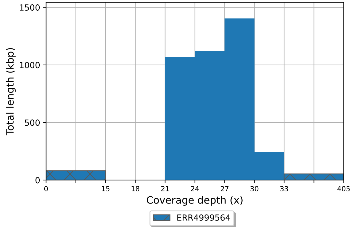
ERR4999564 coverage histogram (bin size: 3x)
