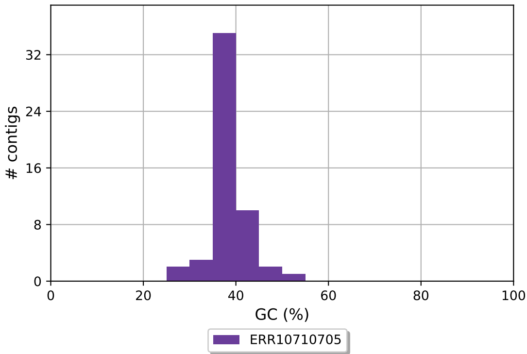
ERR10710705 GC content
