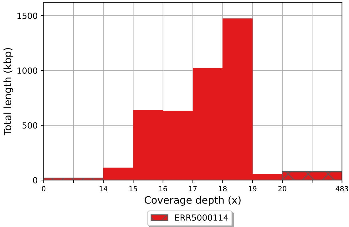
ERR5000114 coverage histogram (bin size: 1x)
