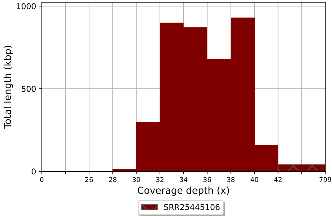
SRR25445106 coverage histogram (bin size: 2x)
