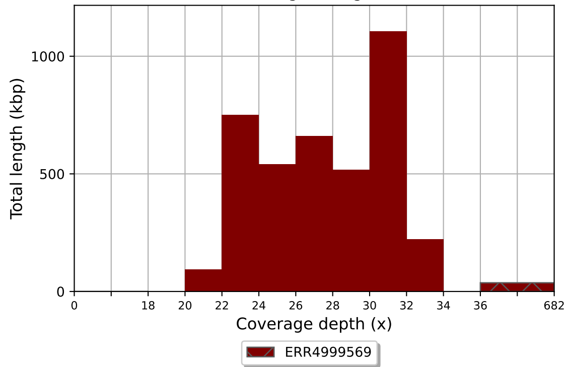
ERR4999569 coverage histogram (bin size: 2x)
