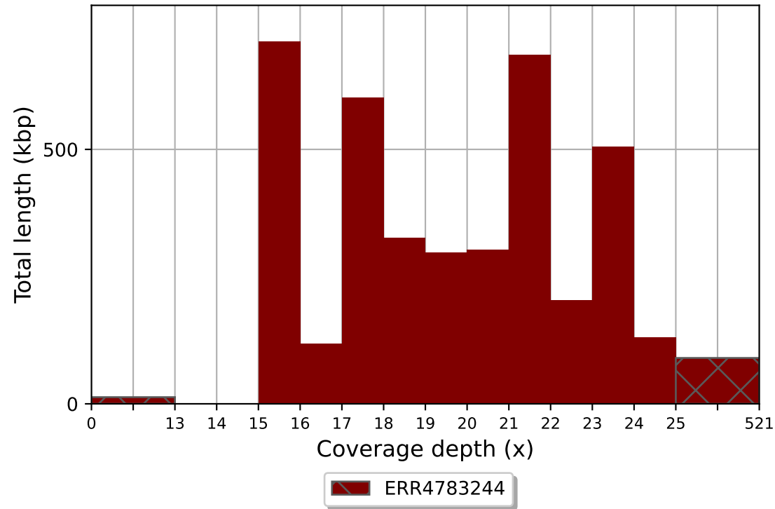
ERR4783244 coverage histogram (bin size: 1x)
