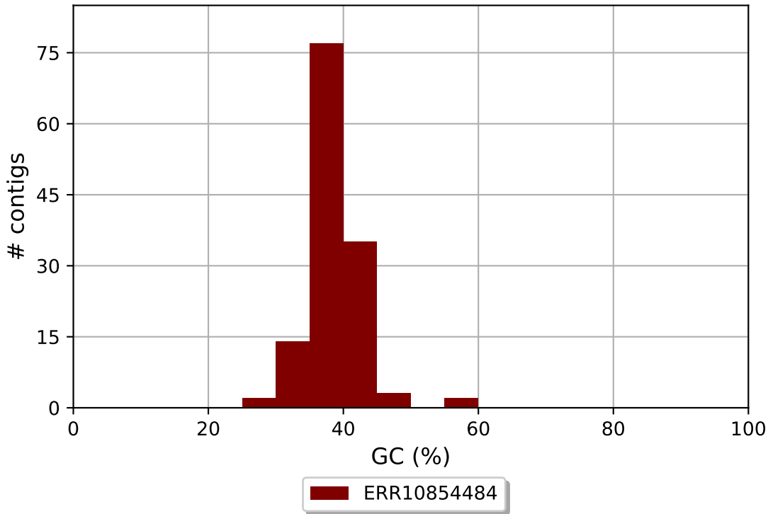
ERR10854484 GC content
