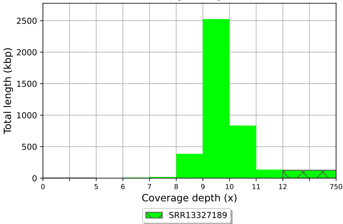
SRR13327189 coverage histogram (bin size: 1x)
