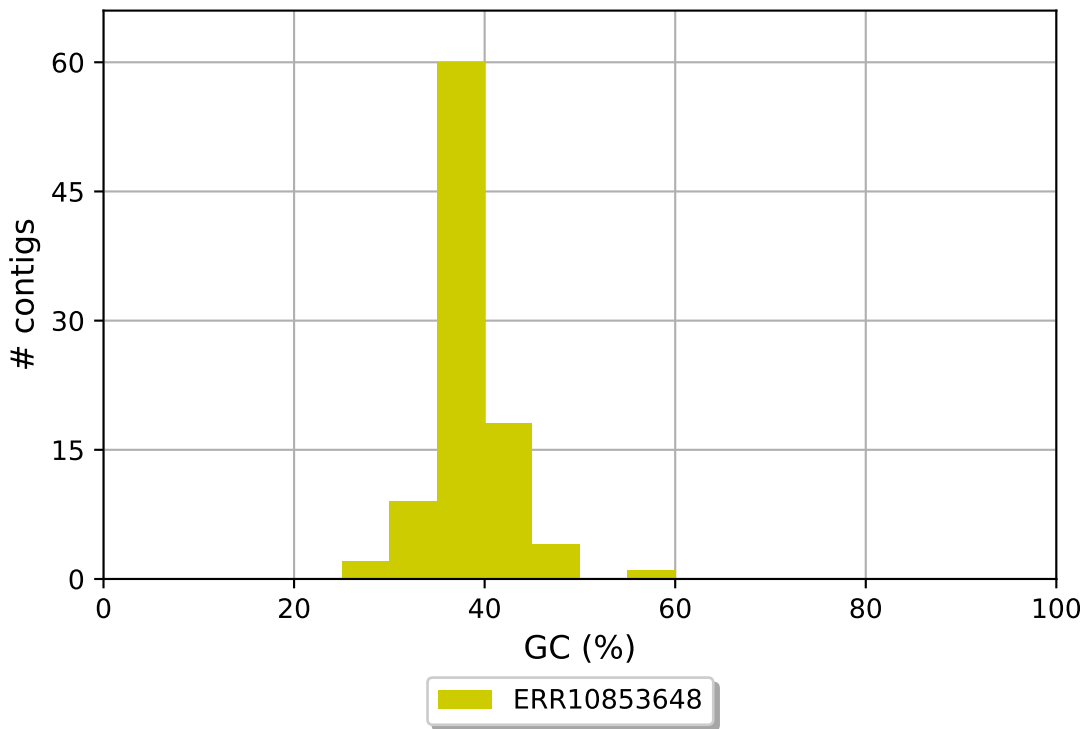
ERR10853648 GC content
