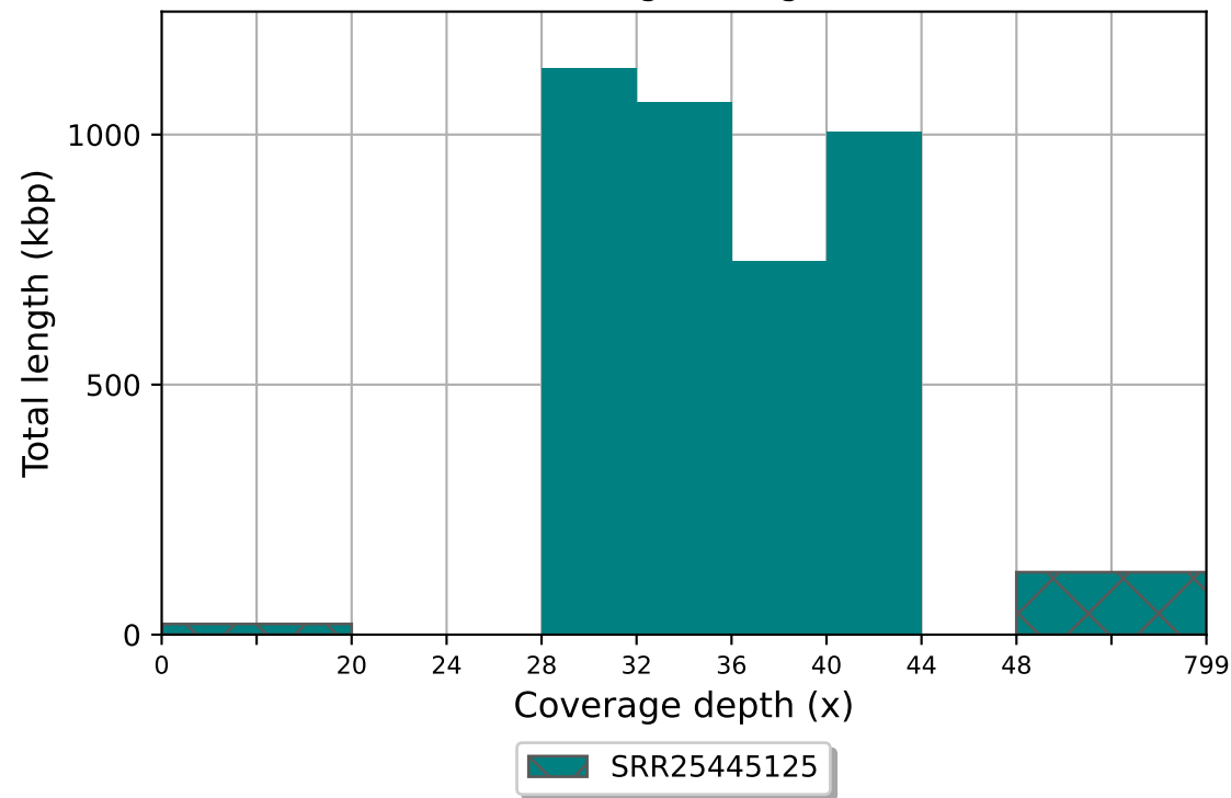
SRR25445125 coverage histogram (bin size: 4x)
