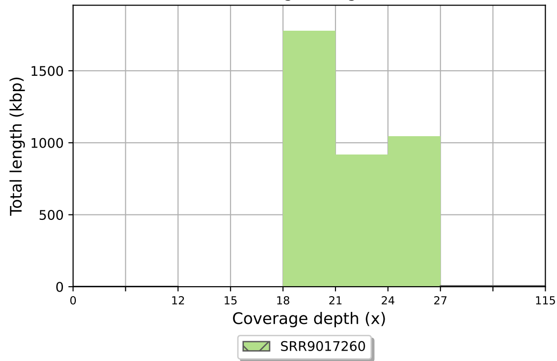
SRR9017260 coverage histogram (bin size: 3x)
