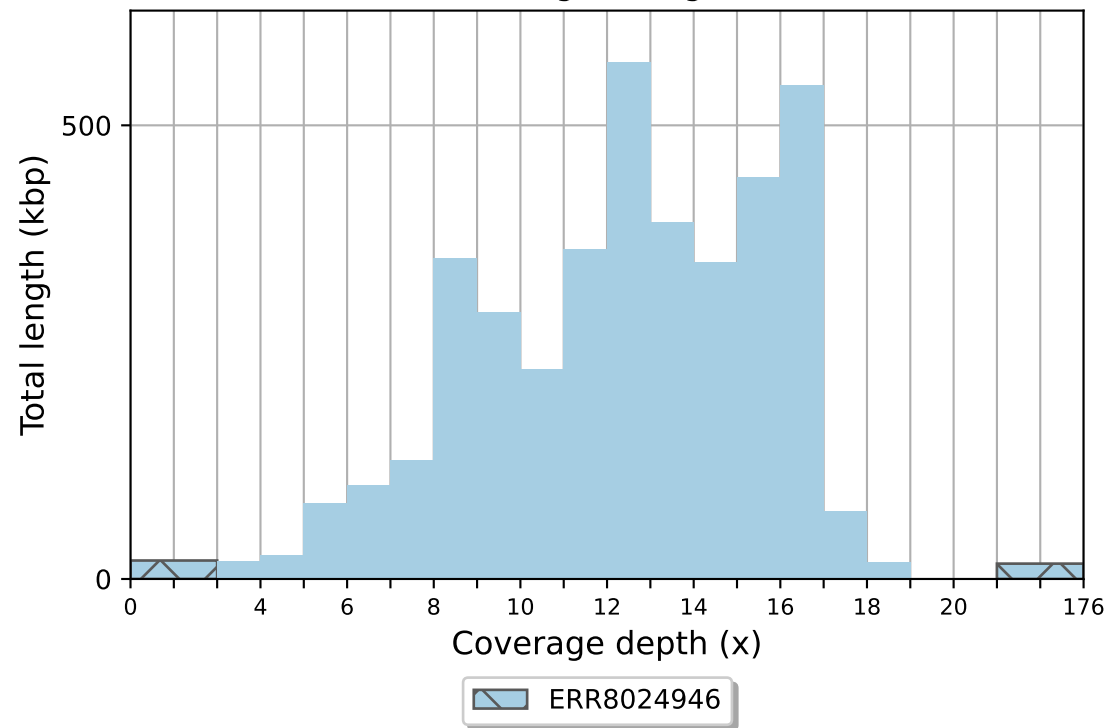
ERR8024946 coverage histogram (bin size: 1x)
