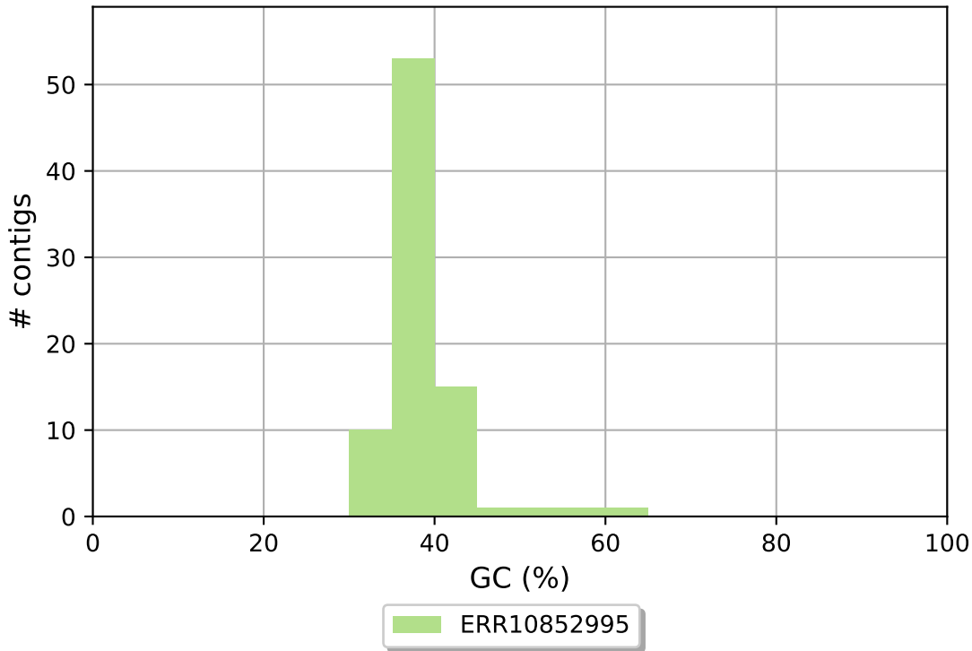
ERR10852995 GC content
