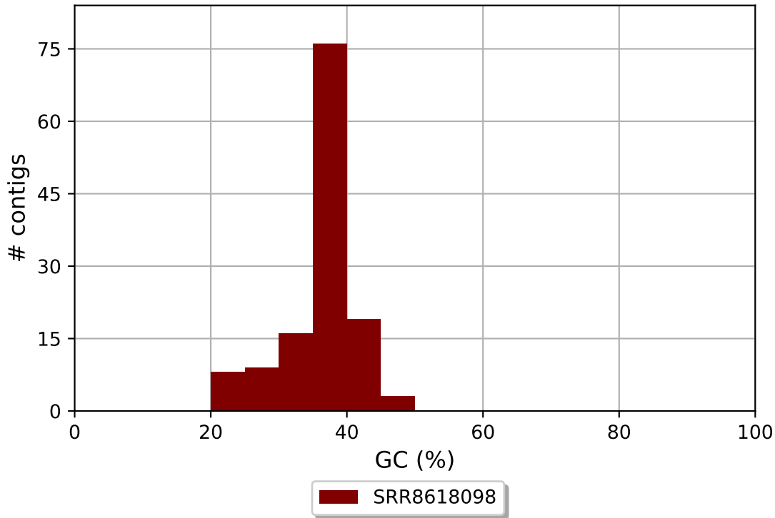
SRR8618098 GC content
