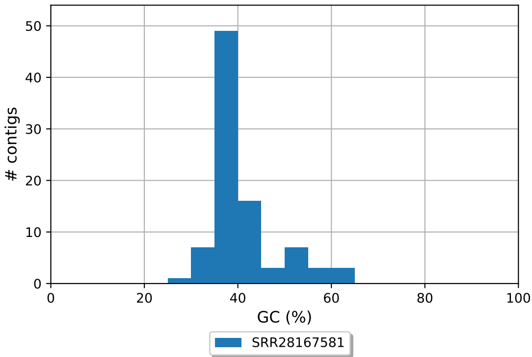
SRR28167581 GC content
