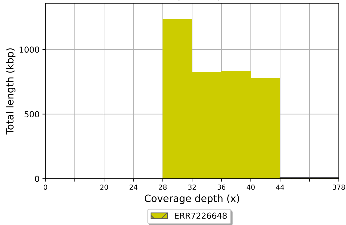
ERR7226648 coverage histogram (bin size: 4x)
