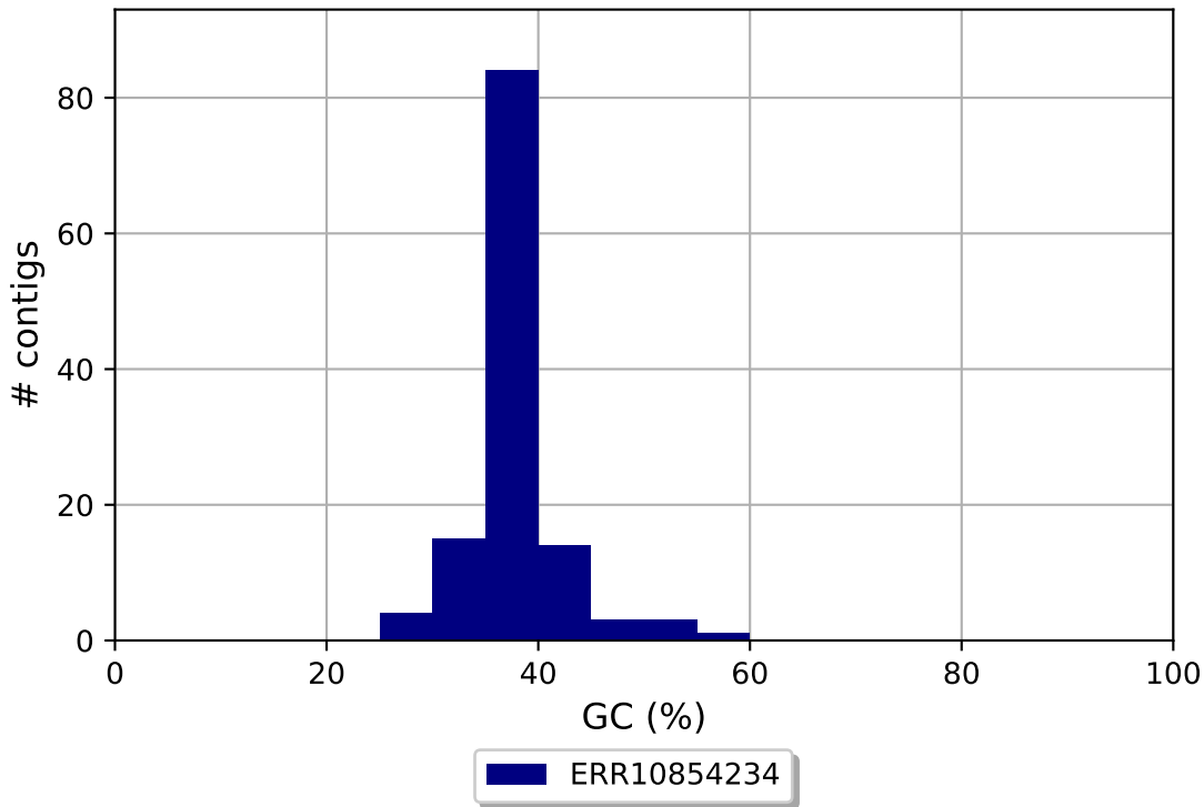
ERR10854234 GC content
