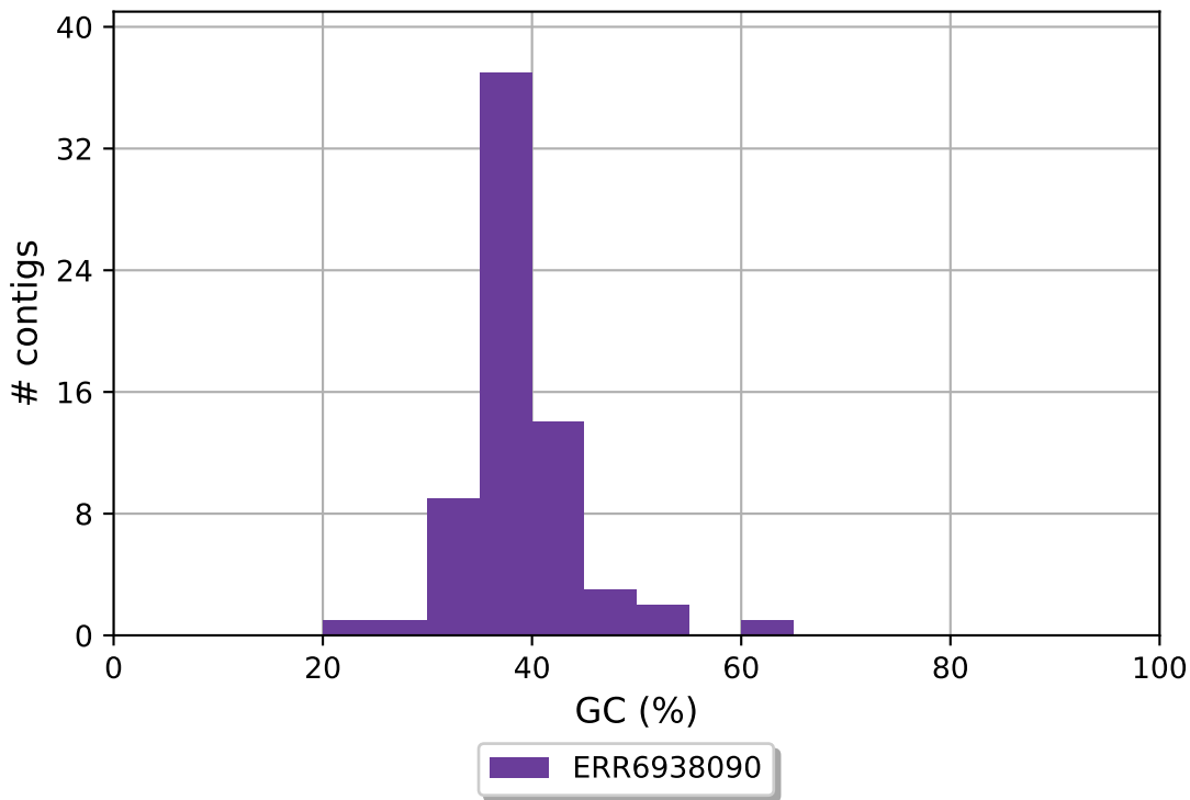
ERR6938090 GC content
