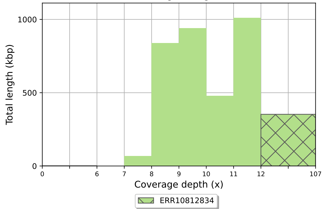
ERR10812834 coverage histogram (bin size: 1x)
