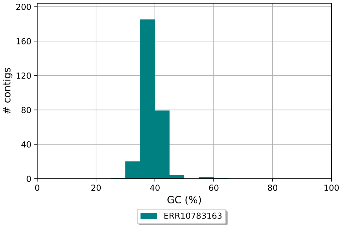
ERR10783163 GC content
