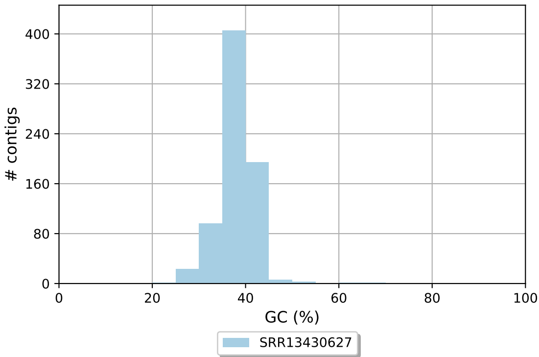
SRR13430627 GC content
