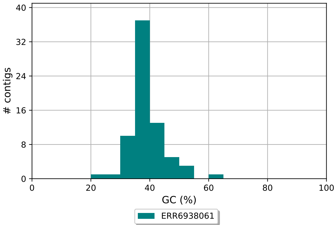
ERR6938061 GC content
