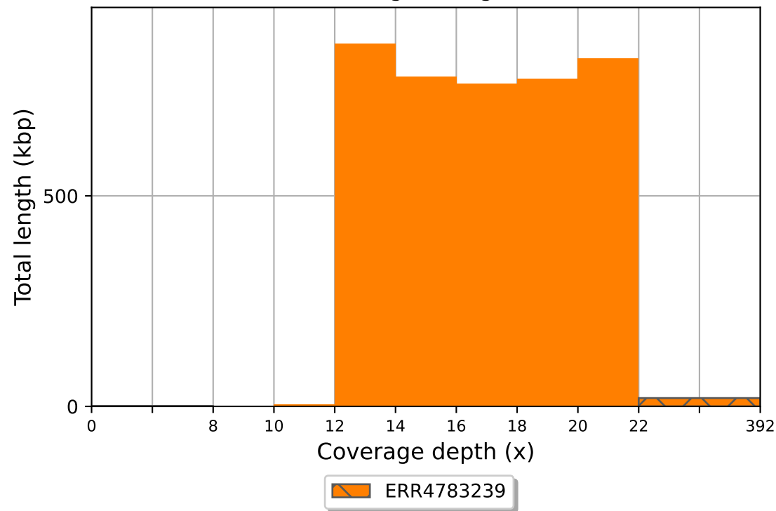
ERR4783239 coverage histogram (bin size: 2x)
