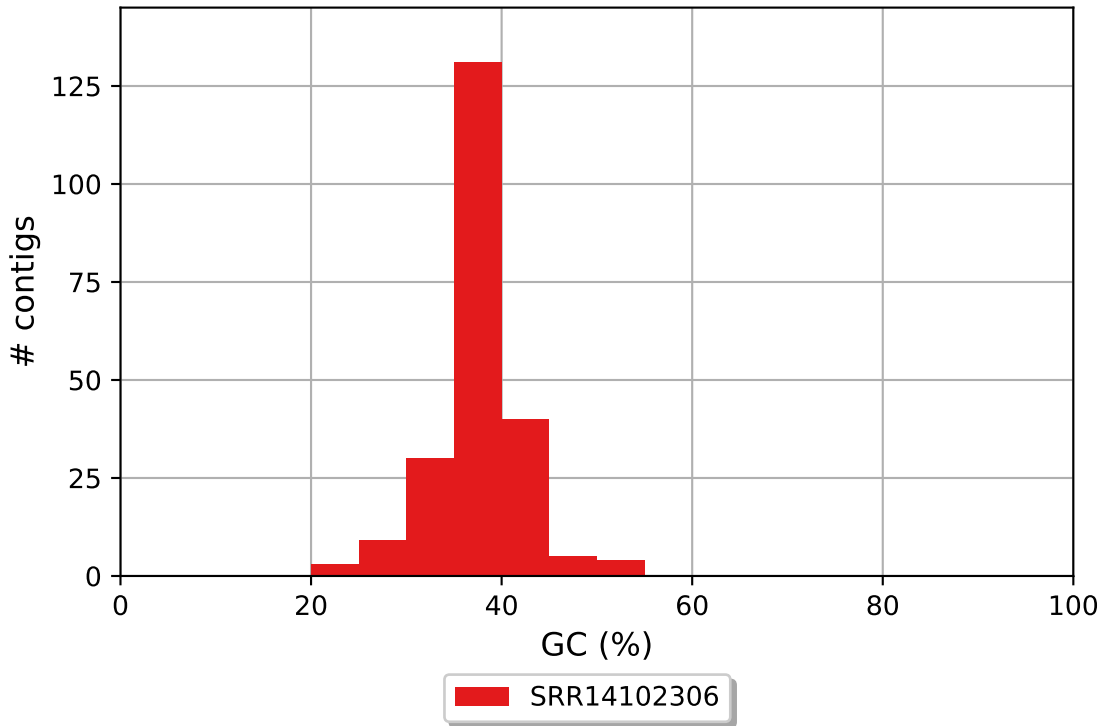
SRR14102306 GC content
