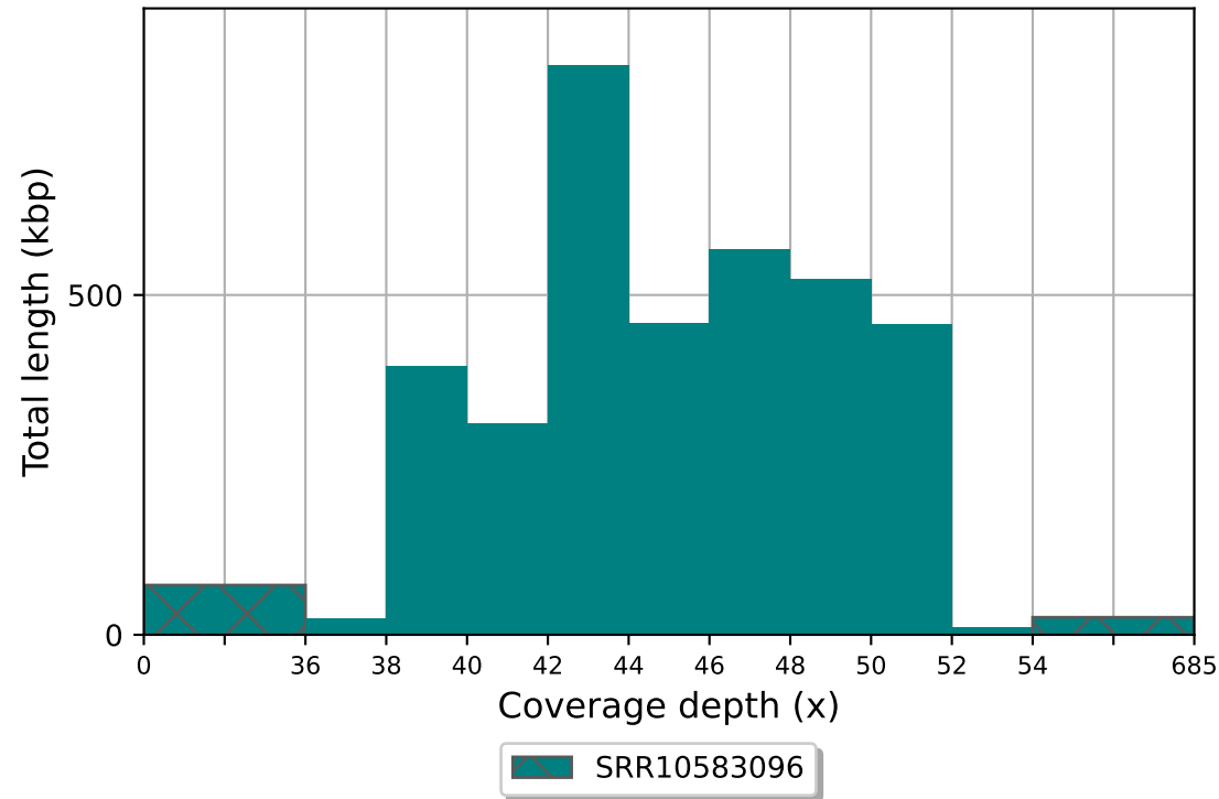
SRR10583096 coverage histogram (bin size: 2x)
