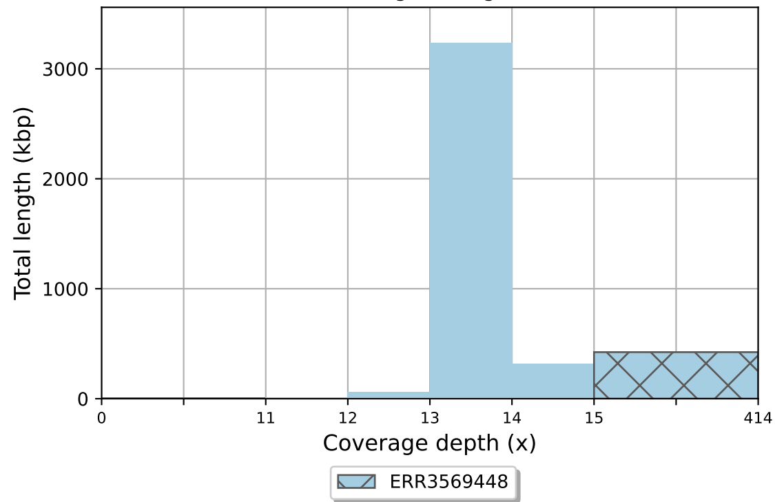
ERR3569448 coverage histogram (bin size: 1x)
