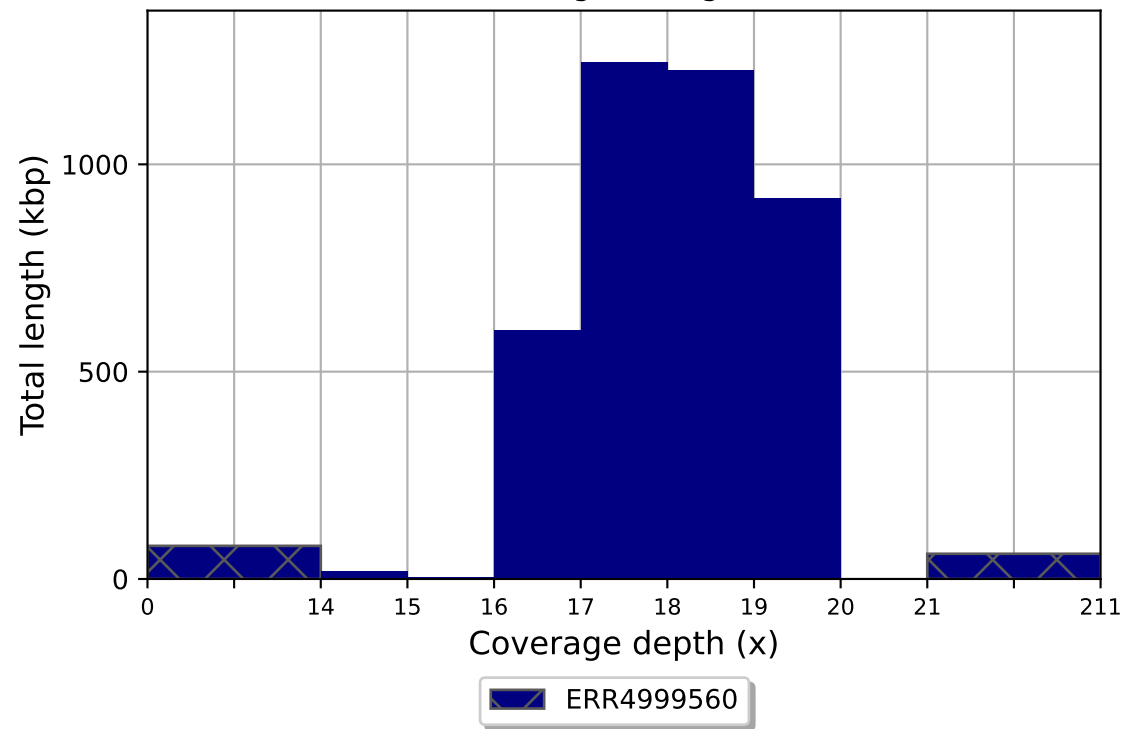
ERR4999560 coverage histogram (bin size: 1x)
