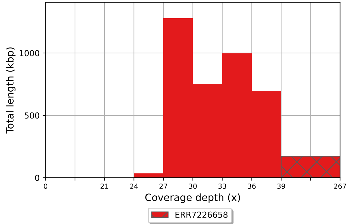
ERR7226658 coverage histogram (bin size: 3x)
