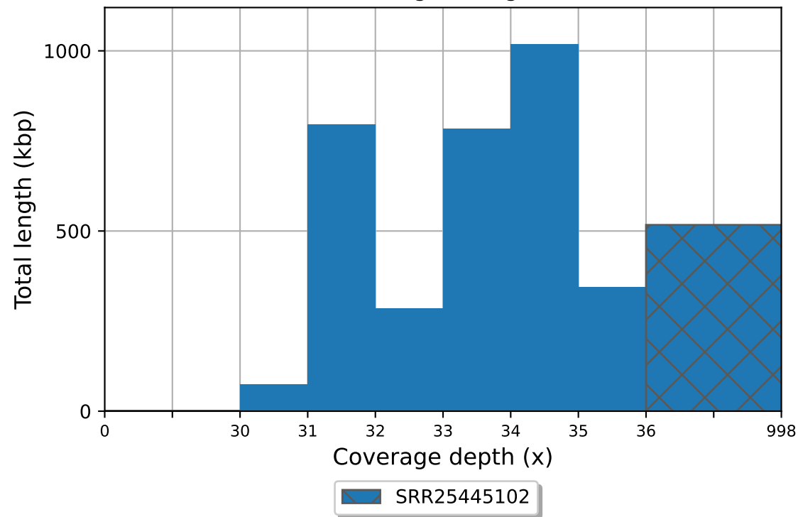
SRR25445102 coverage histogram (bin size: 1x)
