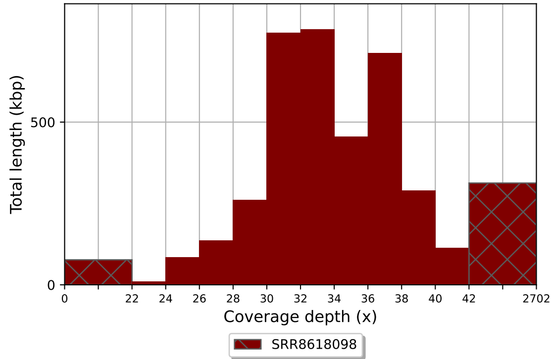
SRR8618098 coverage histogram (bin size: 2x)
