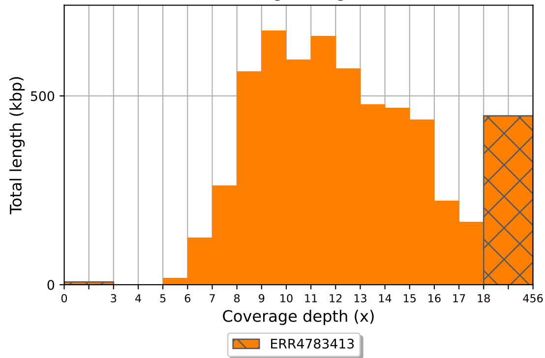
ERR4783413 coverage histogram (bin size: 1x)
