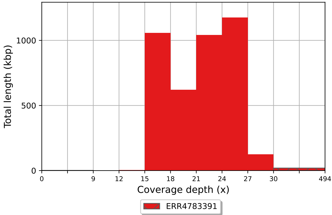
ERR4783391 coverage histogram (bin size: 3x)
