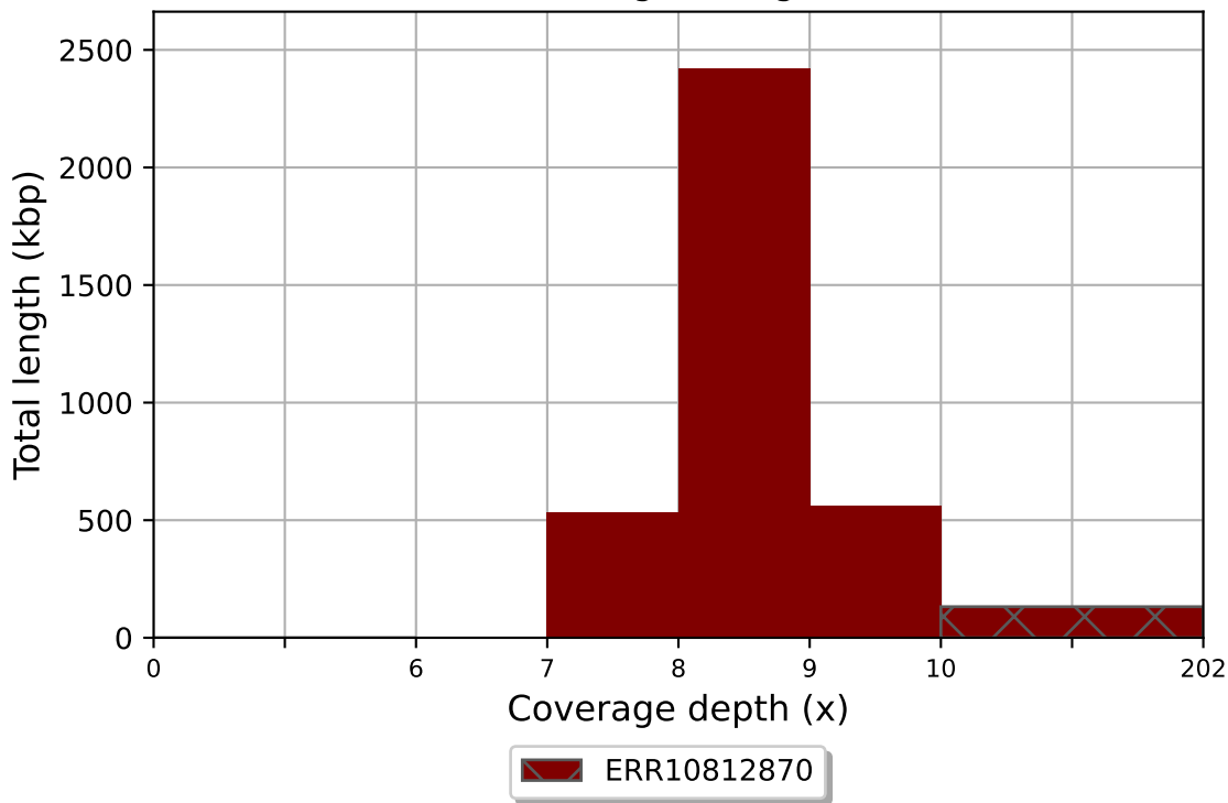
ERR10812870 coverage histogram (bin size: 1x)
