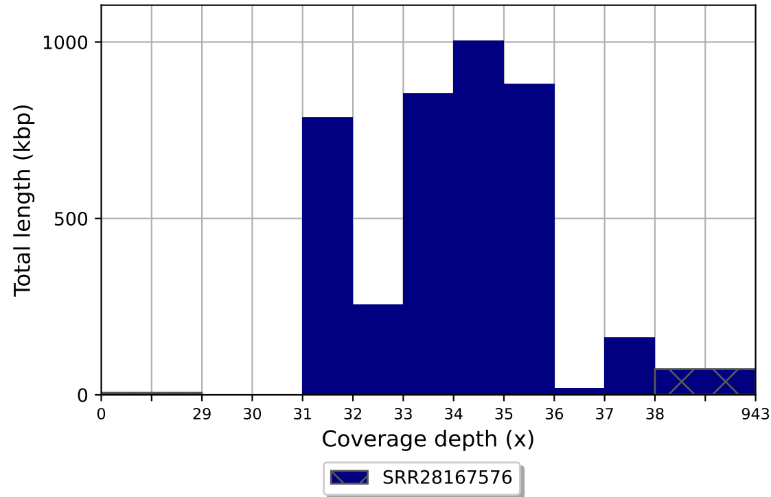
SRR28167576 coverage histogram (bin size: 1x)
