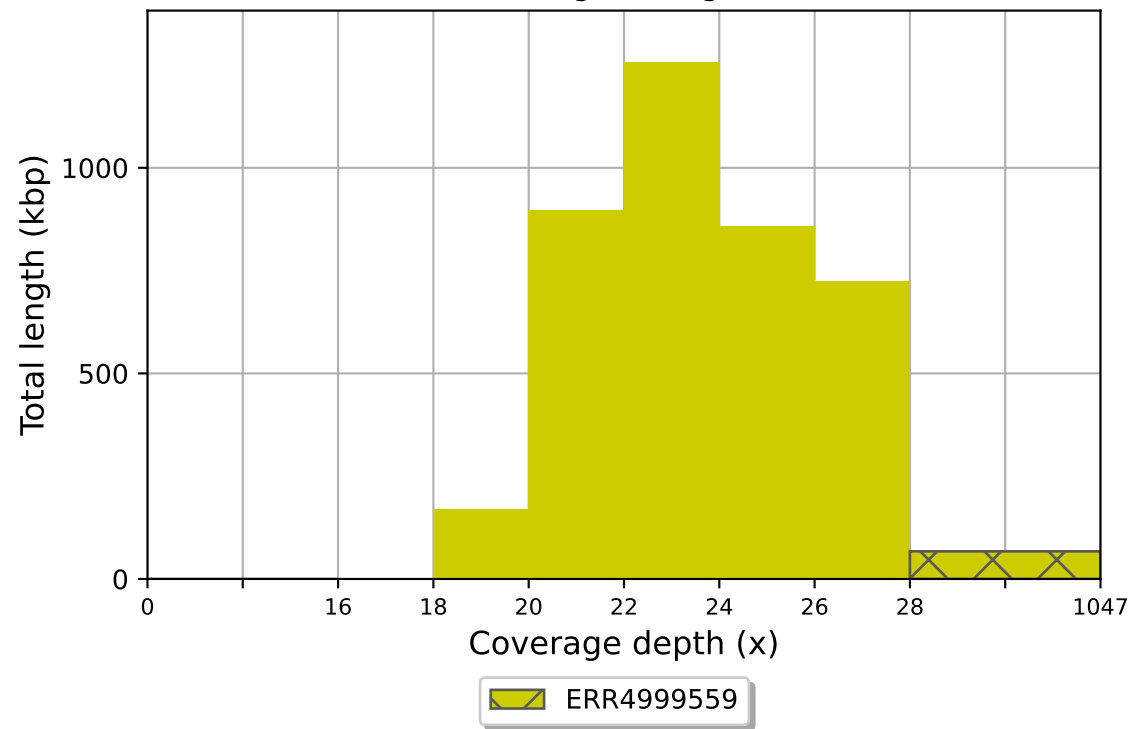
ERR4999559 coverage histogram (bin size: 2x)
