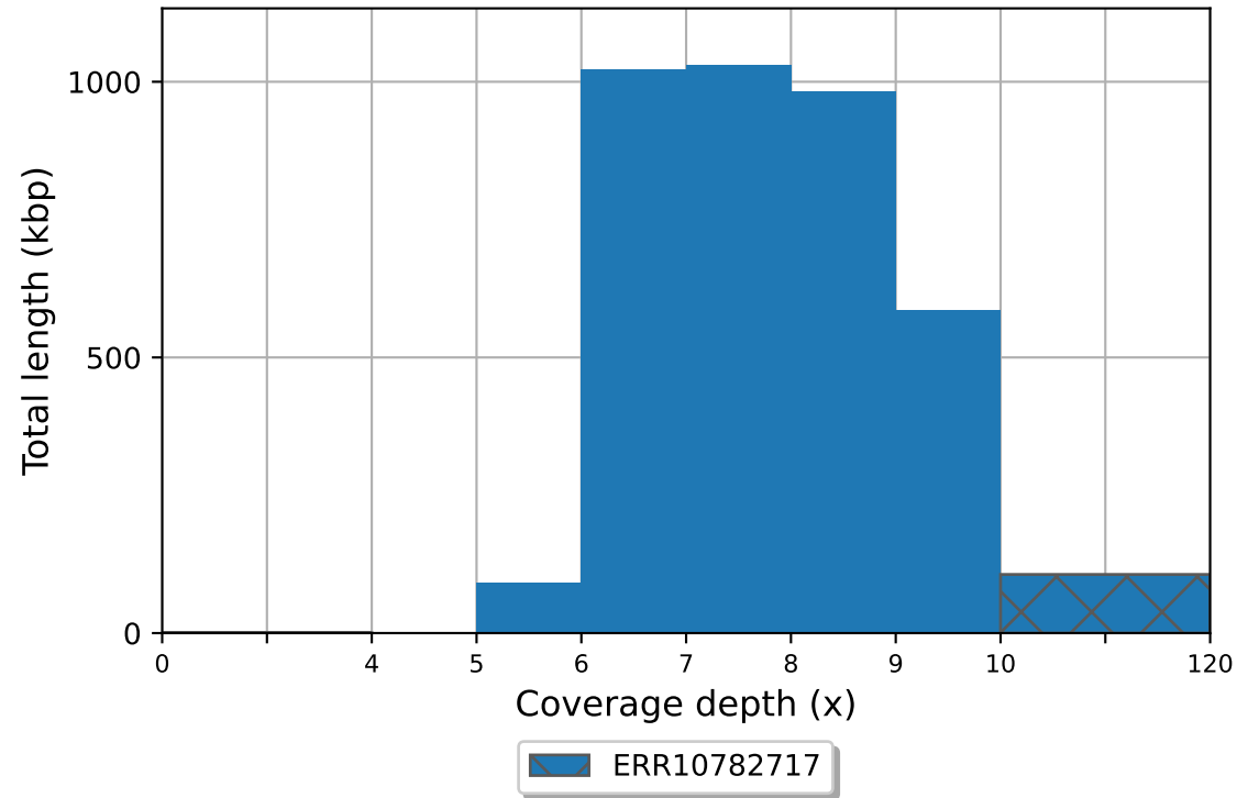
ERR10782717 coverage histogram (bin size: 1x)
