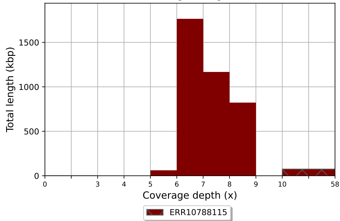
ERR10788115 coverage histogram (bin size: 1x)
