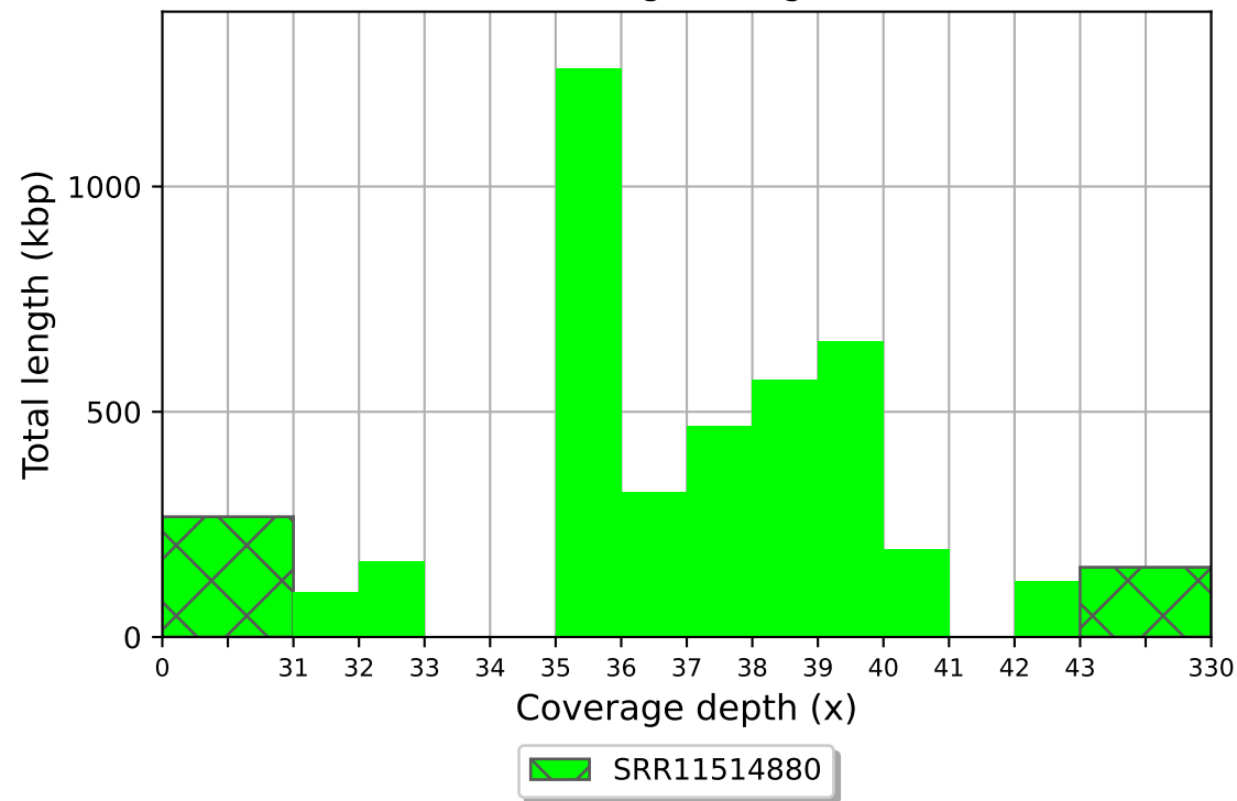
SRR11514880 coverage histogram (bin size: 1x)
