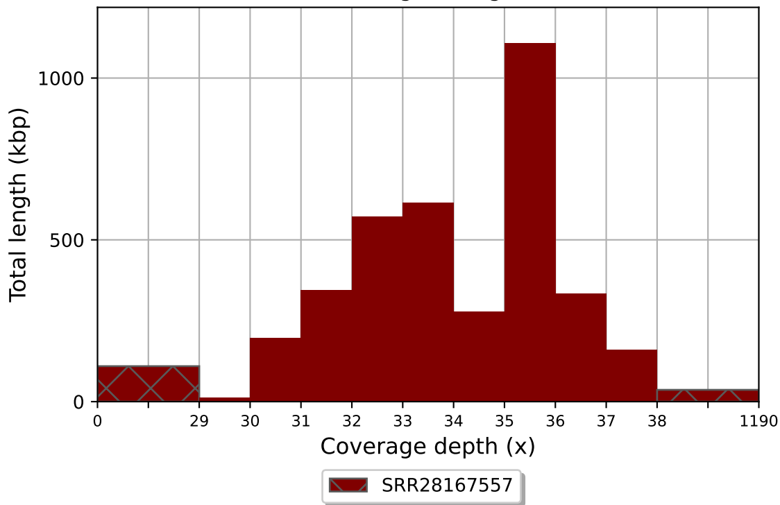
SRR28167557 coverage histogram (bin size: 1x)
