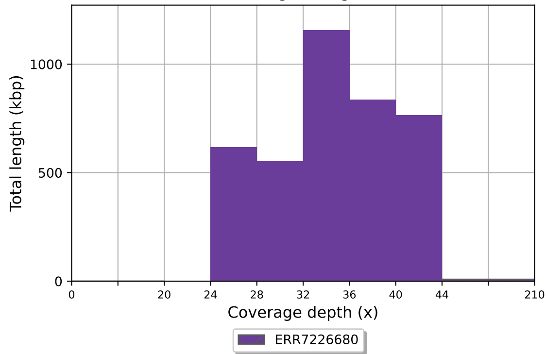
ERR7226680 coverage histogram (bin size: 4x)
