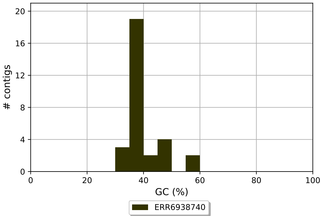
ERR6938740 GC content
