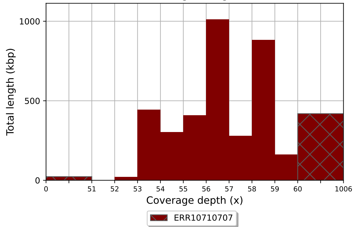
ERR10710707 coverage histogram (bin size: 1x)
