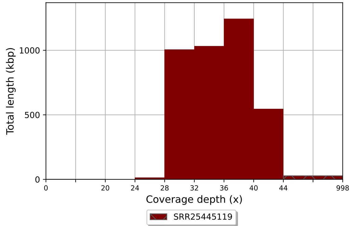
SRR25445119 coverage histogram (bin size: 4x)
