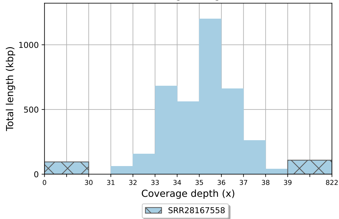
SRR28167558 coverage histogram (bin size: 1x)
