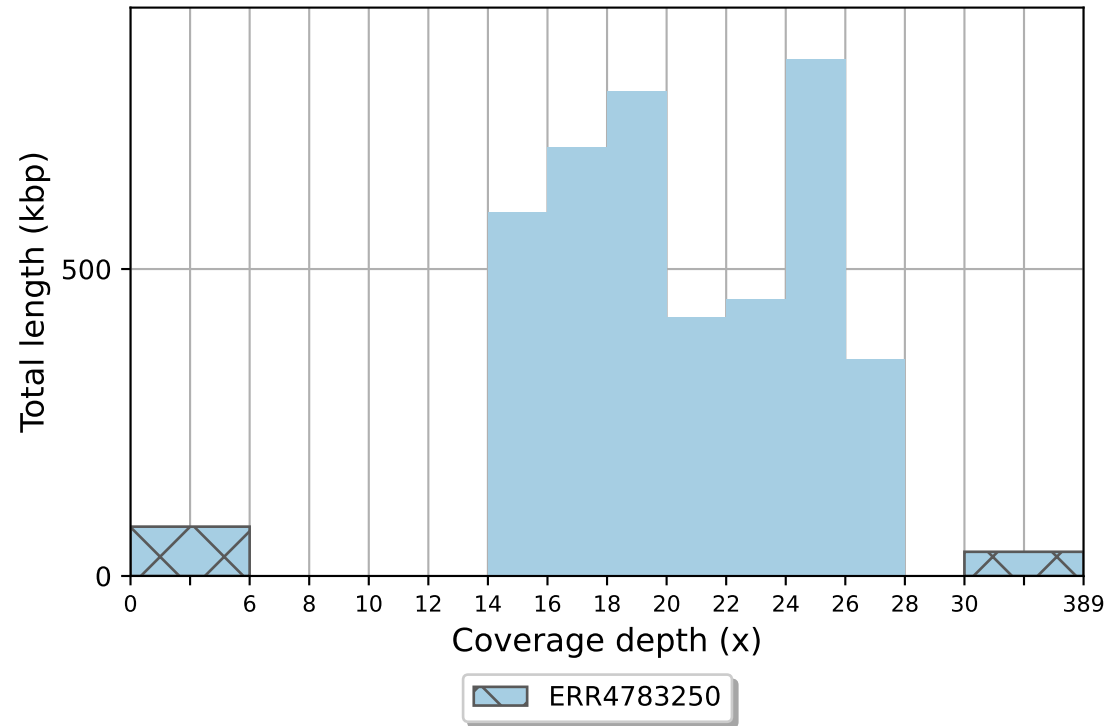
ERR4783250 coverage histogram (bin size: 2x)
