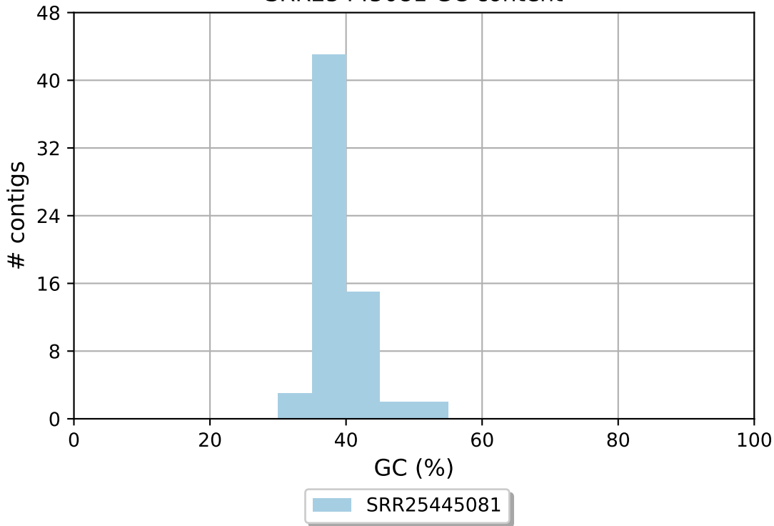
SRR25445081 GC content
