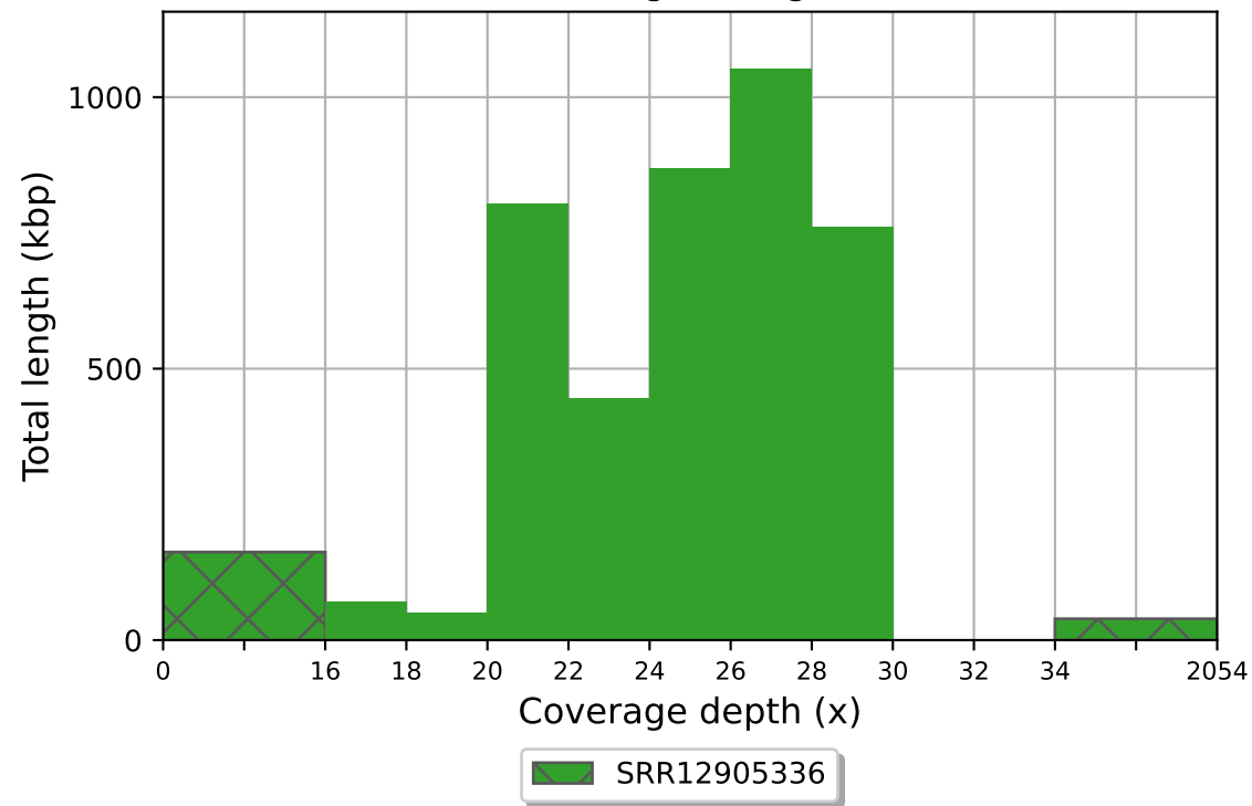
SRR12905336 coverage histogram (bin size: 2x)
