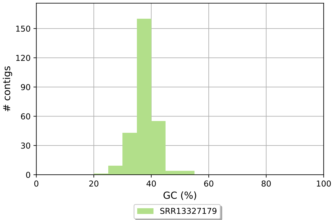
SRR13327179 GC content
