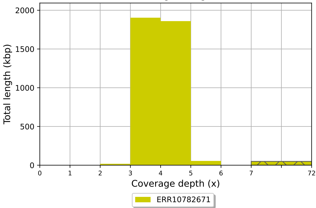
ERR10782671 coverage histogram (bin size: 1x)
