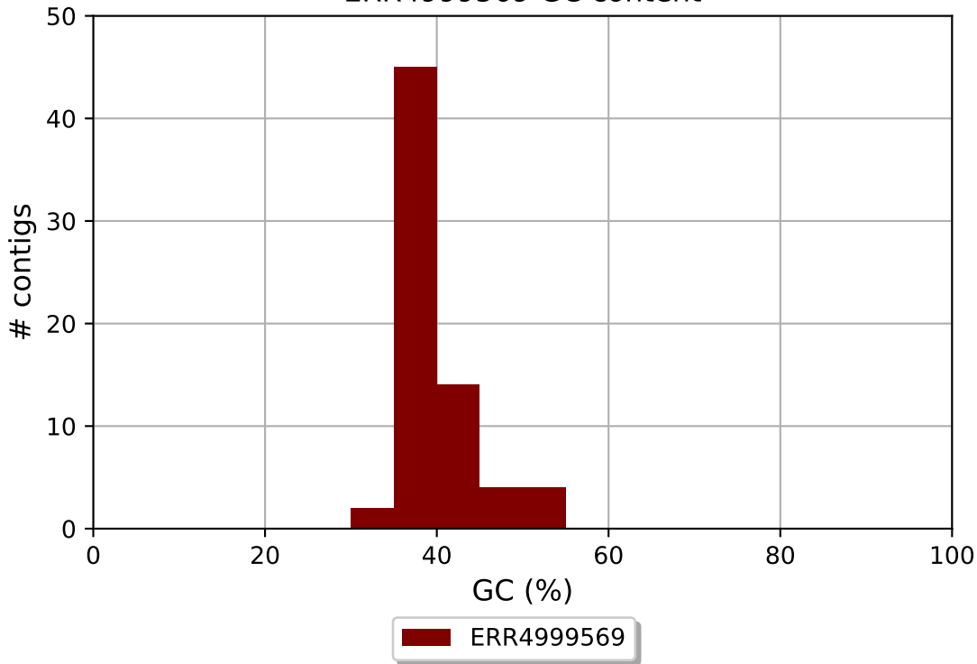
ERR4999569 GC content
