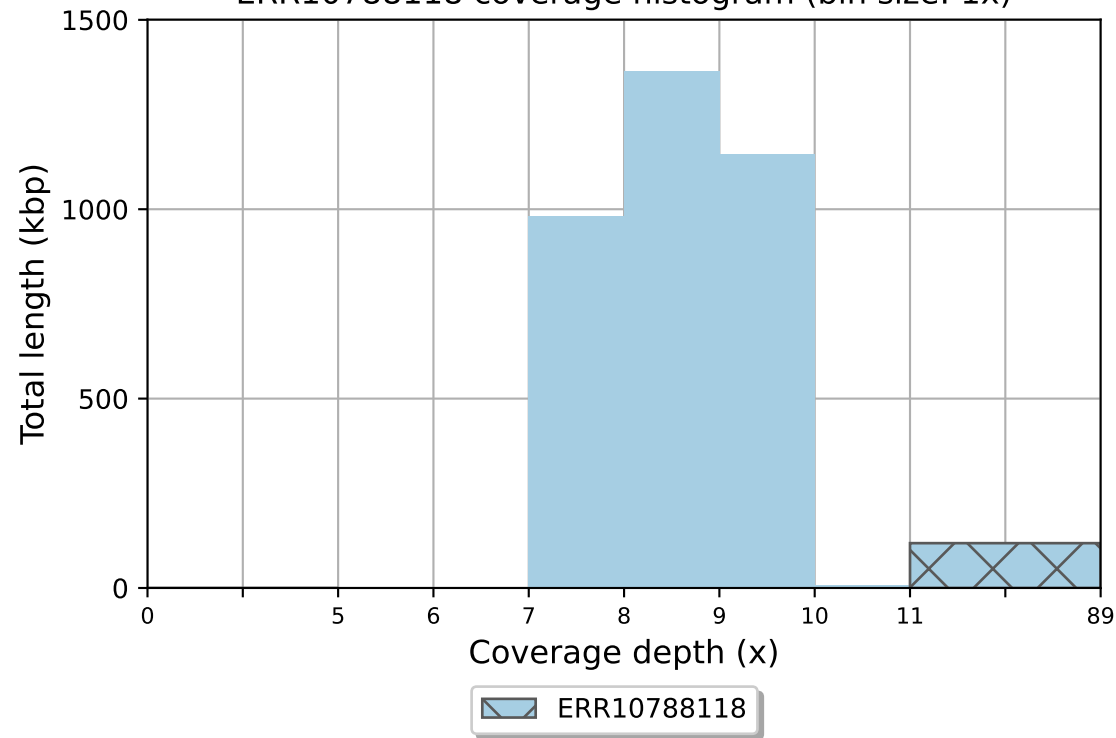
ERR10788118 coverage histogram (bin size: 1x)
