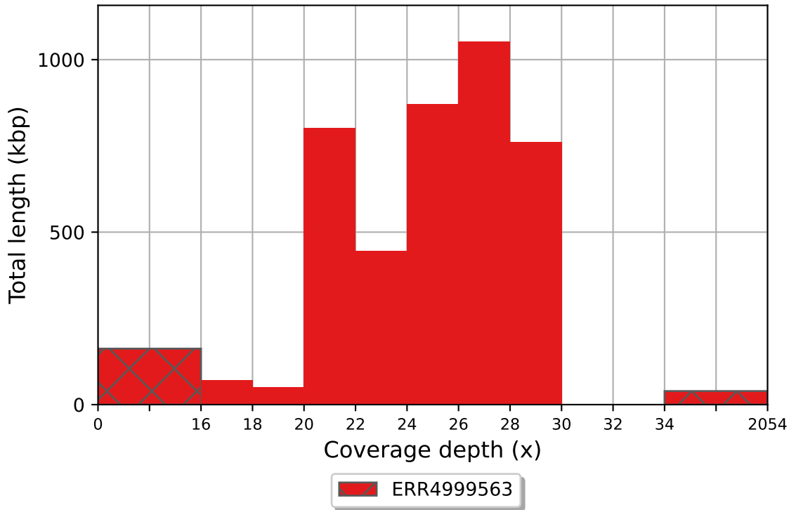
ERR4999563 coverage histogram (bin size: 2x)
