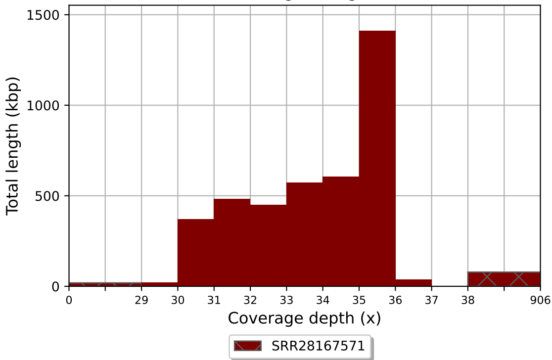
SRR28167571 coverage histogram (bin size: 1x)
