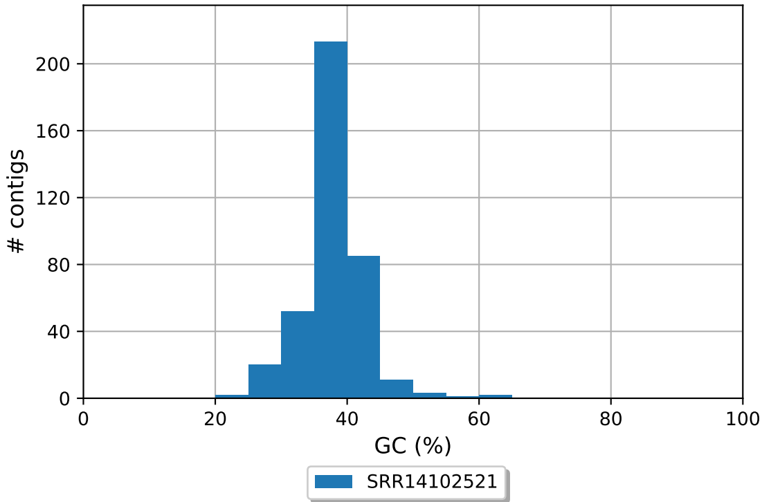
SRR14102521 GC content
