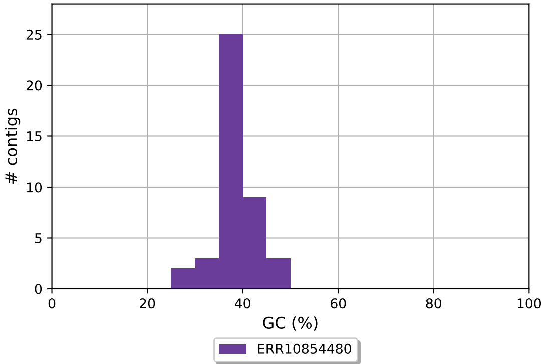
ERR10854480 GC content
