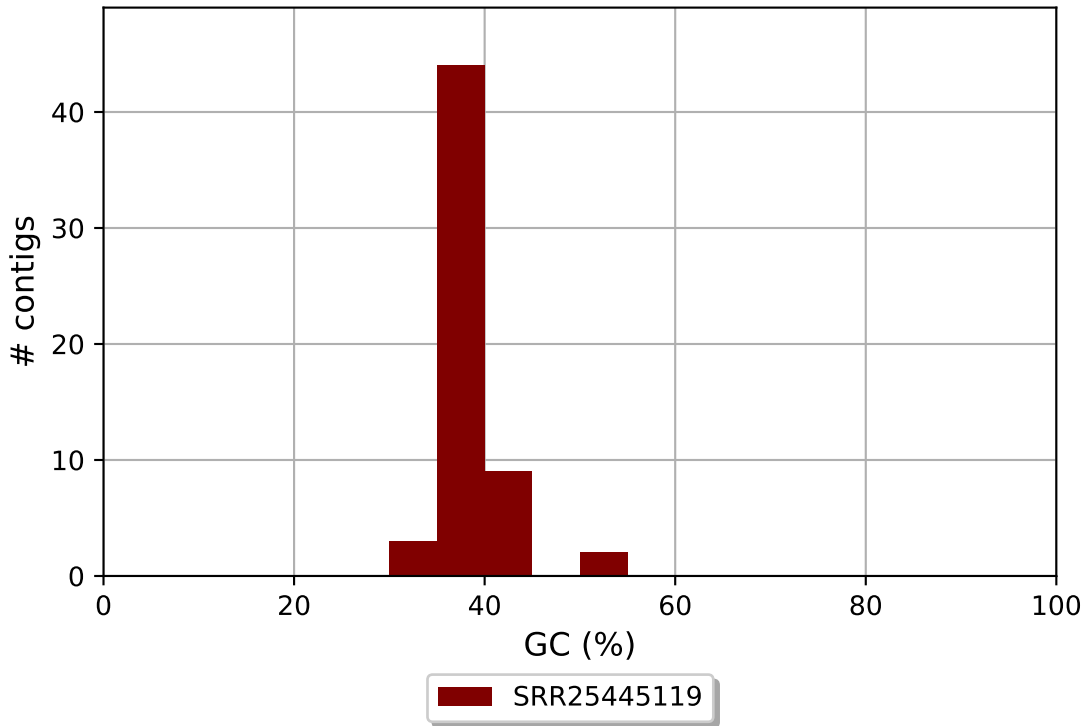
SRR25445119 GC content
