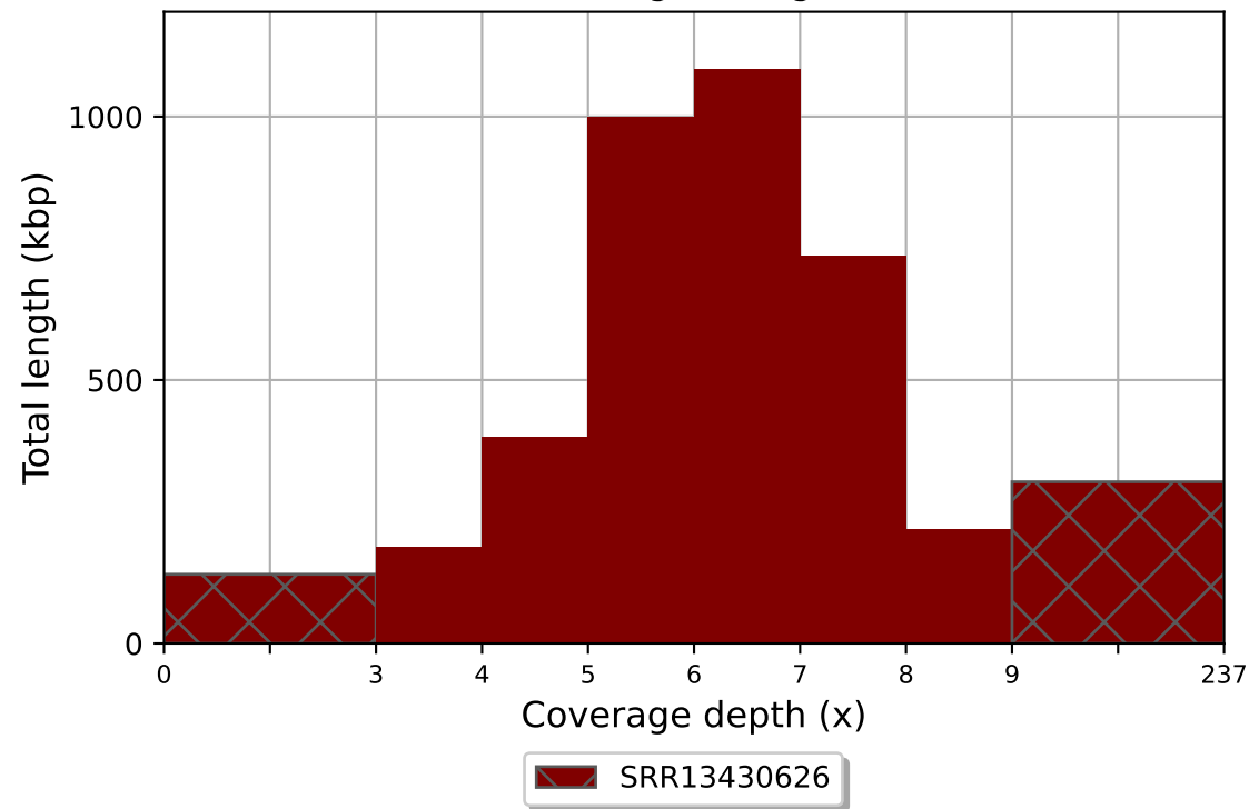
SRR13430626 coverage histogram (bin size: 1x)
