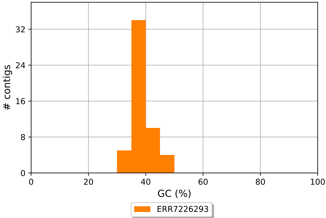
ERR7226293 GC content
