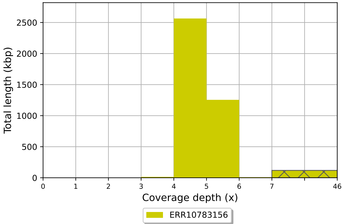
ERR10783156 coverage histogram (bin size: 1x)
