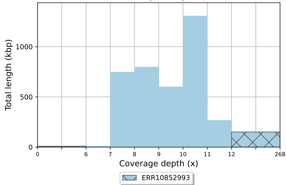
ERR10852993 coverage histogram (bin size: 1x)
