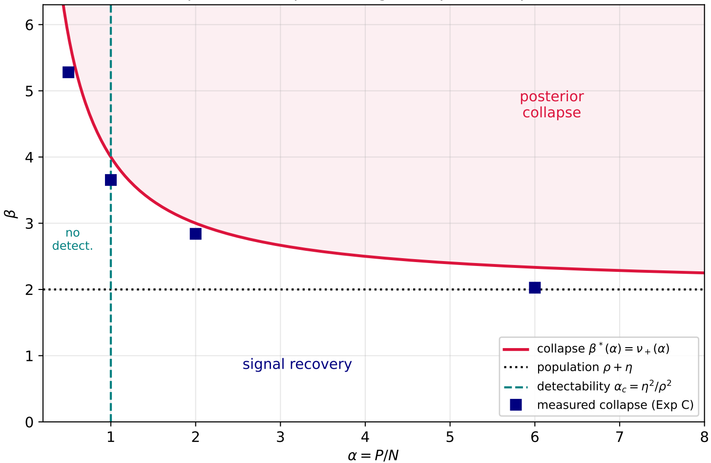
Experiment E: phase diagram ( \rho = 1.0 , \eta = 1.0 )
