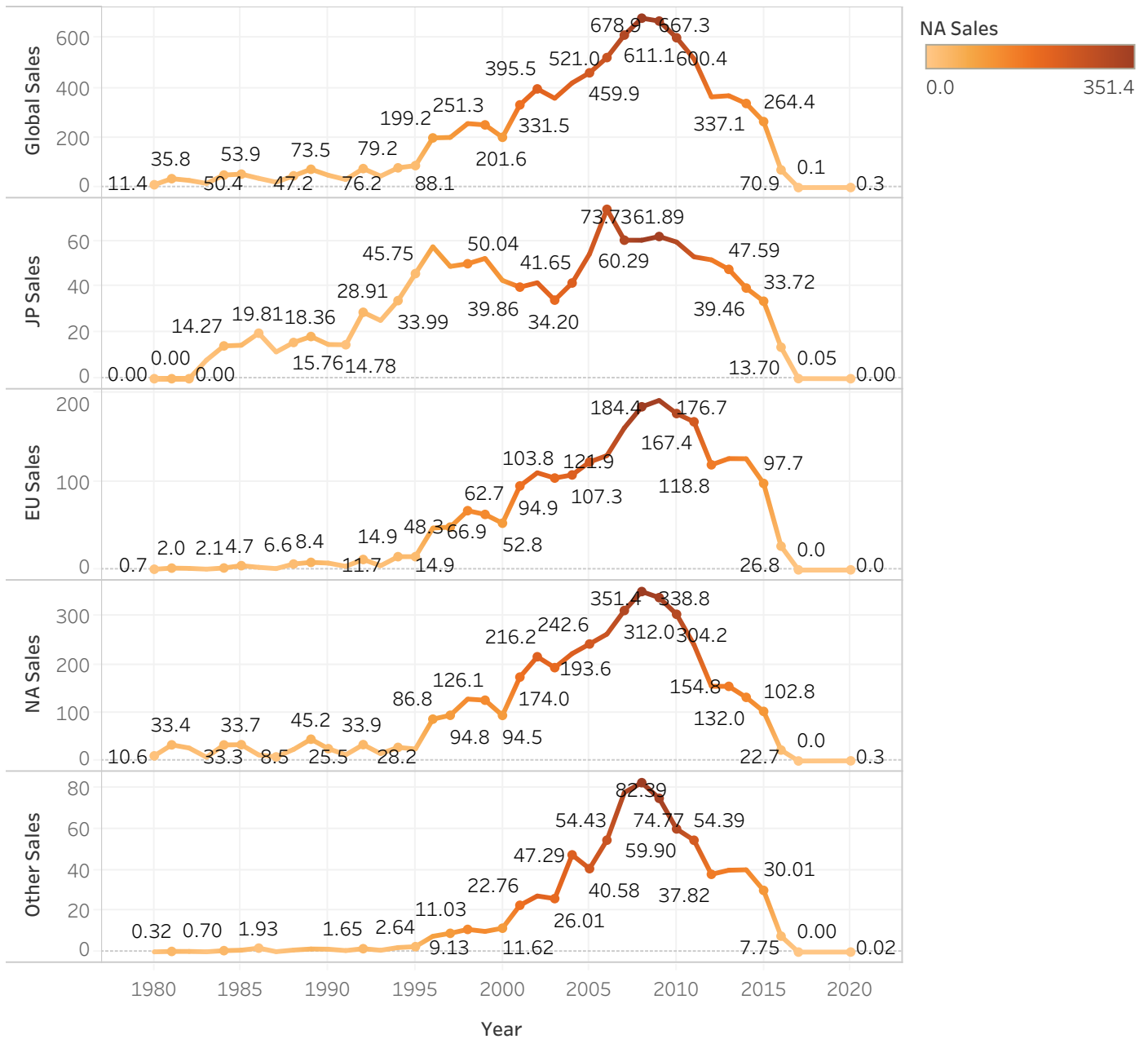
Line Chart for all the sales
