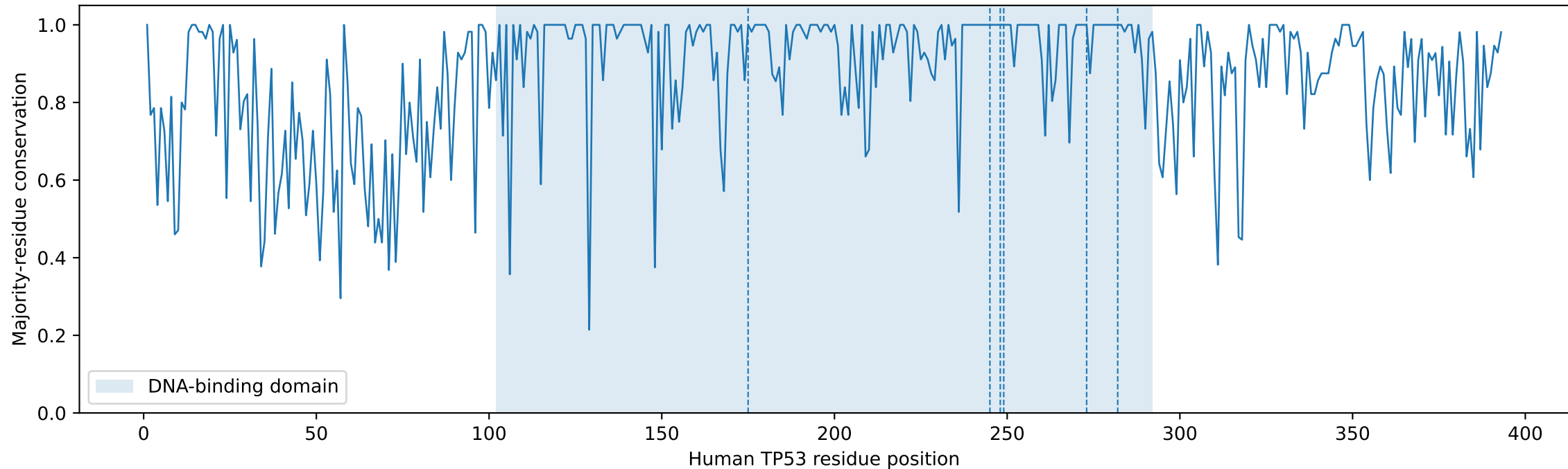
Residue-level conservation profile of mammalian TP53
