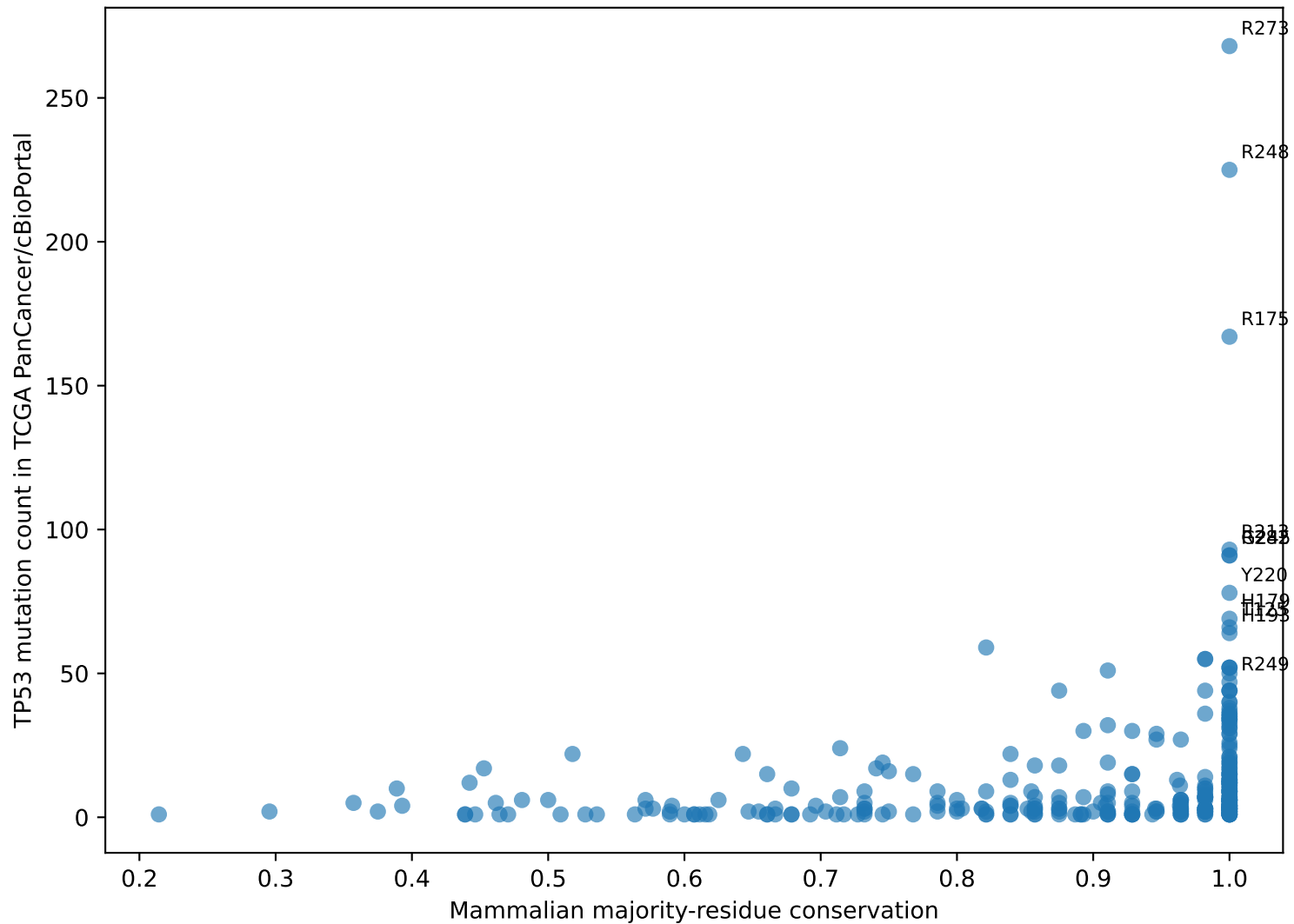
Human TP53 mutation recurrence versus mammalian conservation
