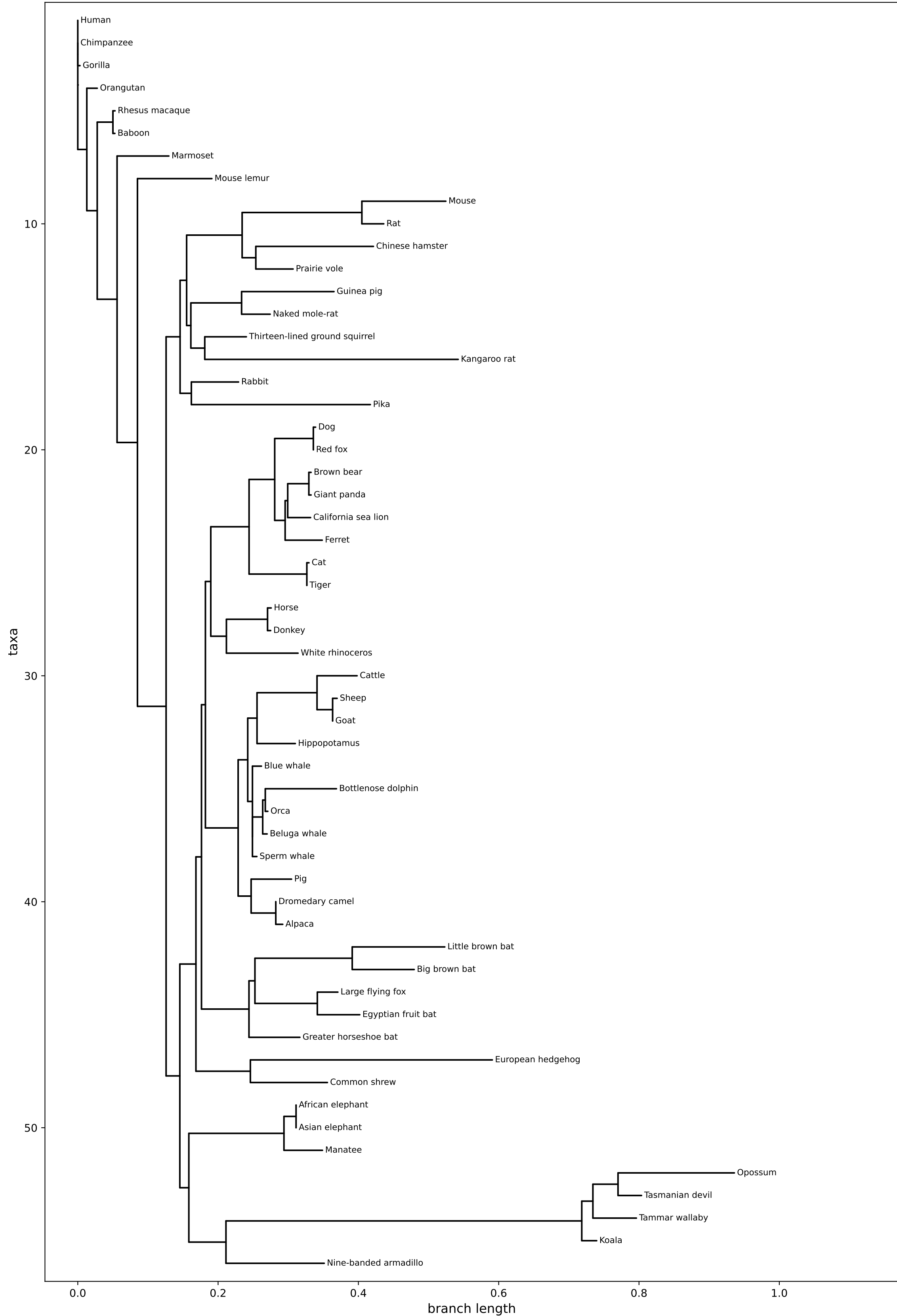
Maximum-likelihood phylogeny of mammalian TP53 protein sequences
