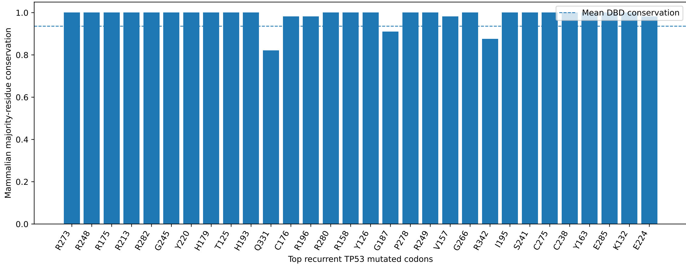
Conservation of the top 30 recurrent TP53 mutated codons
