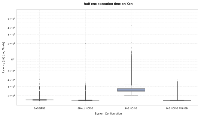
Fig. 35. TACLe benchmark - huff_enc execution time on Xen
