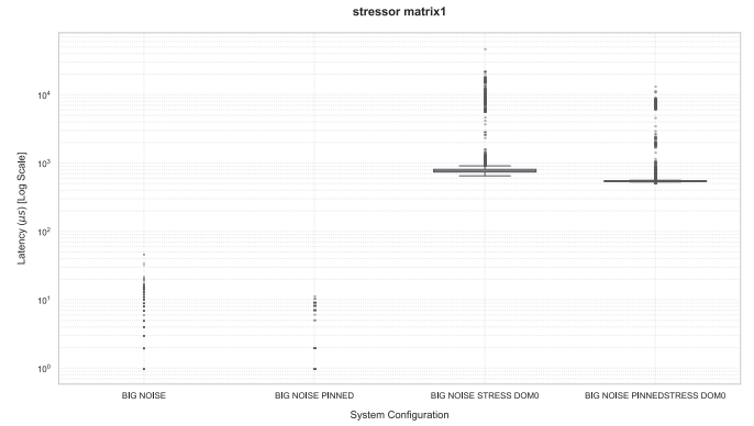
Fig. 41. TACLe benchmark - matrix1 stress dom0
