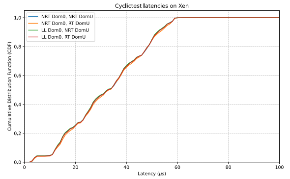
Fig. 12. Baseline Performance - Credit2 Scheduler (No Noise)
