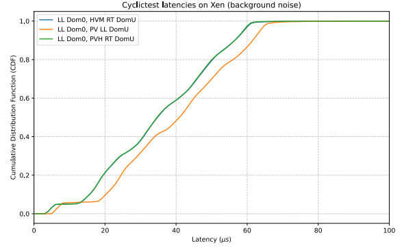
Fig. 47. Comparing HVM, PV and PVH guests - Credit2 Scheduler (Background Noise)
