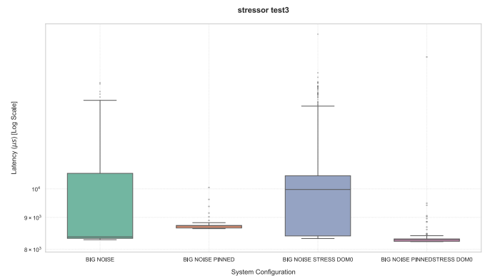
Fig. 42. TACLe benchmark - test3 stress dom0
