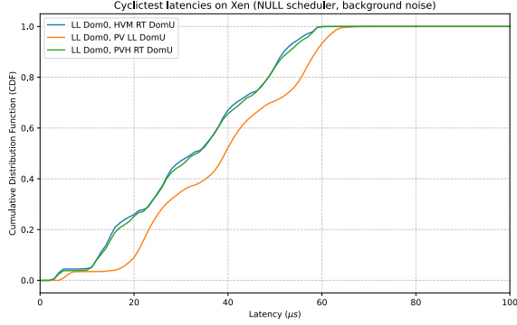
Fig. 51. Comparing HVM, PV and PVH guests - Null Scheduler (Background Noise)
