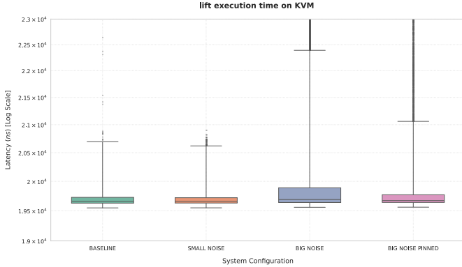
Fig. 9. TACLe benchmark - lift execution time on KVM
