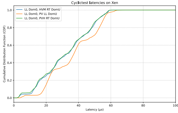
Fig. 45. Comparing HVM, PV and PVH guests - Credit2 Scheduler (No Noise)
