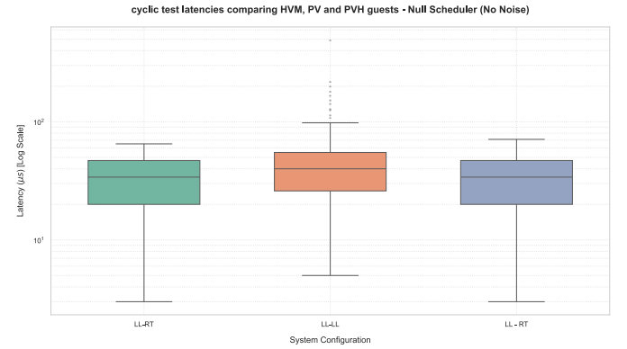
Fig. 50. Comparing HVM, PV and PVH guests - Null Scheduler (No Noise)
