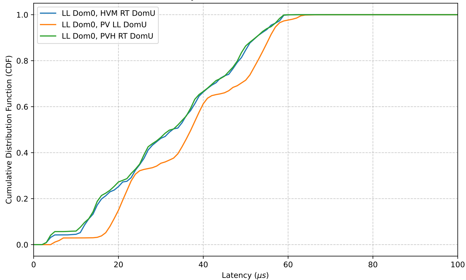
Cyclictest latencies on Xen
