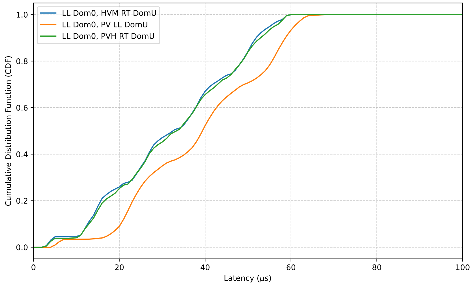
Cyclictest latencies on Xen (NULL scheduler, background noise)
