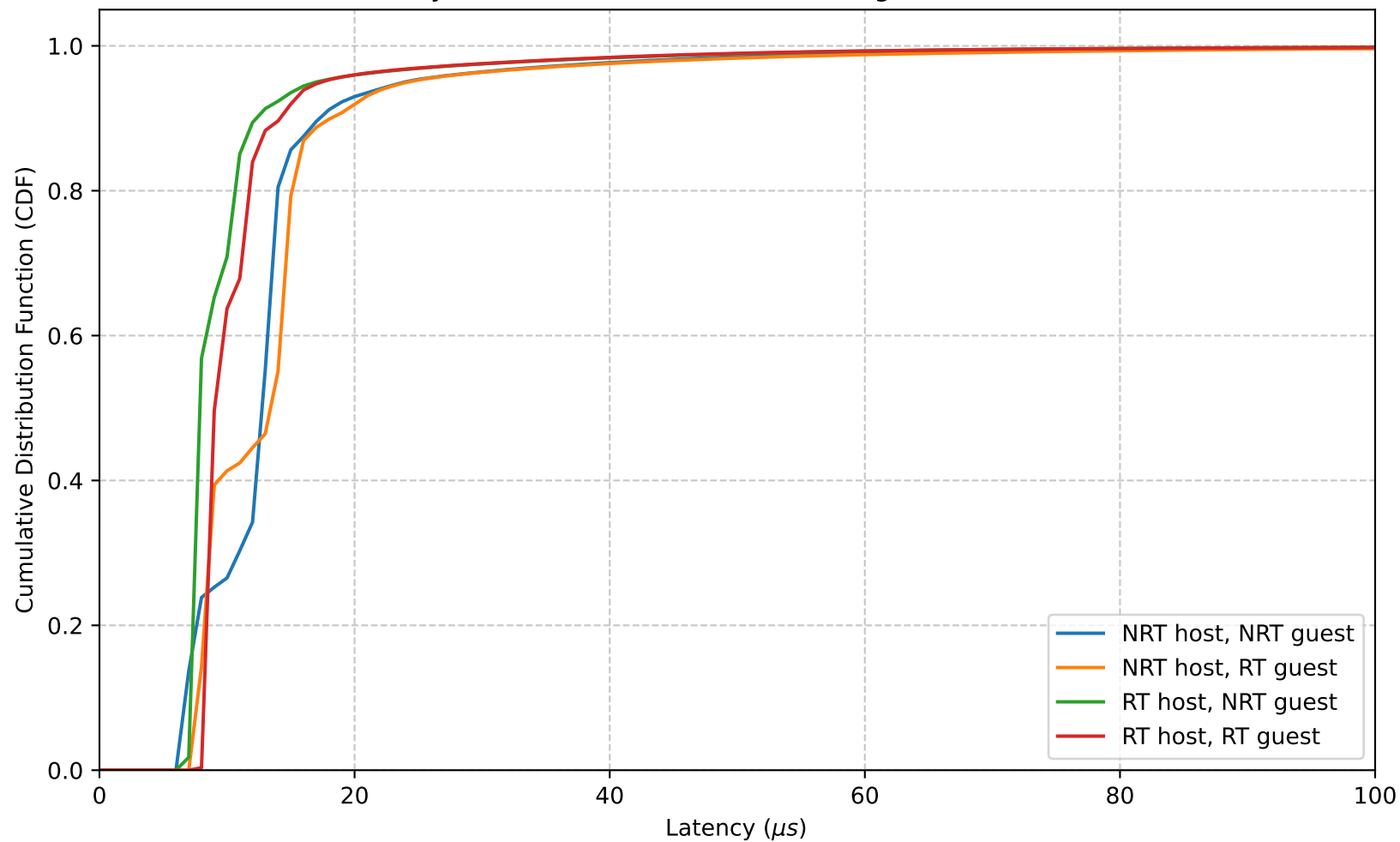
Cyclictest latencies on KVM (background noise)
