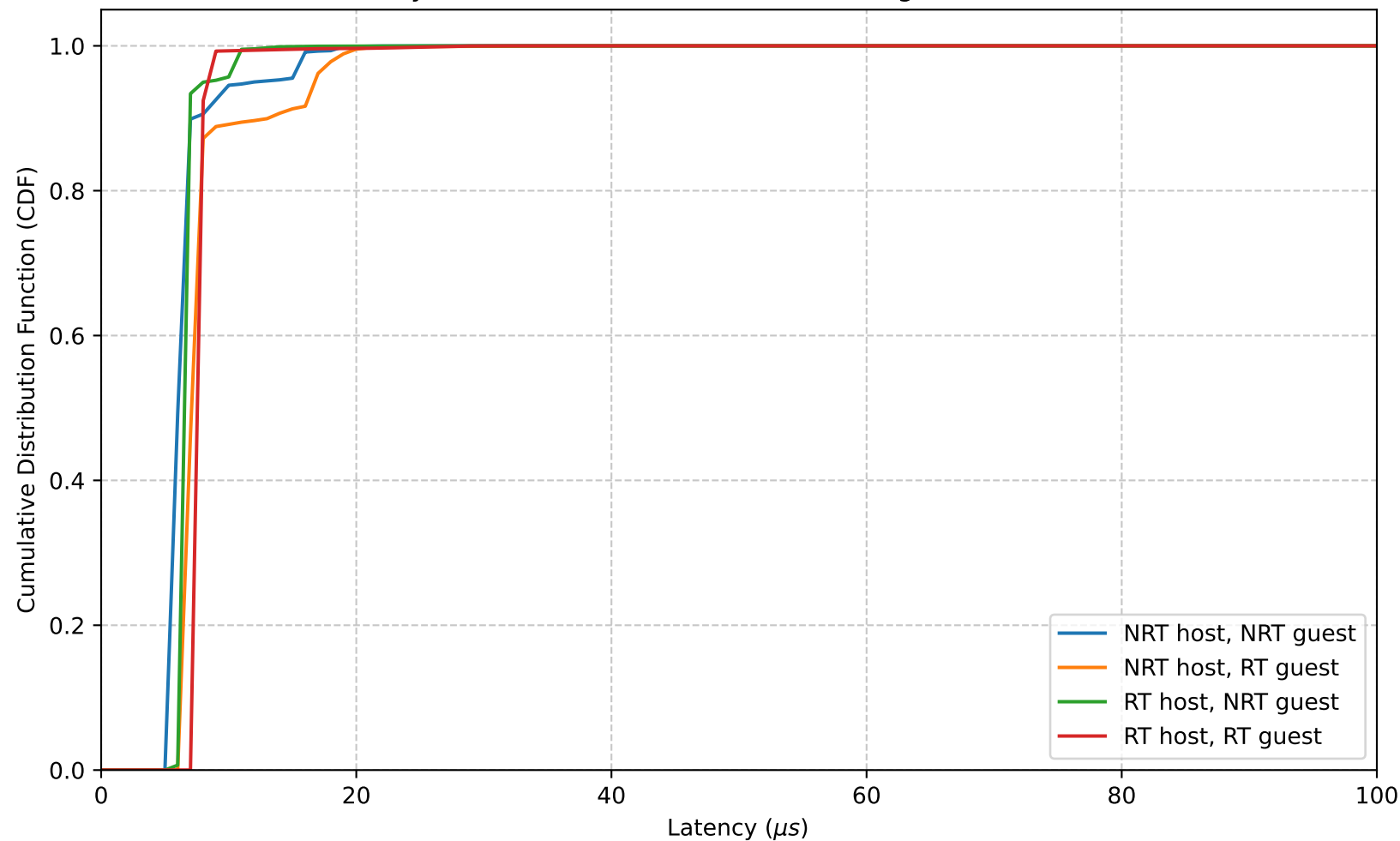
Cyclictest latencies on KVM (no background noise)
