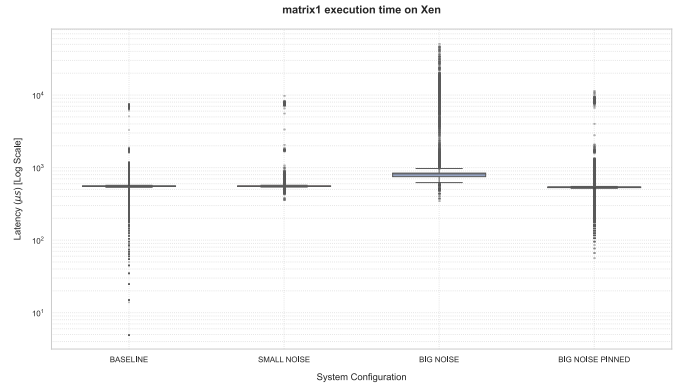
Fig. 37. TACLe benchmark - matrix1 execution time on Xen
