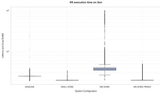
Fig. 36. TACLe benchmark - lift execution time on Xen
