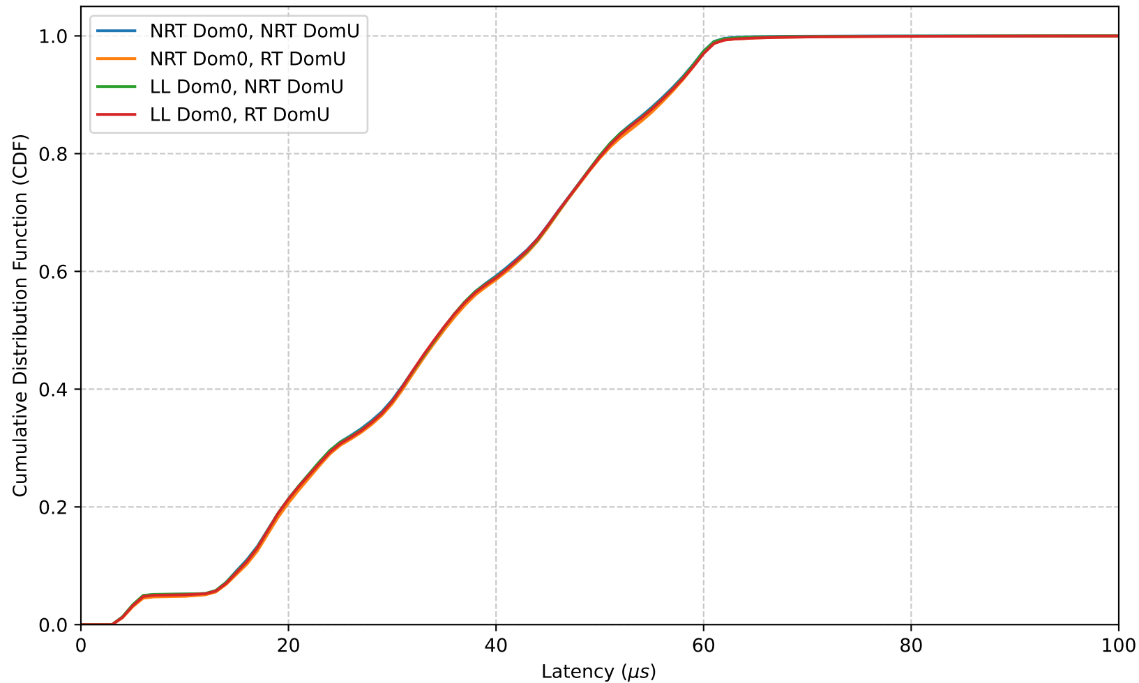
Cyclictest latencies on Xen (background noise)
