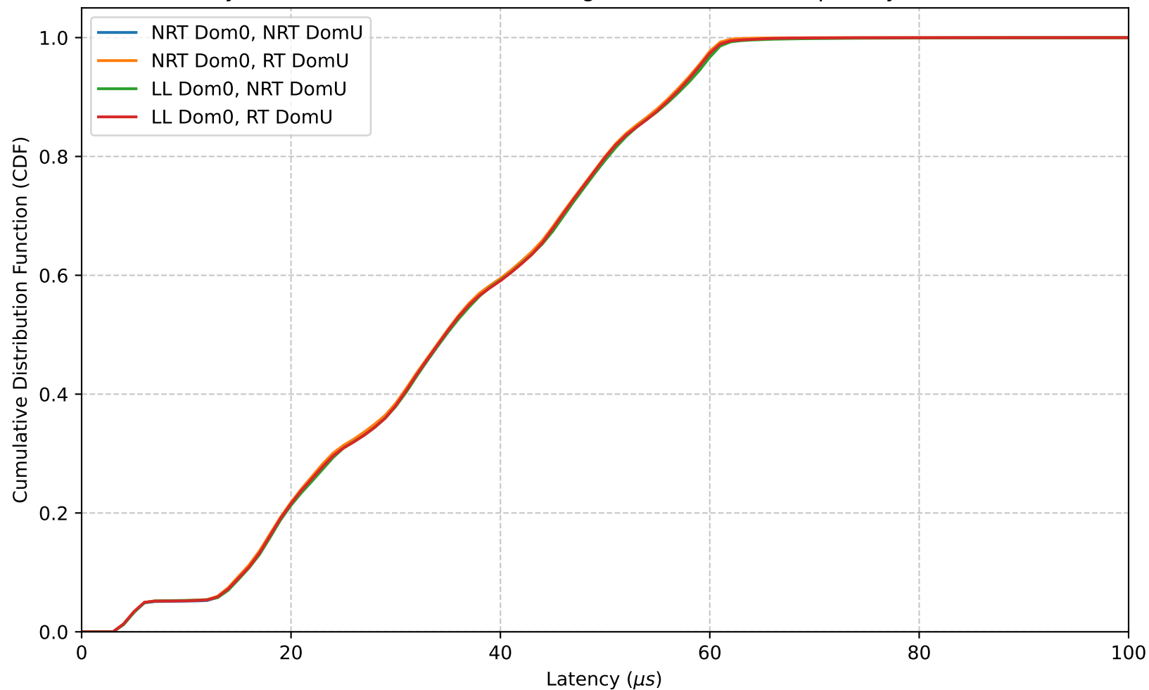
Cyclictest latencies on Xen (background noise, QEMU priority FIFO 99)
