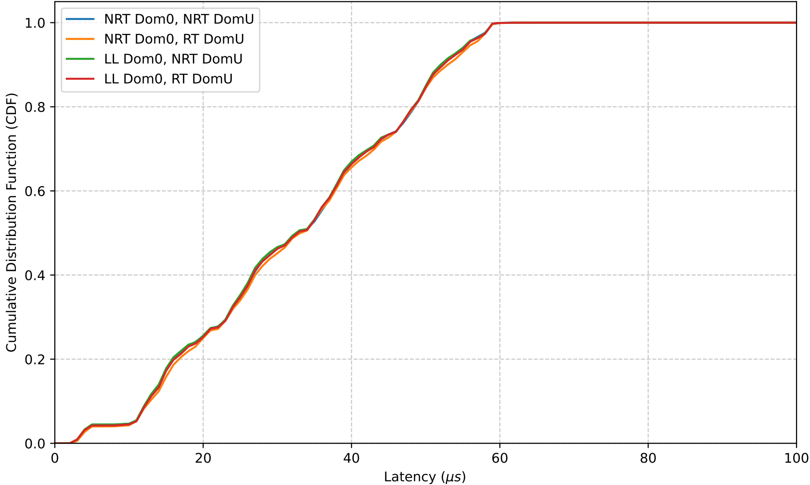
Cyclictest latencies on Xen (no background noise)
