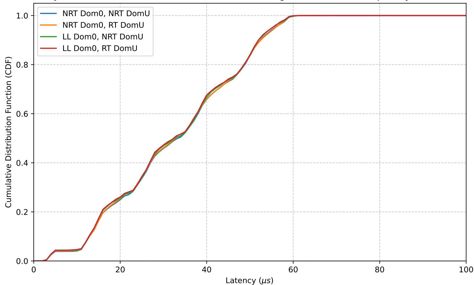
Cyclictest latencies on Xen (NULL scheduler, background noise, QEMU priority FIFO 99)
