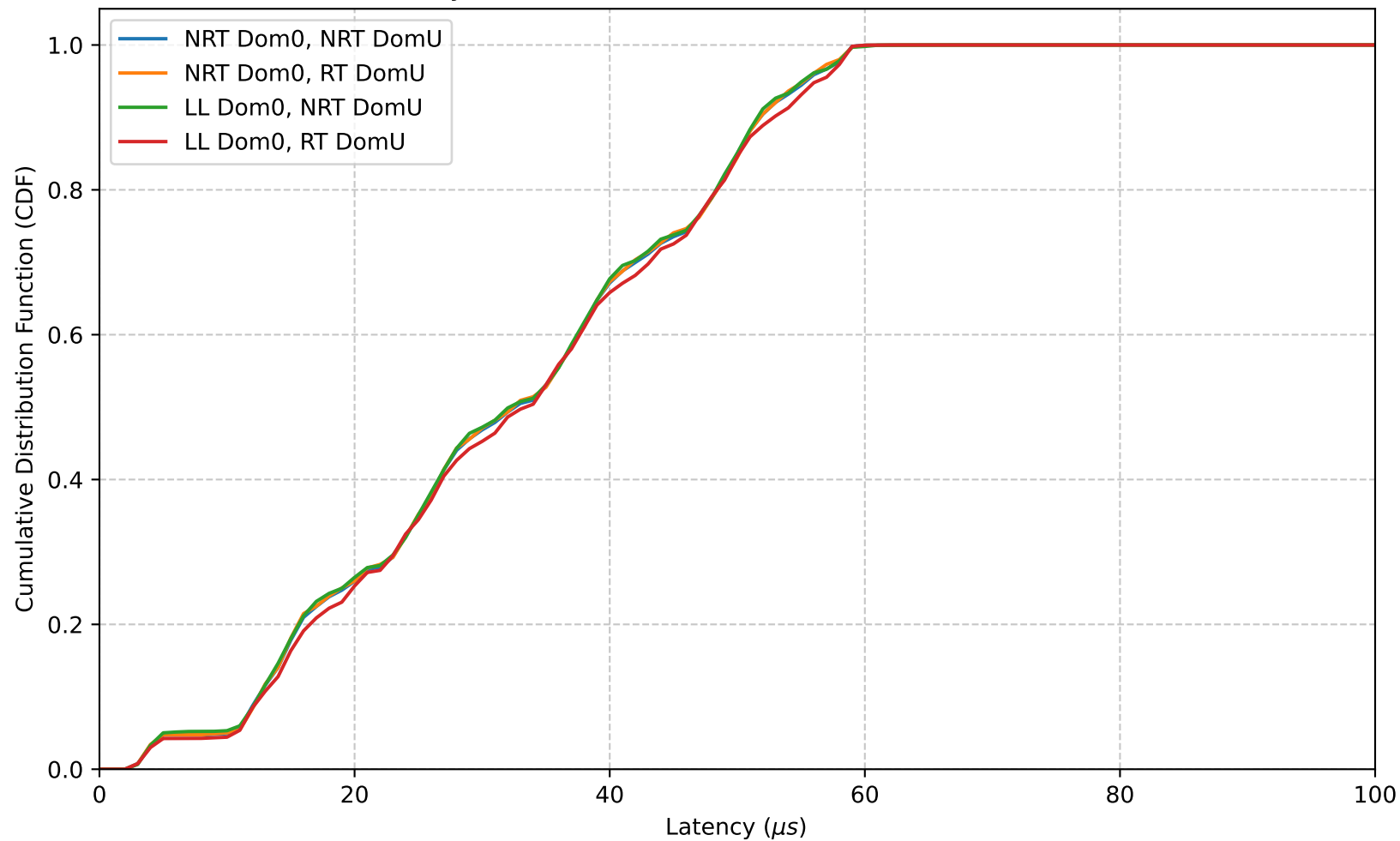
Cyclictest latencies on Xen (NULL scheduler)
