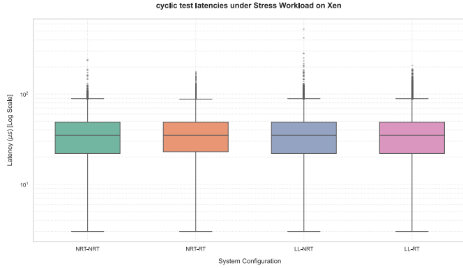
Fig. 15. Performance under Stress Workload - Credit2 Scheduler
