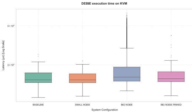
Fig. 7. TACLe benchmark - debie execution time on KVM
