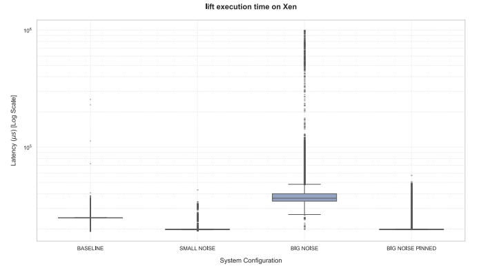
Fig. 36. TACLe benchmark - lift execution time on Xen
