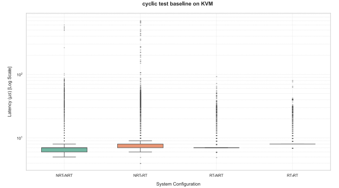
Fig. 2. Baseline Performance - KVM
