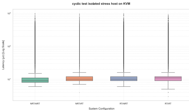
Fig. 6. Performance under stress- KVM OS-level isolation
