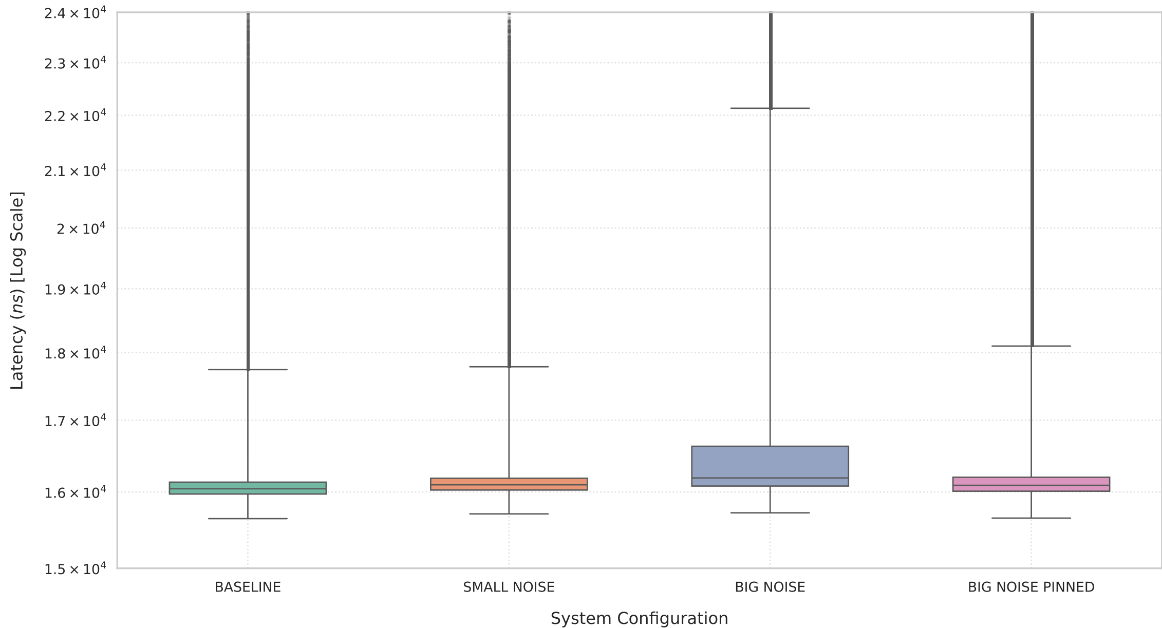
huff_enc execution time on KVM
