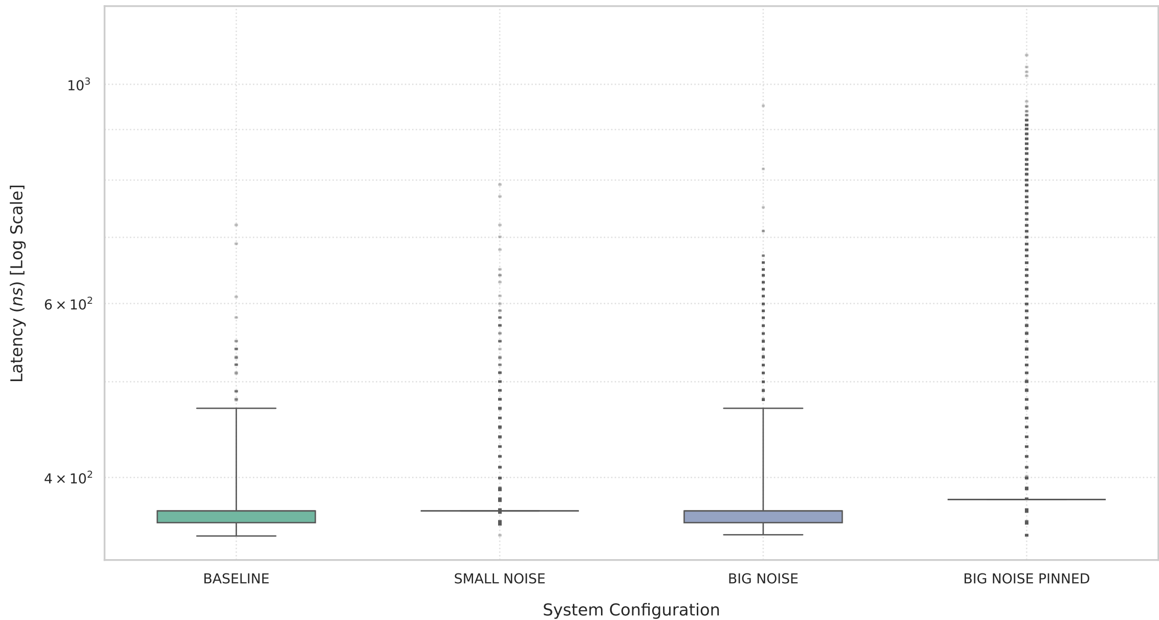
matrix1 execution time on KVM
