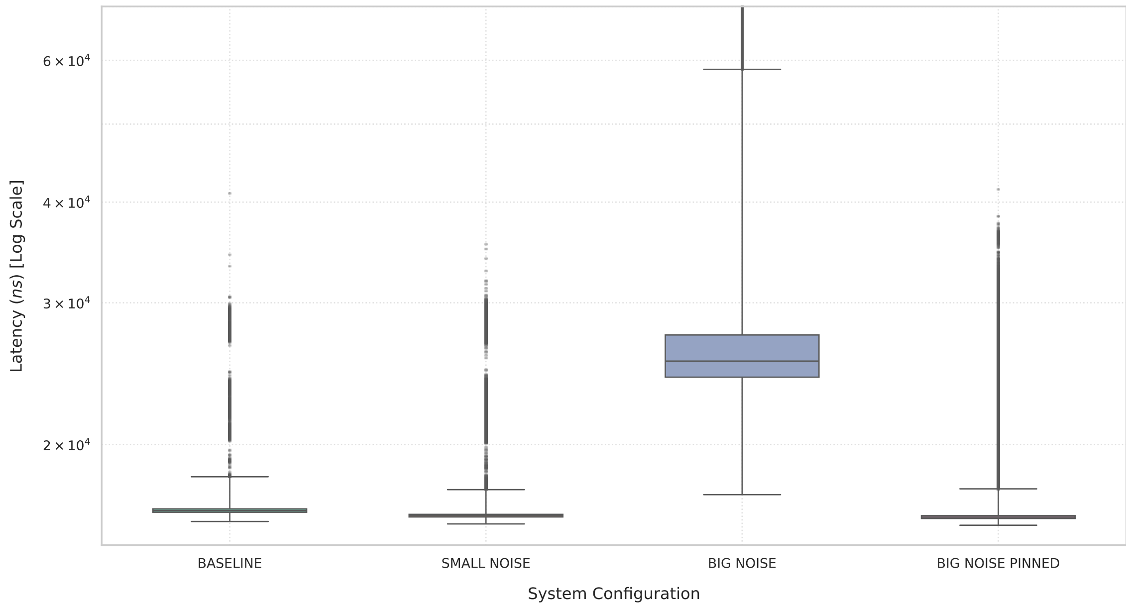
huff_enc execution time on KVM
