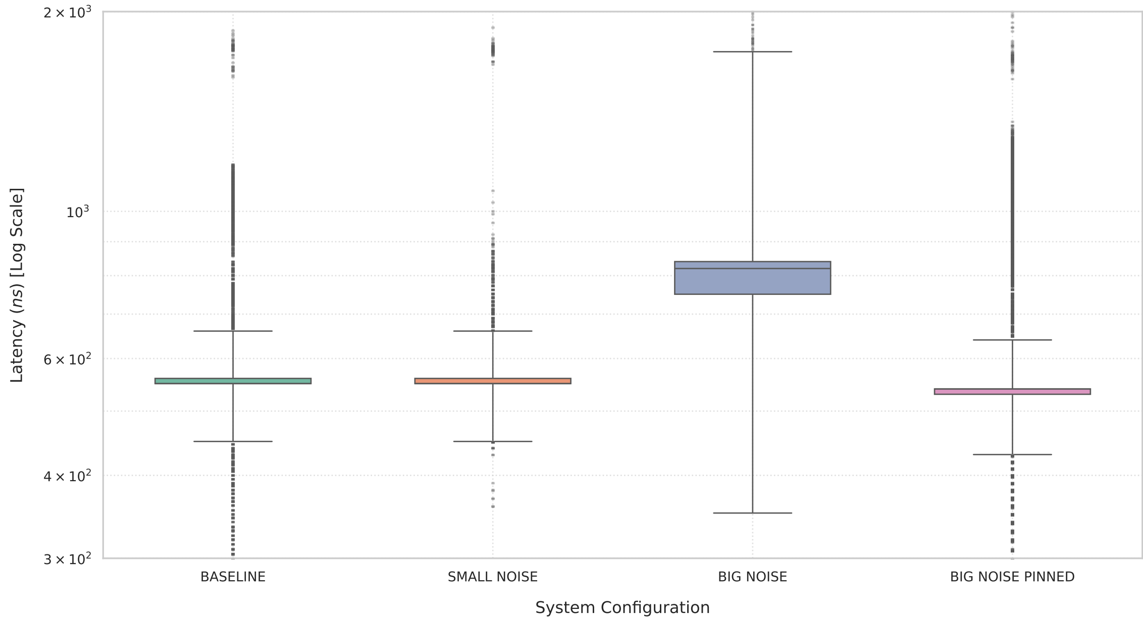
matrix1 execution time on KVM
