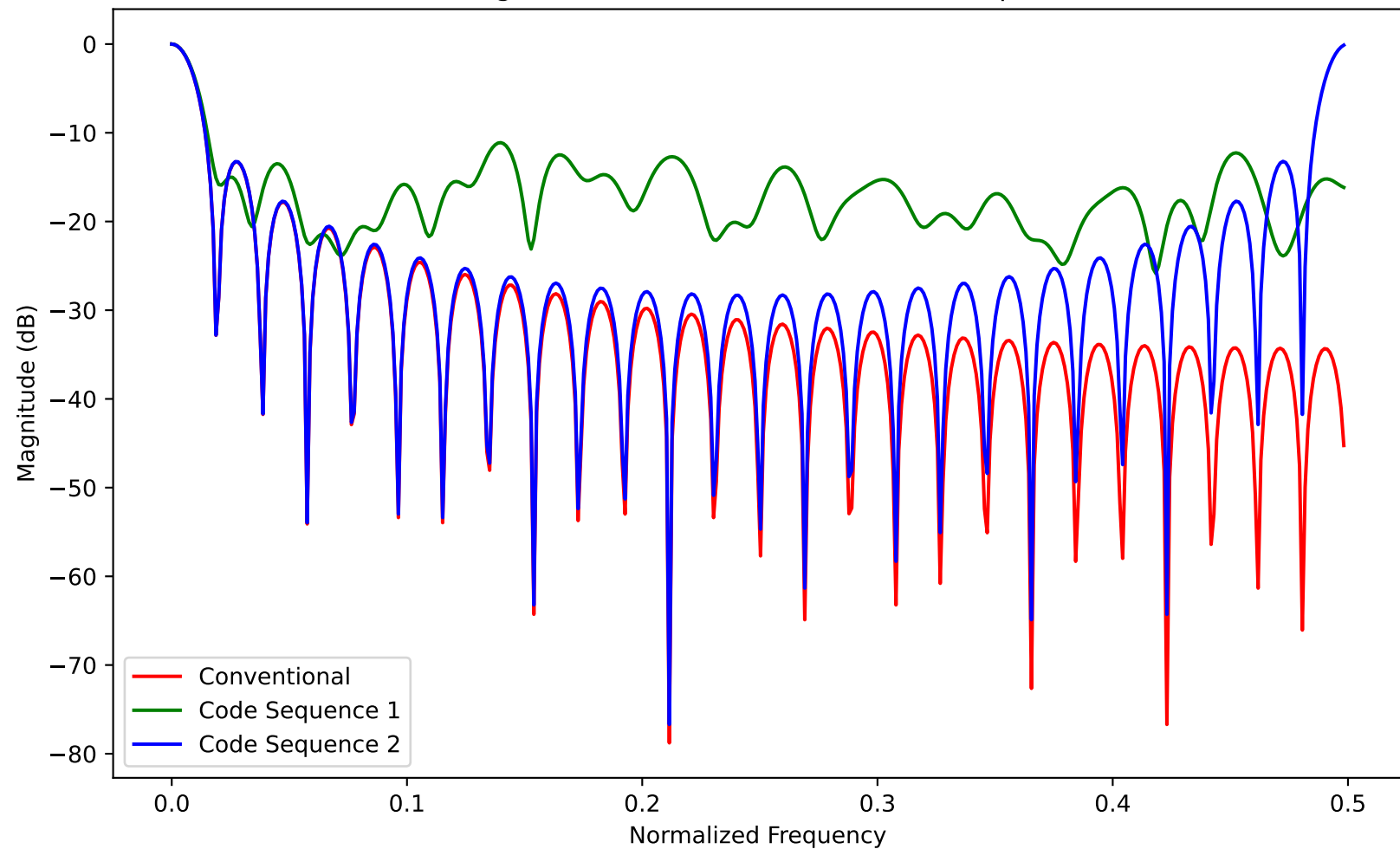
DFT Magnitude of Blur Kernels (Positive Frequencies)
