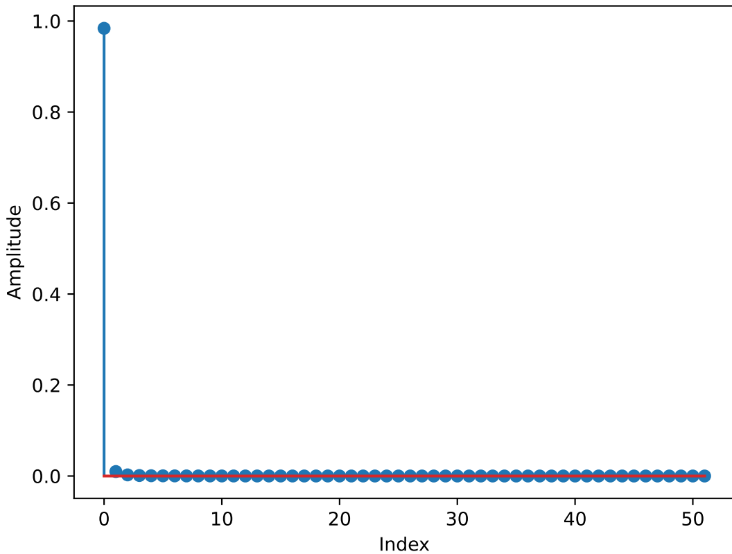
PSF: 1/x^2 normalized
