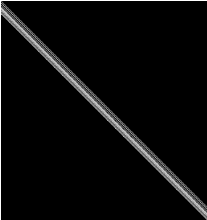
Toeplitz Matrix (Code Sequence 1)
