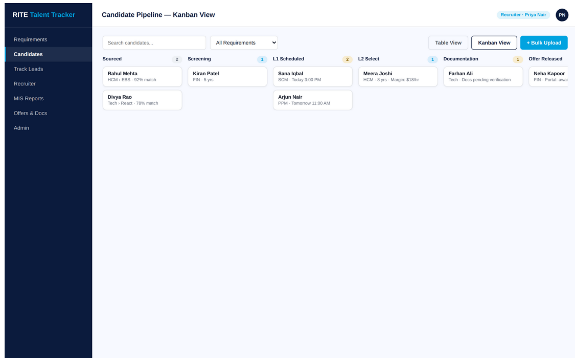
Figure 3.4 — Candidate Kanban board (src/components/PipelineKanban.jsx)
