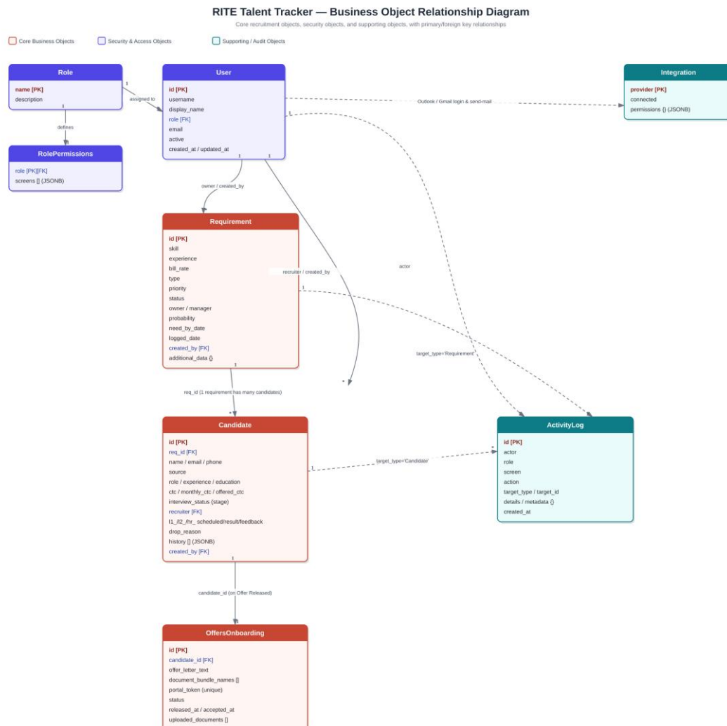
Figure 4.4 — Core, security and supporting business objects and their relationships
