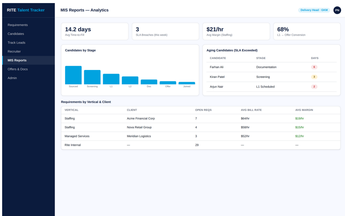
Figure 3.6 — MIS Reports (src/components/MISReports.jsx)
