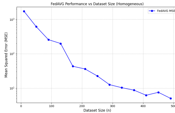
Figure 1: Test MSE for FedAvg on homogeneous data versus dataset size. We see that more training data leads to higher accuracy.
