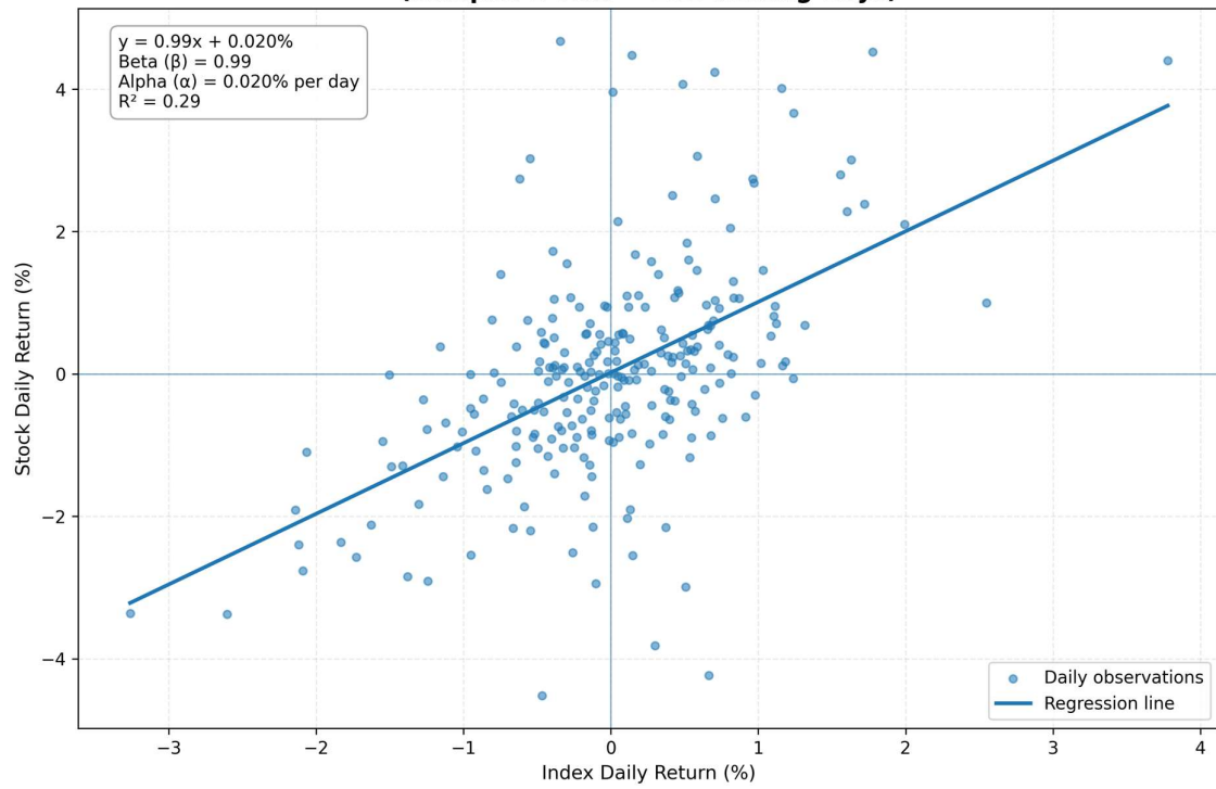
Asian Paints vs NIFTY 50 - Daily Returns Regression (Sample: 1 Year \approx 252 Trading Days)
