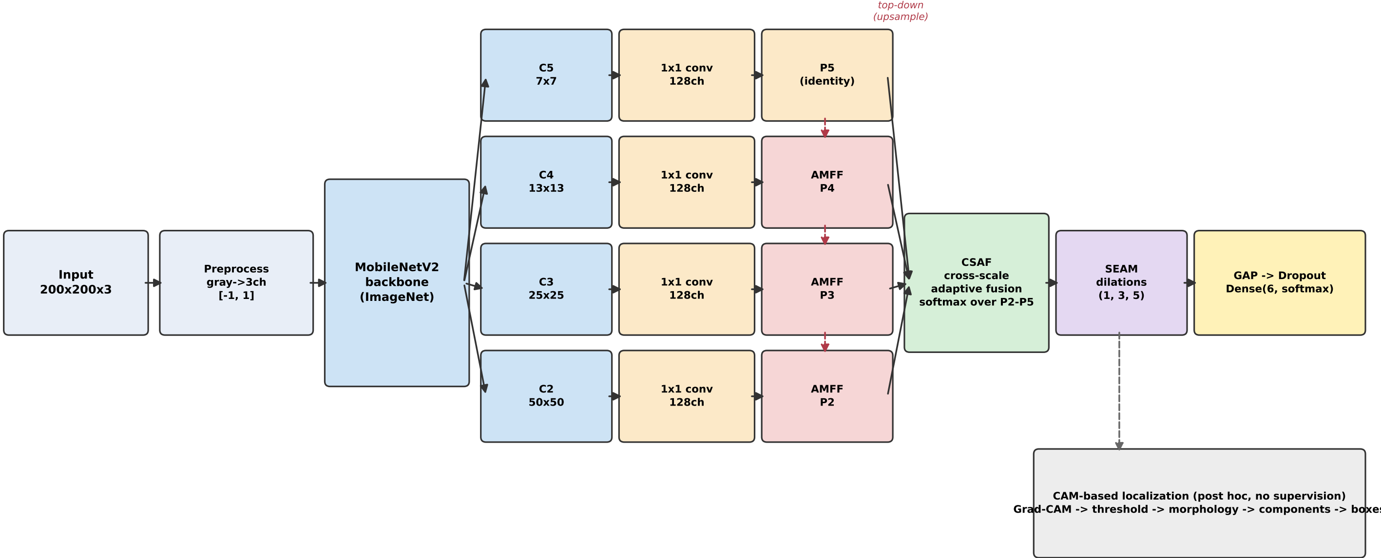
Figure 2 Proposed architecture: MobileNetV2 -> FPN(AMFF) -> CSAF -> SEAM -> classifier
