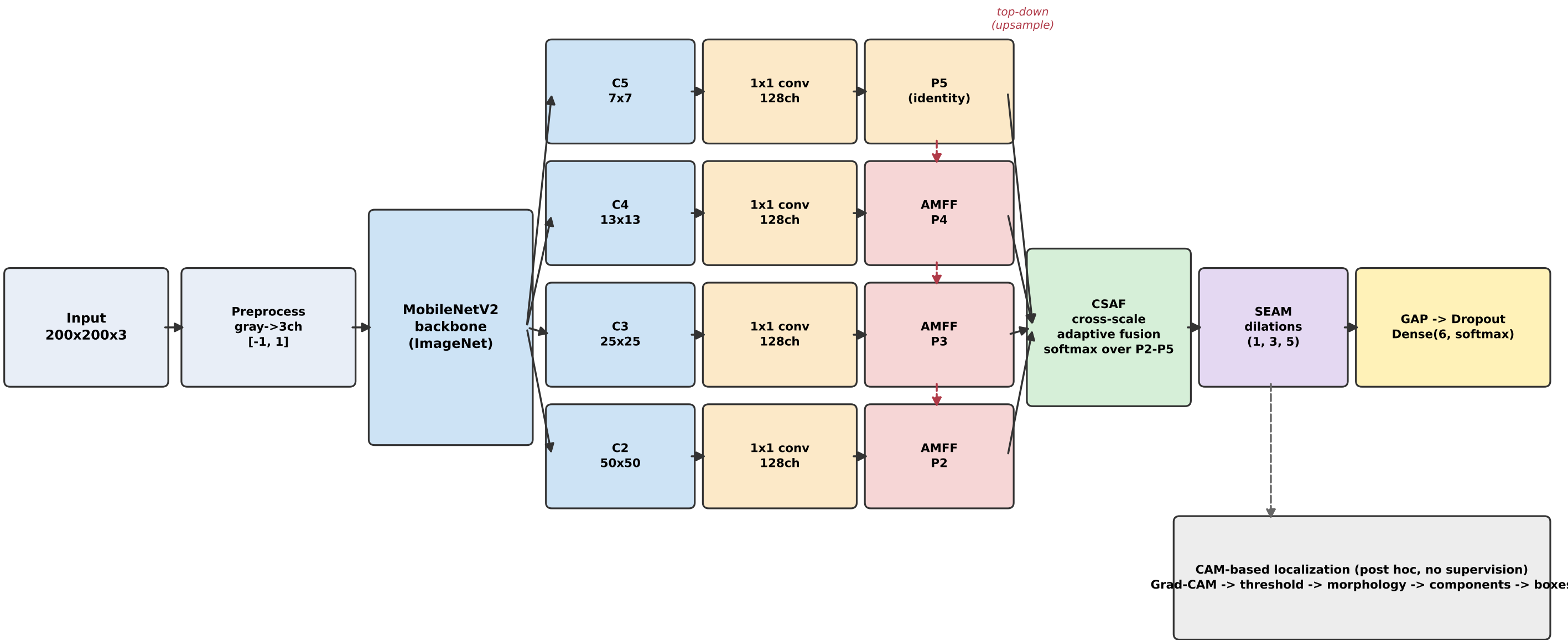
Figure 2 Proposed architecture: MobileNetV2 -> FPN(AMFF) -> CSAF -> SEAM -> classifier
