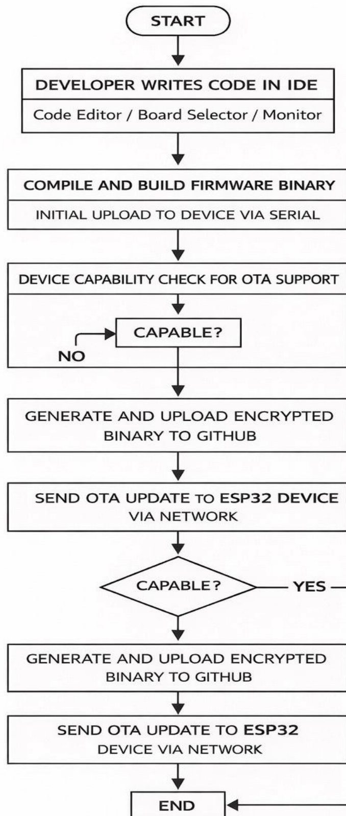
FIG. 2: Firmware Update Workflow of Secure OTA Development Framework
