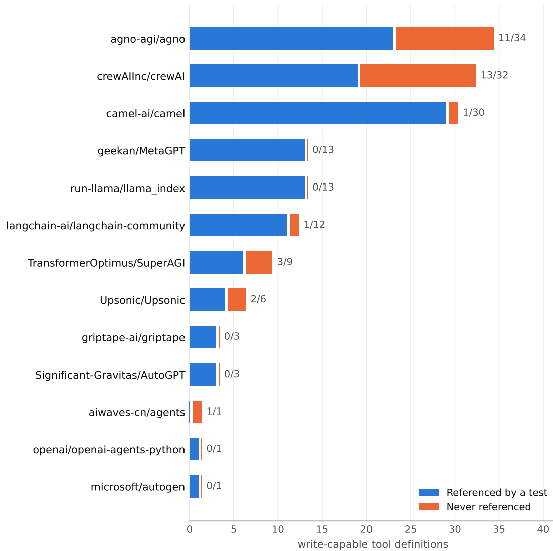
Figure 1. Write-capable tool definitions per repository, split by whether each is referenced anywhere in that repository's tests. Counts at the right are uncovered/total. Generated from part_a/results.json .
