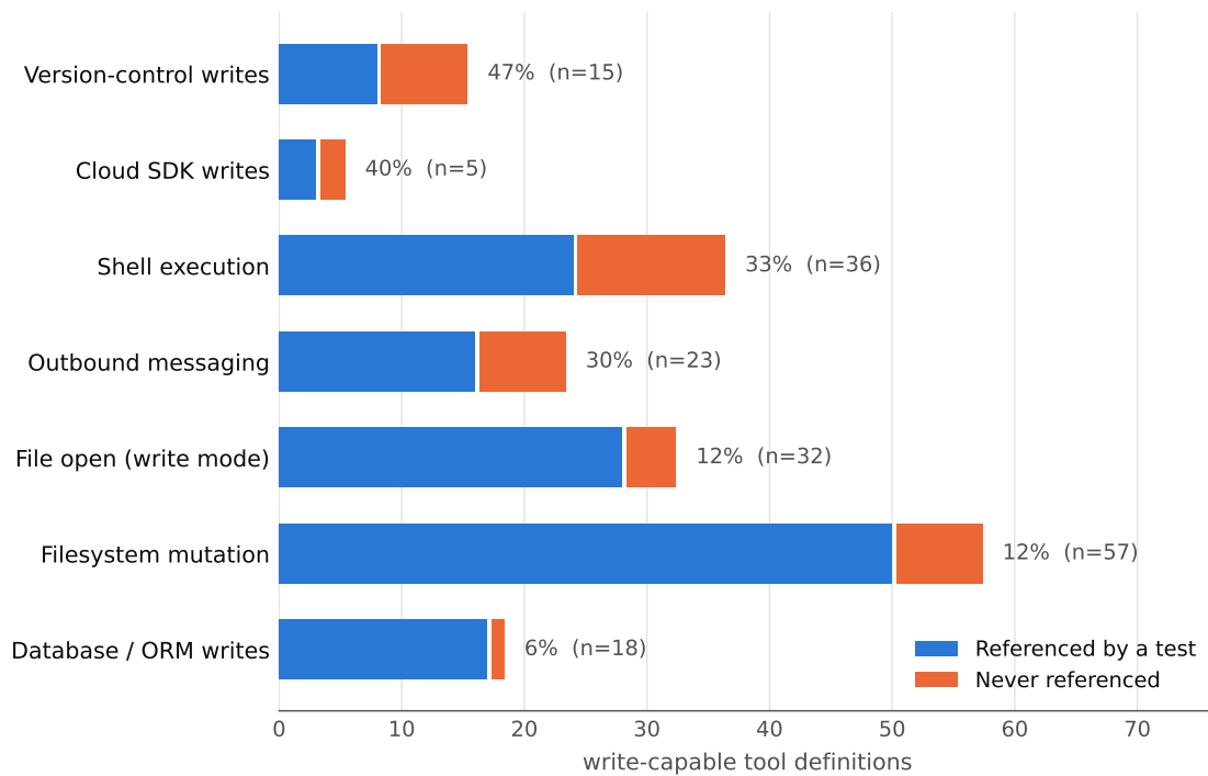
Figure 2. Test coverage by kind of write operation, for categories with at least five tools. Percentages are the share never referenced by any test.
