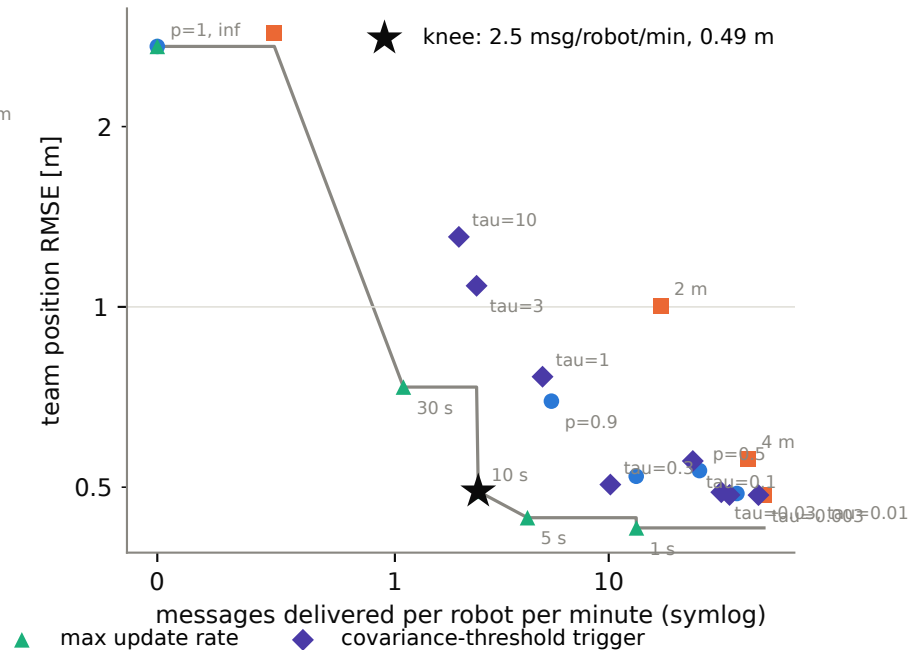
Map-blind team: only robots 1-2 observe landmarks
