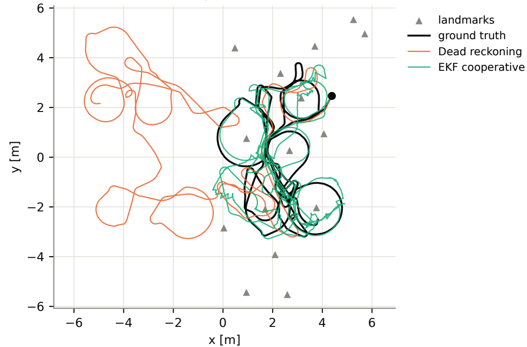
Dataset 1, robot 3: map-blind (no landmark access)
