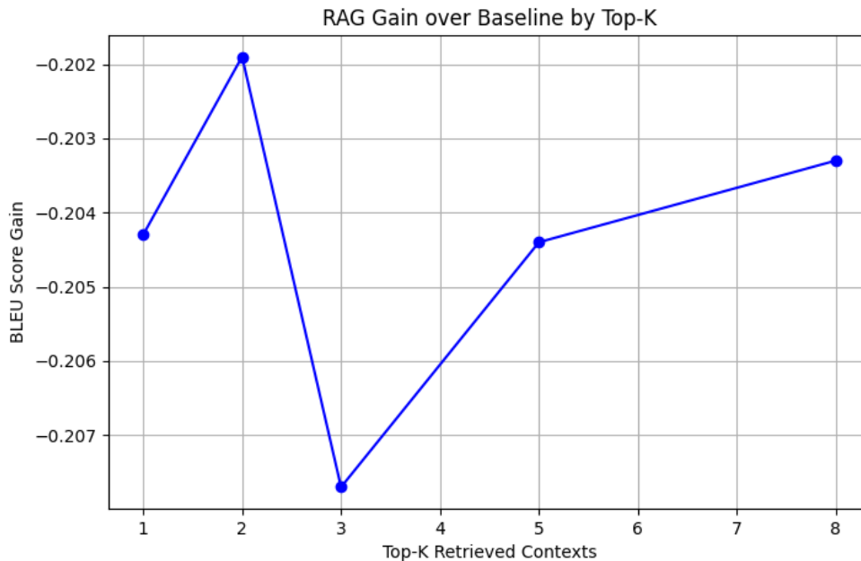
Figure 4.5 — RAG BLEU gain over the no-RAG baseline as a function of top-K (retrieved passages). Every tested depth remains negative, peaking (least negative) at K = 2 and degrading again beyond it.
