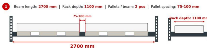
Industrial Pallet - 1200 x 1000 mm
