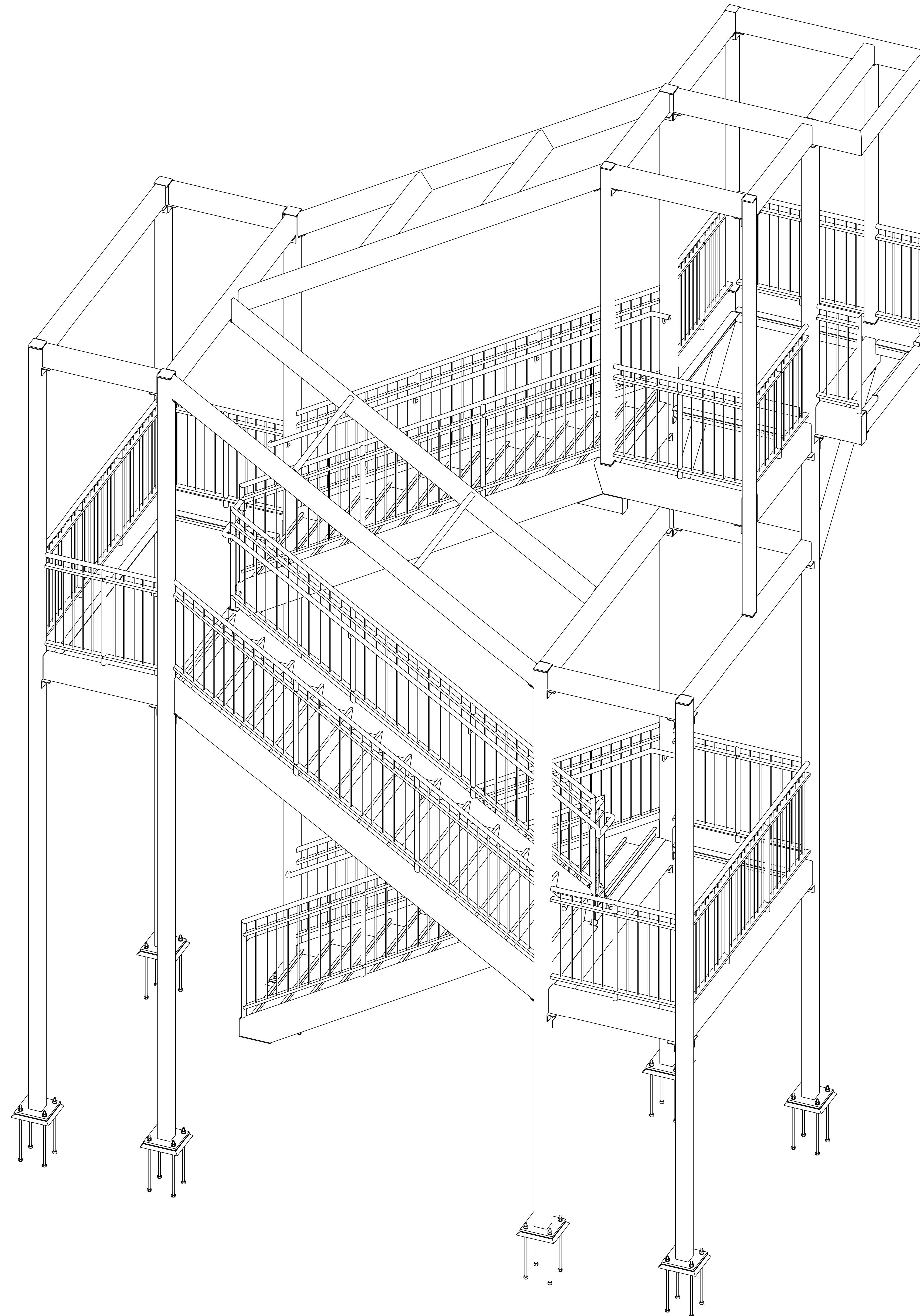
ISOMETRIC VIEW
