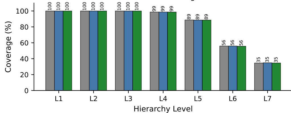
Per-Level Coverage
