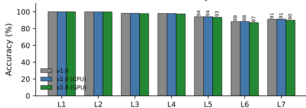
Per-Level Accuracy
