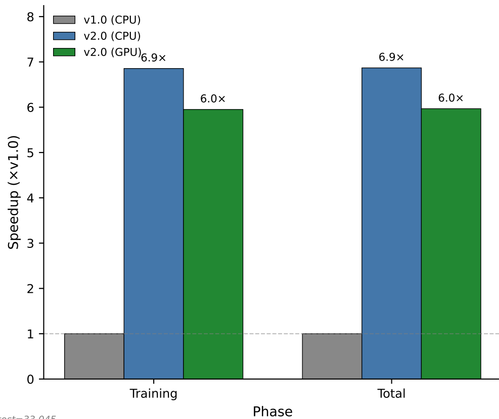
Dataset: Wang
