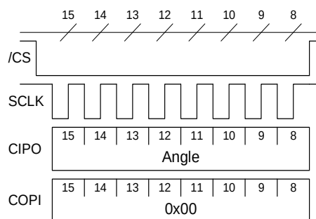
Figure 11: Diagram of a Partial 8-Bit SPI Angle Reading
