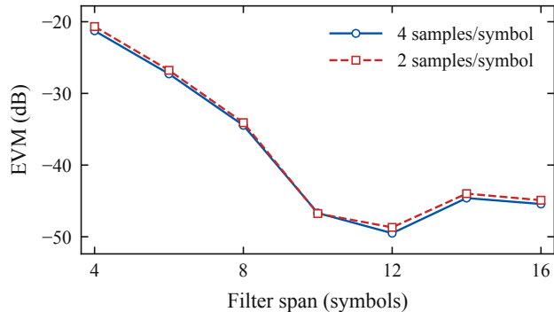
(a) Digital TX EVM
