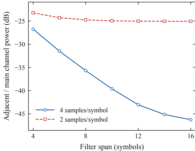
(b) Adjacent-channel leakage
