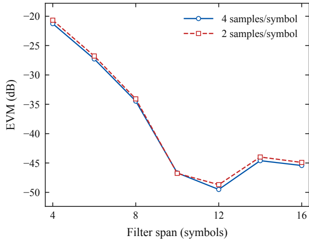
(a) Digital TX EVM
