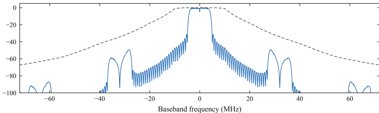
(c) 4 sps, filter tune 0
