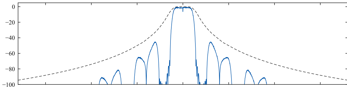
(c) 4 sps, filter tune 0
