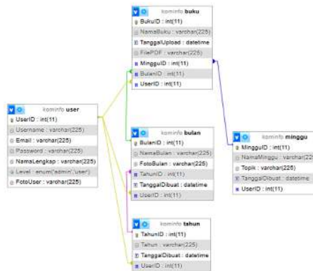
Gambar 3.10 Diagram ERD Design
