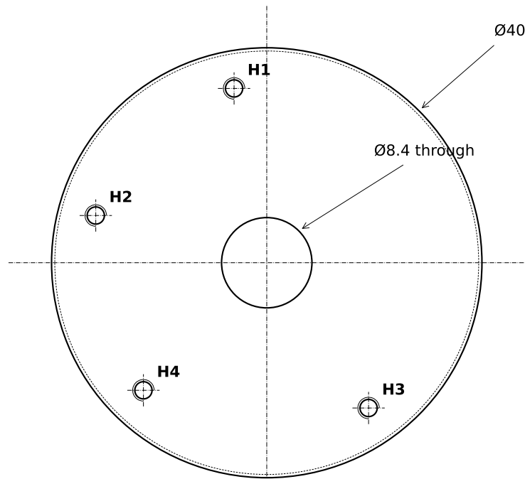
TOP VIEW (cap side, +x right, +y up) 2:1
